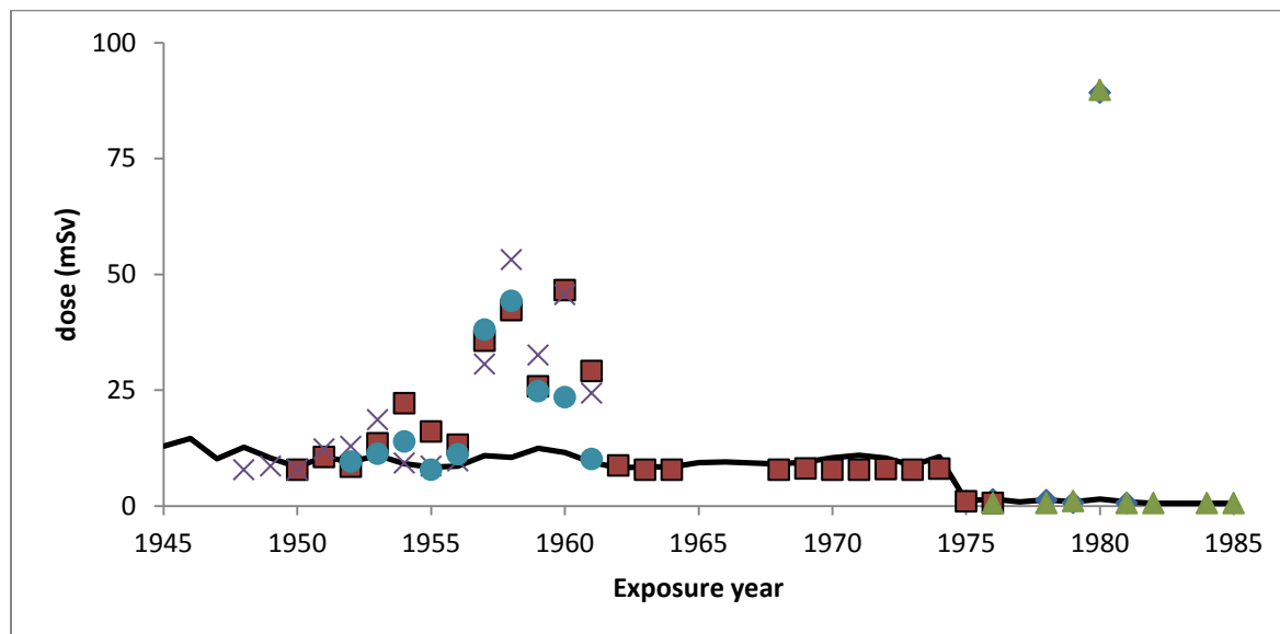
Figure 4. Annual doses for workers (n=5) with outlying cumulative doses relative to the coworker model. Solid line indicates coworker 95 th -percentile values from Table 1 of ORAUT-OTIB-0026.
