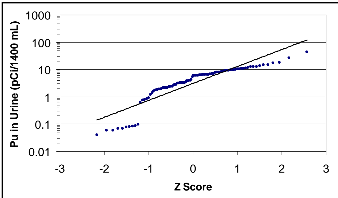
Figure B-2. Plutonium urine sample data through April 18, 1945. The geometric mean = 3.1 pCi/day, the GSD = 4.2, and r^2 = 0.82 .
