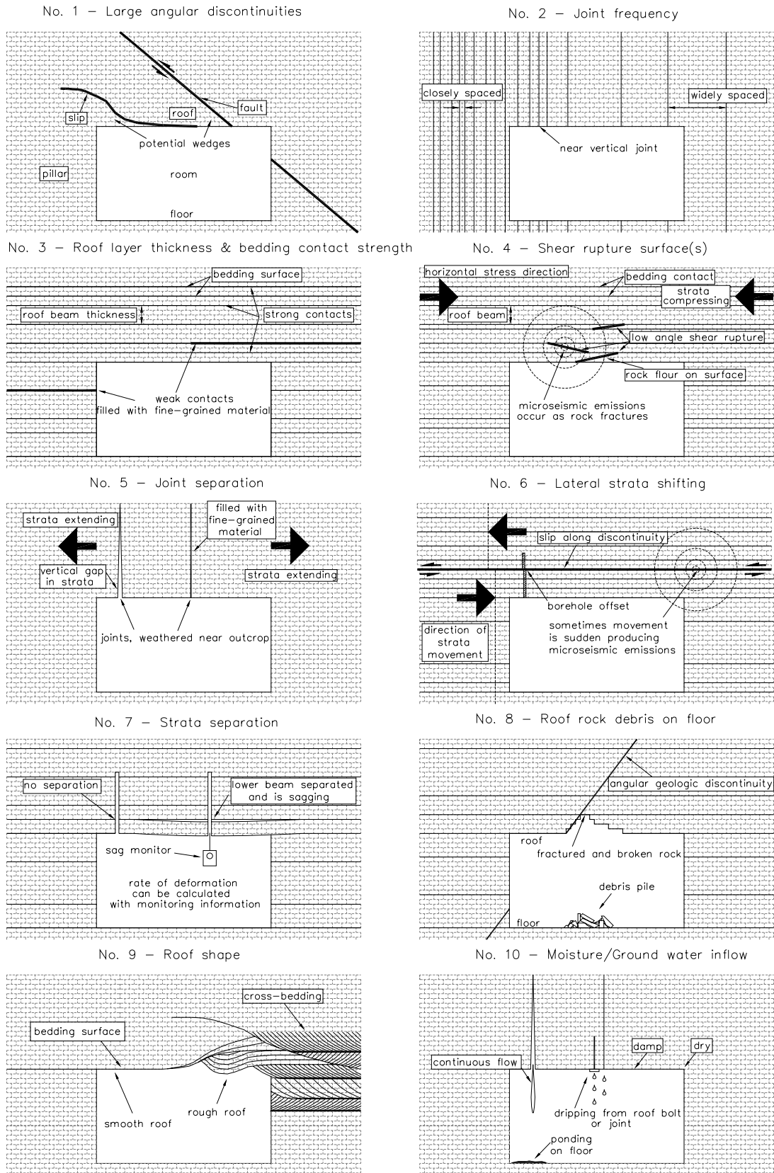
Figure 1. Sketch of parameters associated with the ten defect categories.
