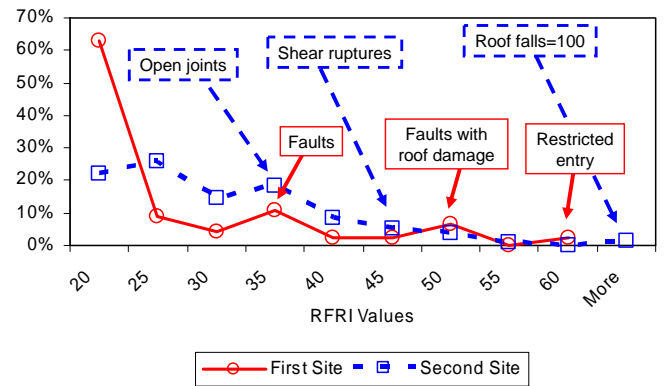
Figure 3. Percentage of RFRI values collected from the two field verification sites.
