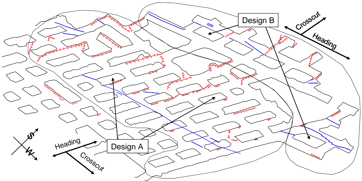
Figure 4. The second field verification site measurement region showing the two mine layout designs. Major defects are also shown where shear ruptures are drawn as tracked features and open joints are drawn as solid lines.
