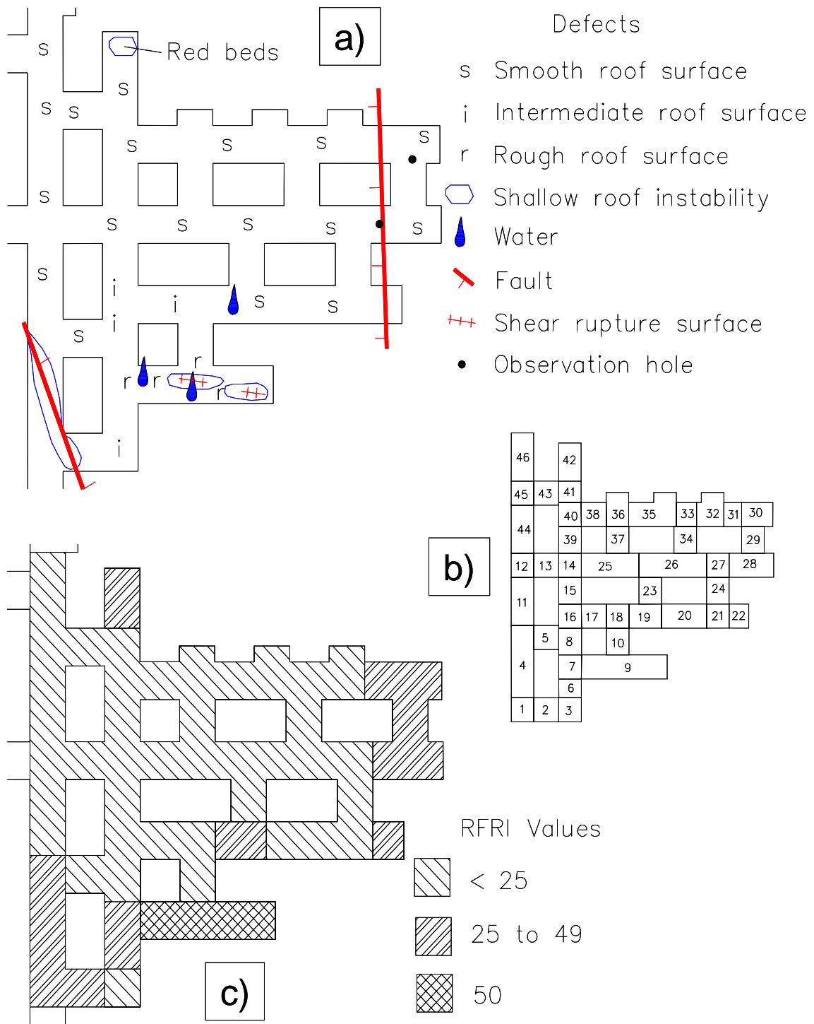
Figure 2. The first field verification site measurement region: a) defects map, b) 46 measurement areas, and c) roof fall risk map displaying the individual RFRI values over the measurement region.
