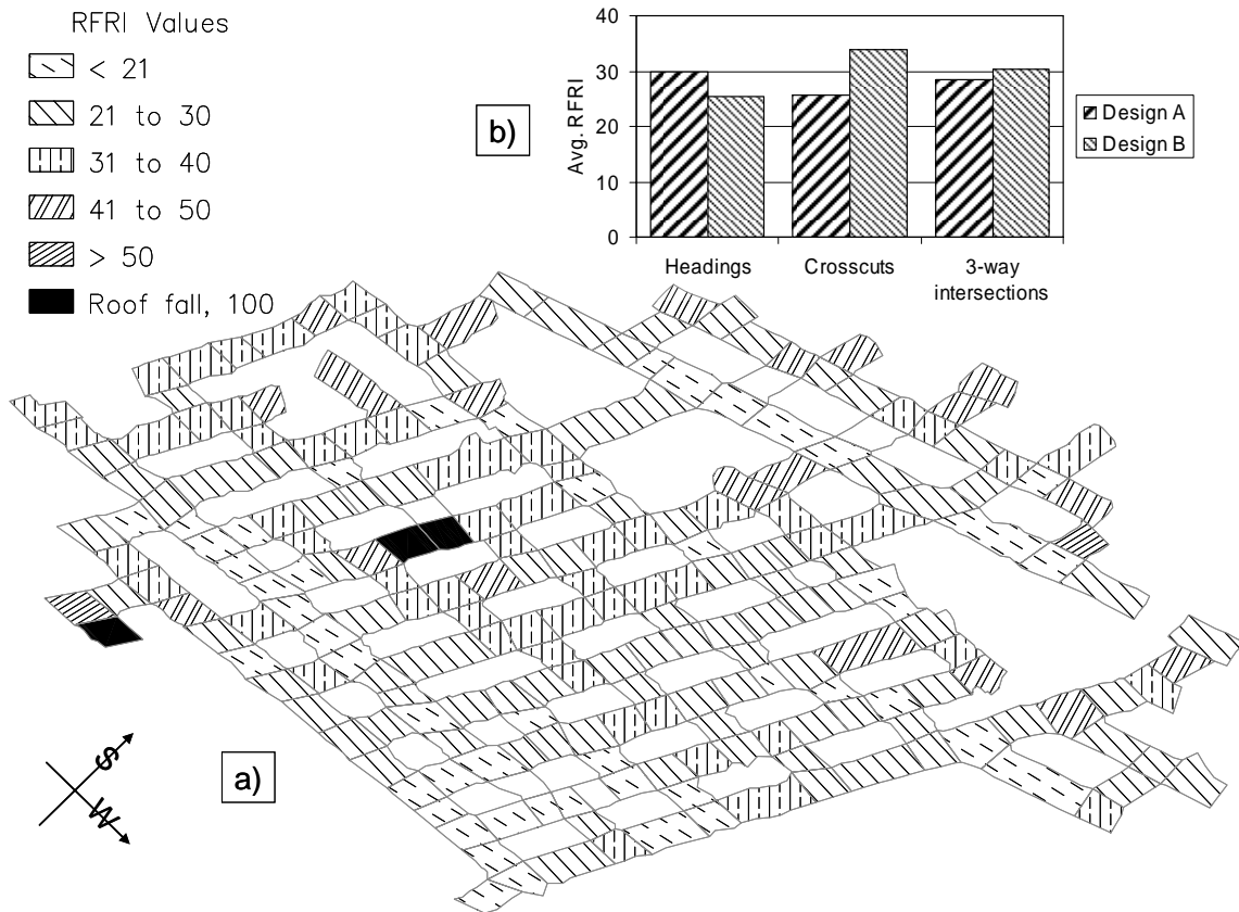
Figure 5. (a) Roof fall risk map displaying the 226 RFRI values over the measurement region. (b) RFRI for different entry characteristics in the Design A and Design B.
