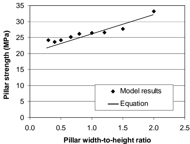
Figure 7. Graph showing modeled pillar strength for a uniform rock mass compared to the Obert-Duval (1967) equation for pillar strength.
