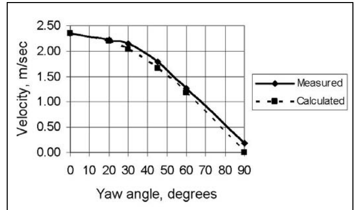
Figure 12. Measured and calculated function of the cosine angle of flow due to yaw angle.
