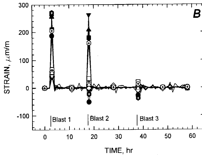
Figure 4. Incremental strain changes after blasts. A, Bolt 1; B, bolt 2.
