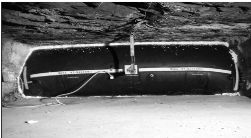
Figure 4. Testing of an inflatable temporary ventilation control device.
