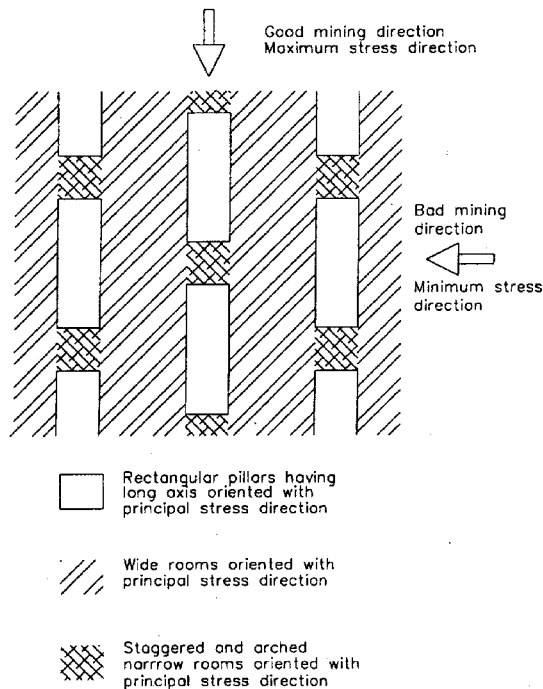
Optimum mine layout for controlling strata in high horizontal-stress conditions.
