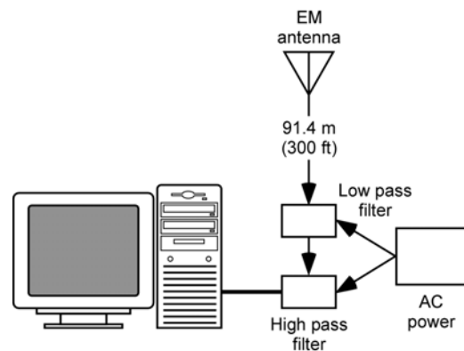
Fig. 2 Schematic of data acquisition
