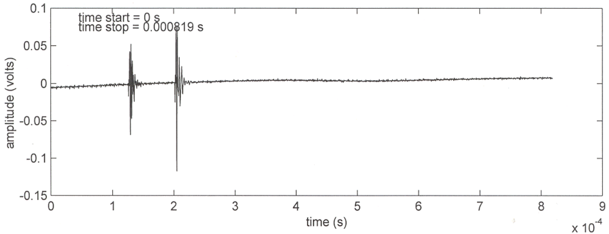
Fig. 4 Air door (electrical noise) waveform.
