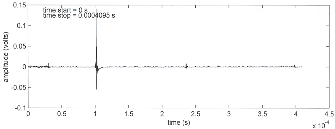
Fig. 6 EM event recorded during blasting
