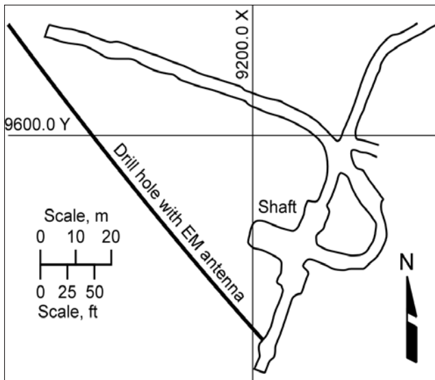
Fig. 3 Plan view of downhole antenna
