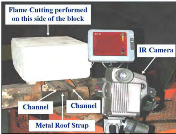
Setup of block and metal roof strap experiment.
