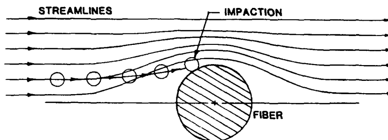
FIGURE 2-15. Impaction capture mechanism 1
