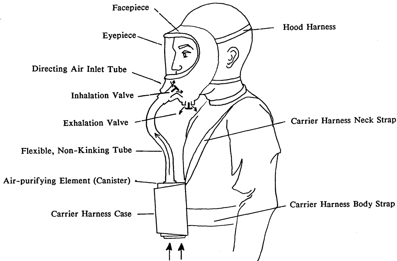
FIGURE 2-29. Typical front- and back-mounted canister gas mask
