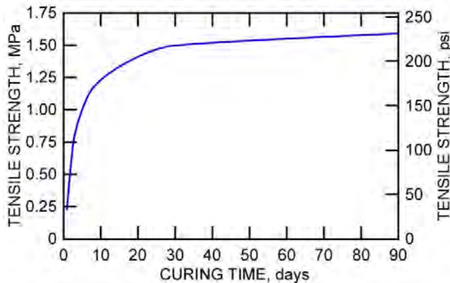
Figure 60. Typical shotcrete tensile strength test results for 0–90 day cure time (n=54).
