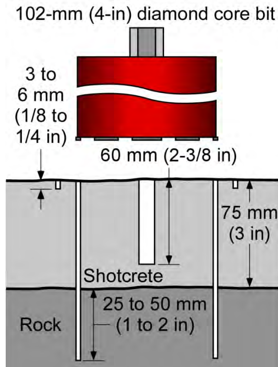
Figure 57. Schematic showing a vertical cross-section of the drill hole configuration for a shotcrete bond strength test.
