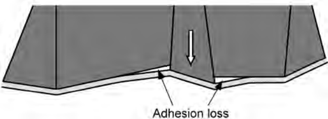
Figure 22. Flexural failure of shotcrete resulting from insufficient adhesion strength, after Kuchta [2002].
