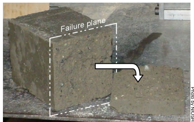
Figure 43. Shotcrete sample showing exposed failure plane.
