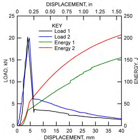
Figure 102. Comparison of load versus displacement and energy versus displacement curves for 1.87\text{-kg/m}^3 ( 3.15\text{-lb/yd}^3 ) Performax fiber mix with 28-day cure time.
