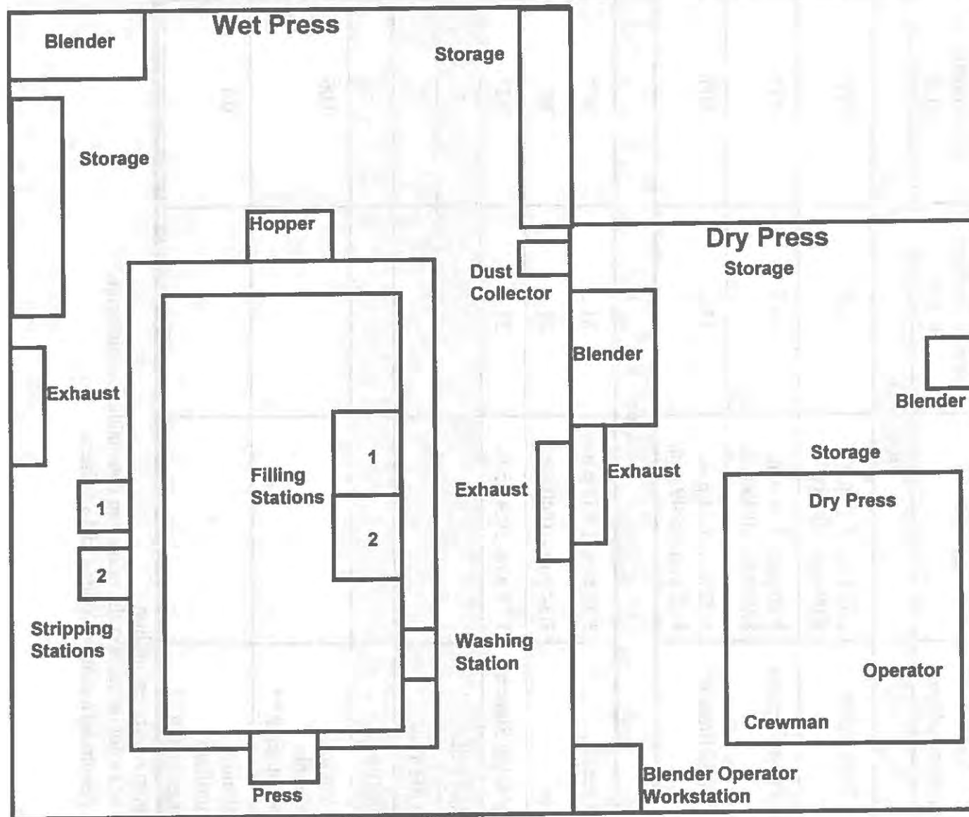
Figure 1 - Wet and Dry Press Areas North American Refractories Co. HETA 95-0147
