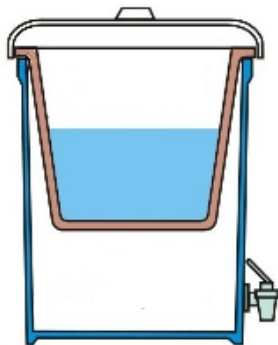
Ceramic filter system design Potters for Peace
