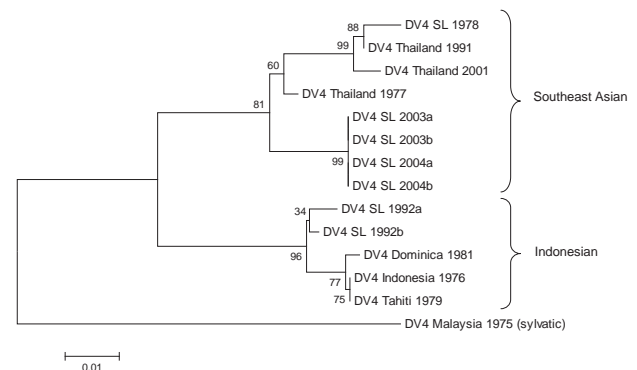
Figure 7. Phylogram of dengue serotype 4 viruses (DENV-4) from Sri Lanka (SL), 1978–2004, and other DENV-4 viruses. The tree is based on a 296-bp fragment for positions 787–1083 coding for portions of premembrane and envelope proteins. The tree was constructed as described in Figure 4 and rooted by using a sylvatic DENV-4 strain. Classification and naming of different DENV-4 genotypes is based on the report by Rico-Hesse (5). Scale bar represents number of base substitutions per site.
