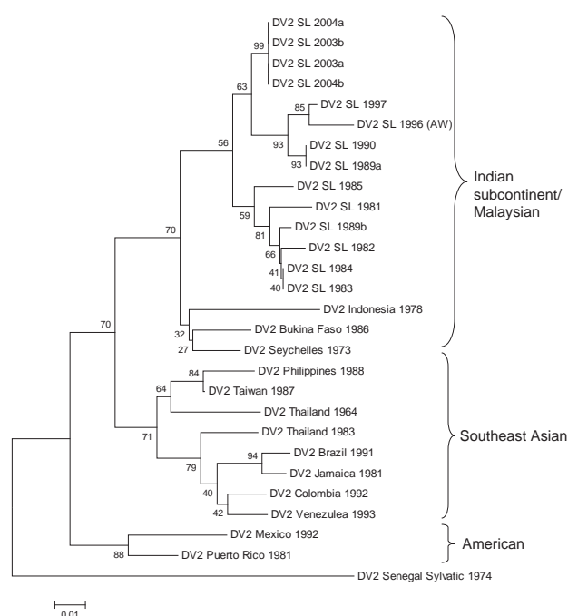
Figure 5. Phylogram of dengue serotype 2 viruses (DENV-2) from Sri Lanka (SL), 1981–2004, and other DENV-2 viruses. The tree is based on a 239-bp fragment for positions 2311–2550 coding for amino acids at the envelope protein/nonstructural protein 1 junction. The tree was constructed as described in Figure 4 and was rooted by using a DENV-2 sylvatic strain. Classification and naming of different DENV-2 genotypes is based on the report by Rico-Hesse (5). Scale bar represents number of base substitutions per site.
