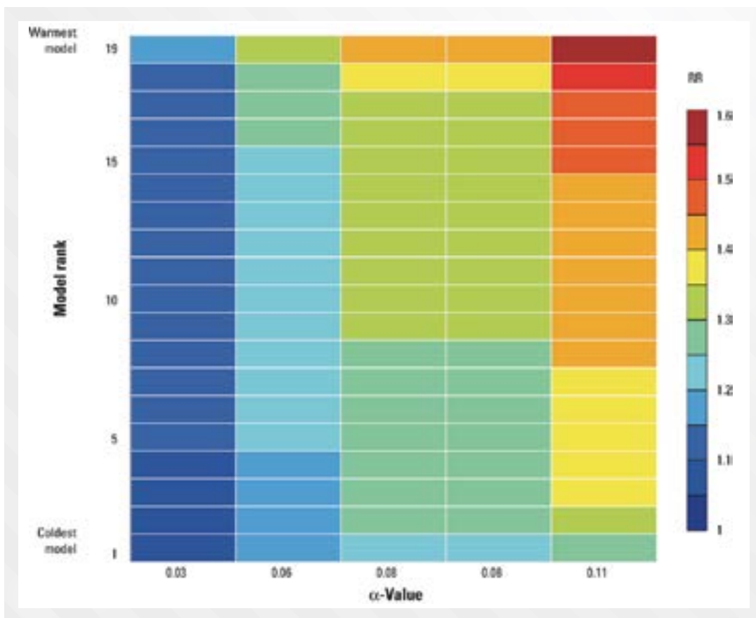
Figure 8. Schematic illustrating the effect of model choice and \alpha on the magnitude of diarrheal disease estimates. In this case, estimates are expressed as relative risk of diarrheal disease in the setting of climate change relative to the risk without. From Kolstad and Johansson, 105 used with permission.
