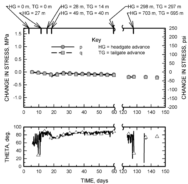
Figure 8.—Horizontal stress change and direction versus time as measured by BSM 3, mine B. Theta zero direction is direction of longwall advance, and counterclockwise is positive in plan view.
