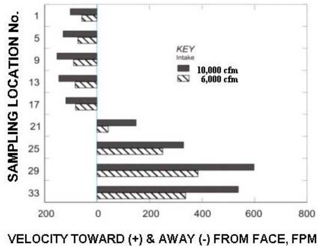
Figure 8. Air speed toward face in 13 ft entry, 2 ft from the left side
