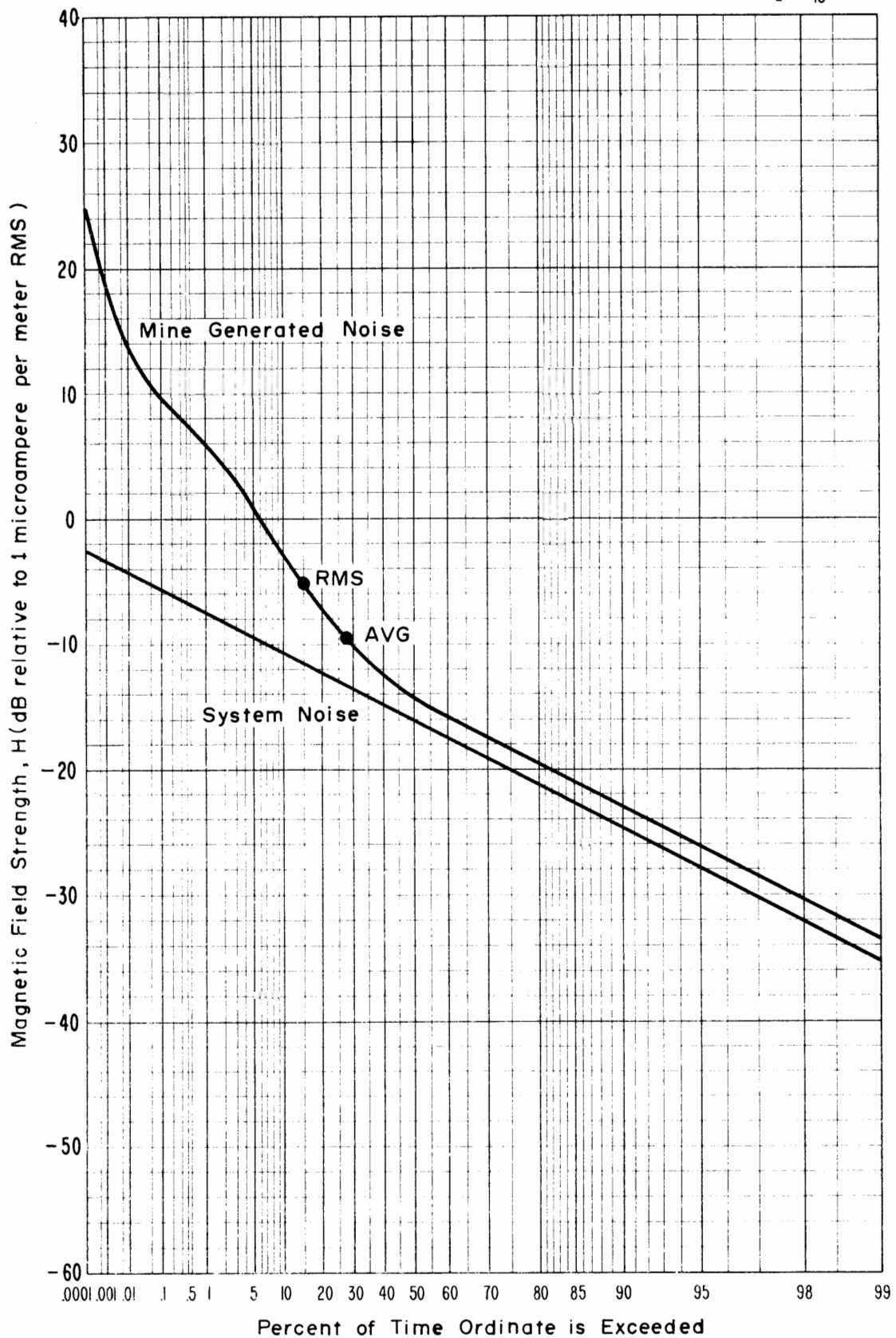
Figure 4-2 APD, Magnetic field strength, 70 kHz, Horizontal (North-South) component, Headframe, Lucky Friday Mine, 1 kHz predetection bandwidth. Time was 11:00 a.m., August 27, 1973.
