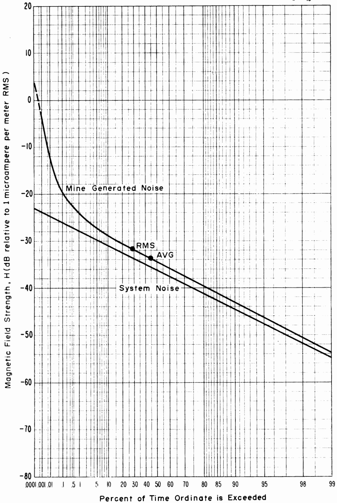
Figure 4-12 APD, Magnetic field strength, 250 kHz, Vertical component, 1450 level, Lucky Friday Mine, 1.2 kHz predetection bandwidth. Time was 1:00 p.m., August 27, 1973.
