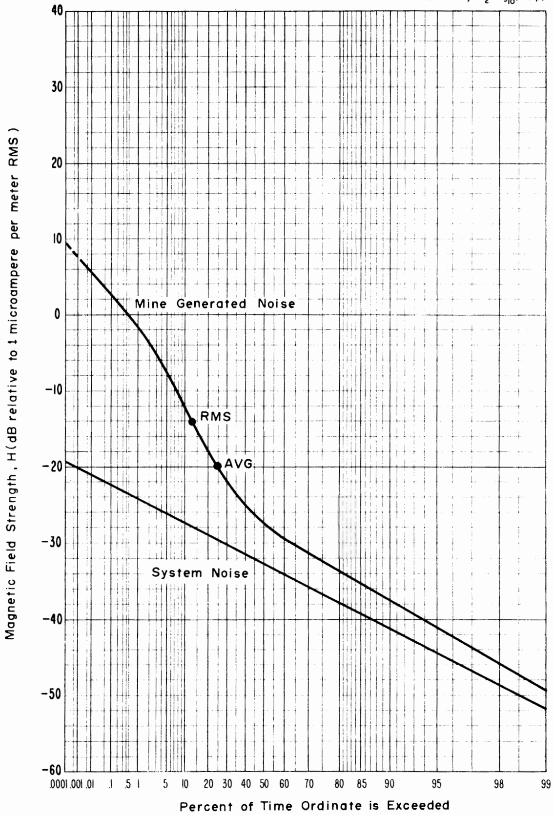
Figure 4-16 APD, Magnetic field strength, 250 kHz, Horizontal (North-South) component, 1450 level, Lucky Friday Mine, 1.2 kHz predetection bandwidth. Time was 1:30 p.m., August 27, 1973.
