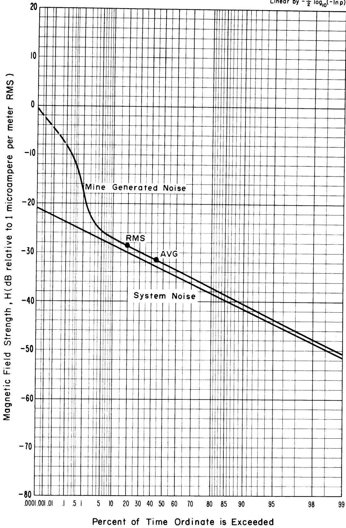
Figure 4-21 APD, Magnetic field strength, 70 kHz, Vertical component, 3050 level, Lucky Friday Mine, 1 kHz predetection bandwidth. Time was 2:30 p.m., August 27, 1973.
