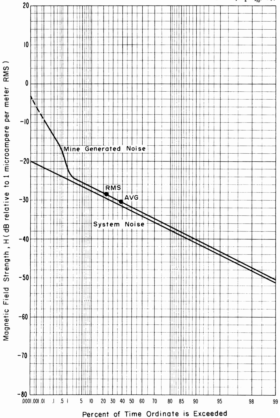
Figure 4-22 APD, Magnetic field strength, 150 kHz, Vertical component, 3050 level, Lucky Friday Mine, 1.2 kHz pre-detection bandwidth. Time was 2:30 p.m., August 27, 1973.
