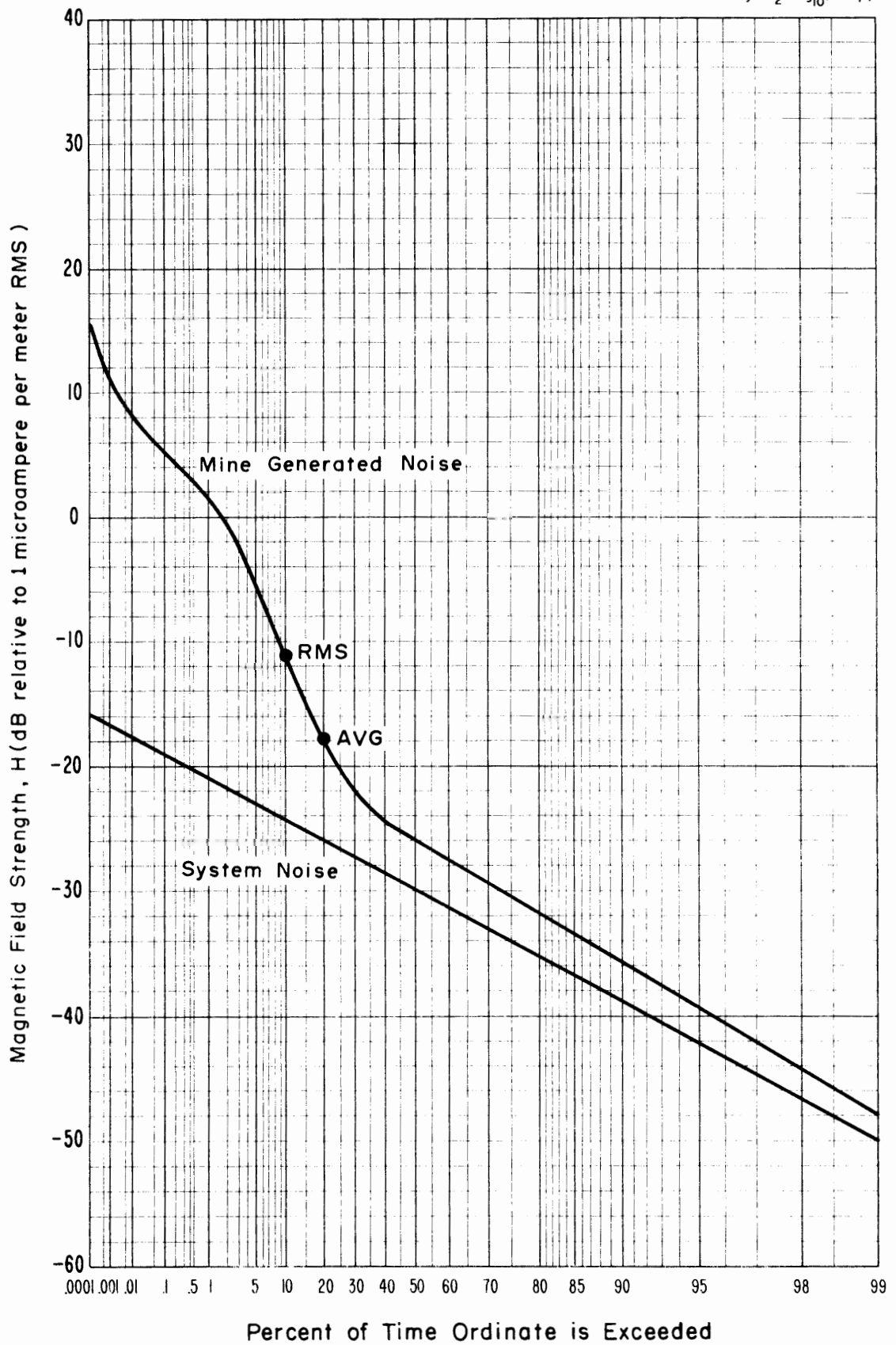
Figure 4-8 APD, Magnetic field strength, 250 kHz, Vertical component, Headframe, Lucky Friday Mine, 1.2 kHz predetection bandwidth. Time was 10:30 a.m., August 27, 1973.
