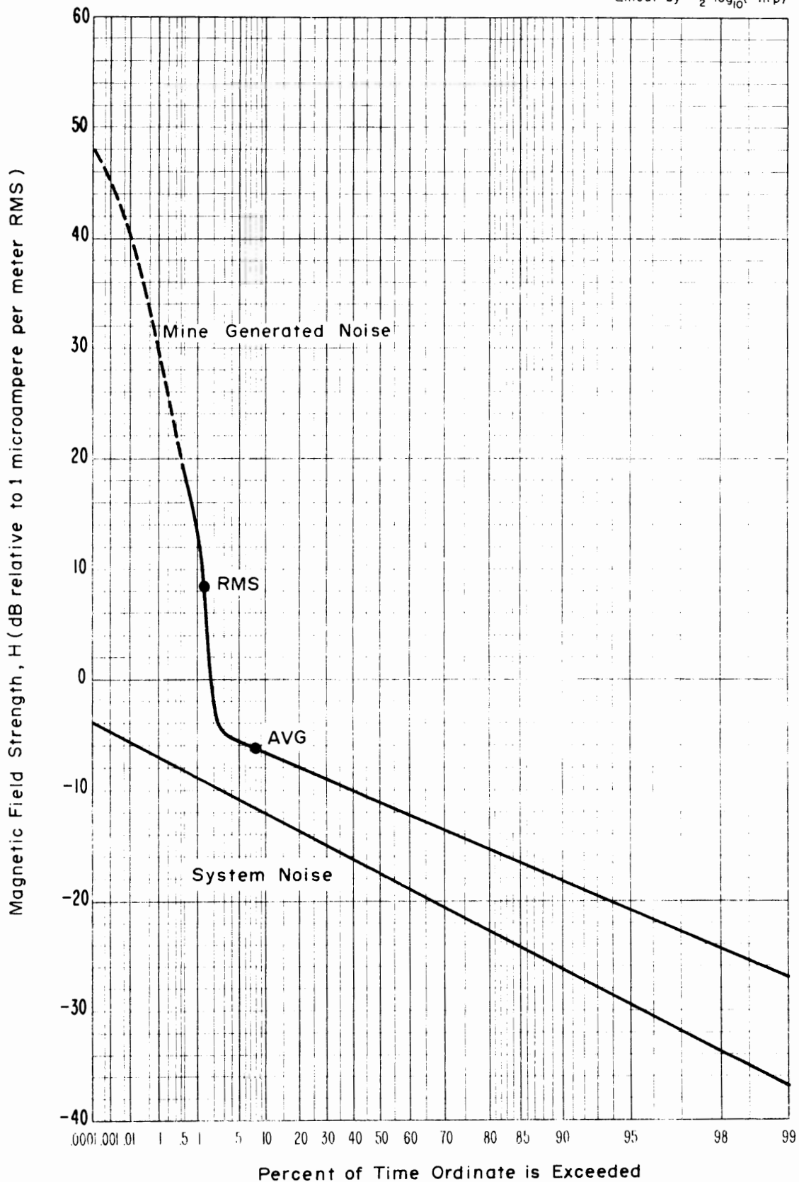
Figure 4-17 APD, Magnetic field strength, 30 kHz, Horizontal (North-South) component, 3050 level, Lucky Friday Mine, 1 kHz predetection bandwidth. Time was 3:00 p.m., August 27, 1973.
