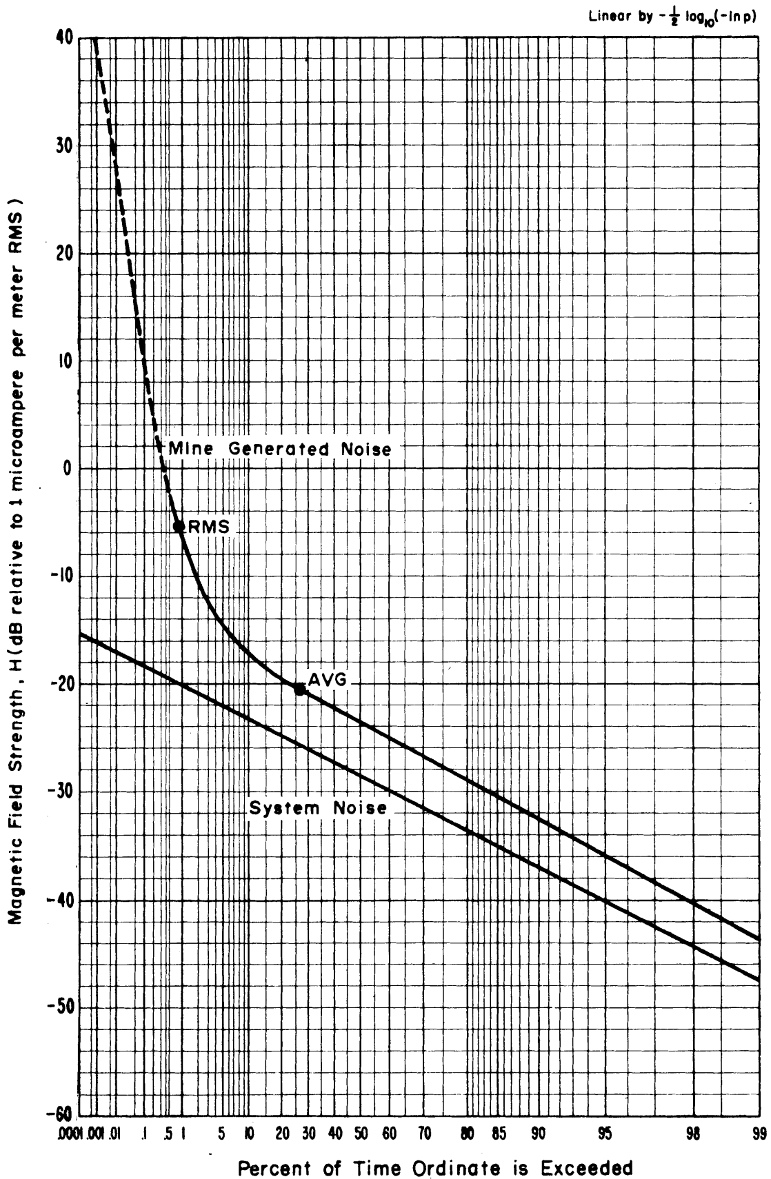
Figure 4-24 APD, Magnetic field strength, 75 kHz, Horizontal (North-South) component, 3650 level, Lucky Friday Mine, 1 kHz predetection bandwidth. Time was 10:00 a.m., February 8, 1974.
