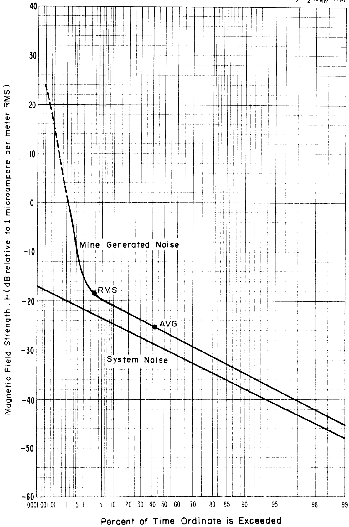
Figure 4-23 APD, Magnetic field strength, 35 kHz, Horizontal (North-South) component, 3650 level, Lucky Friday Mine, 1 kHz predetection bandwidth. Time was 10:00 a.m., February 8, 1974.
