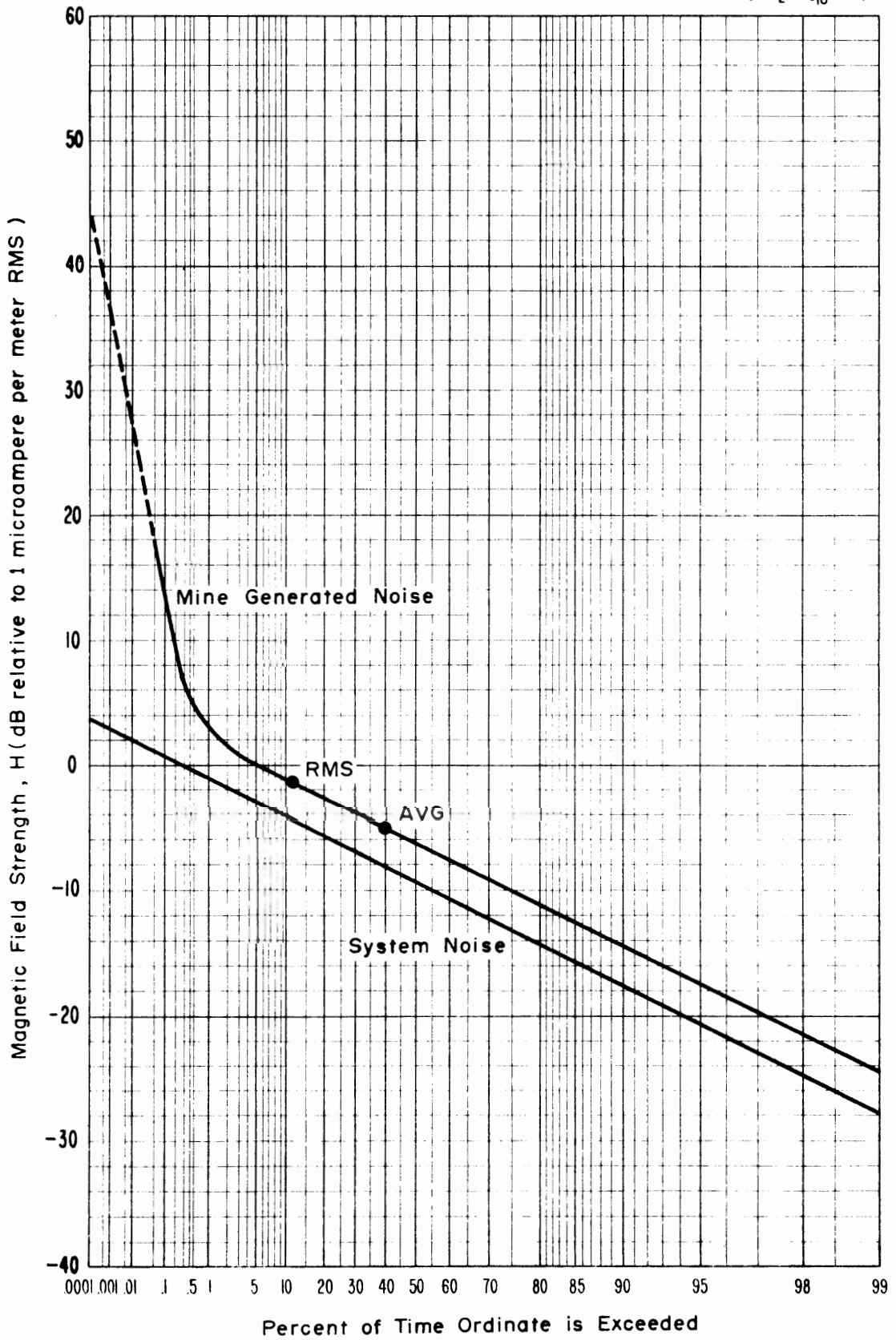
Figure 4-28 APD, Magnetic field strength, 200 kHz, Vertical component, 3650 level, Lucky Friday Mine, 1.2 kHz predetection bandwidth. Time was 10:30 a.m., February 8, 1974.
