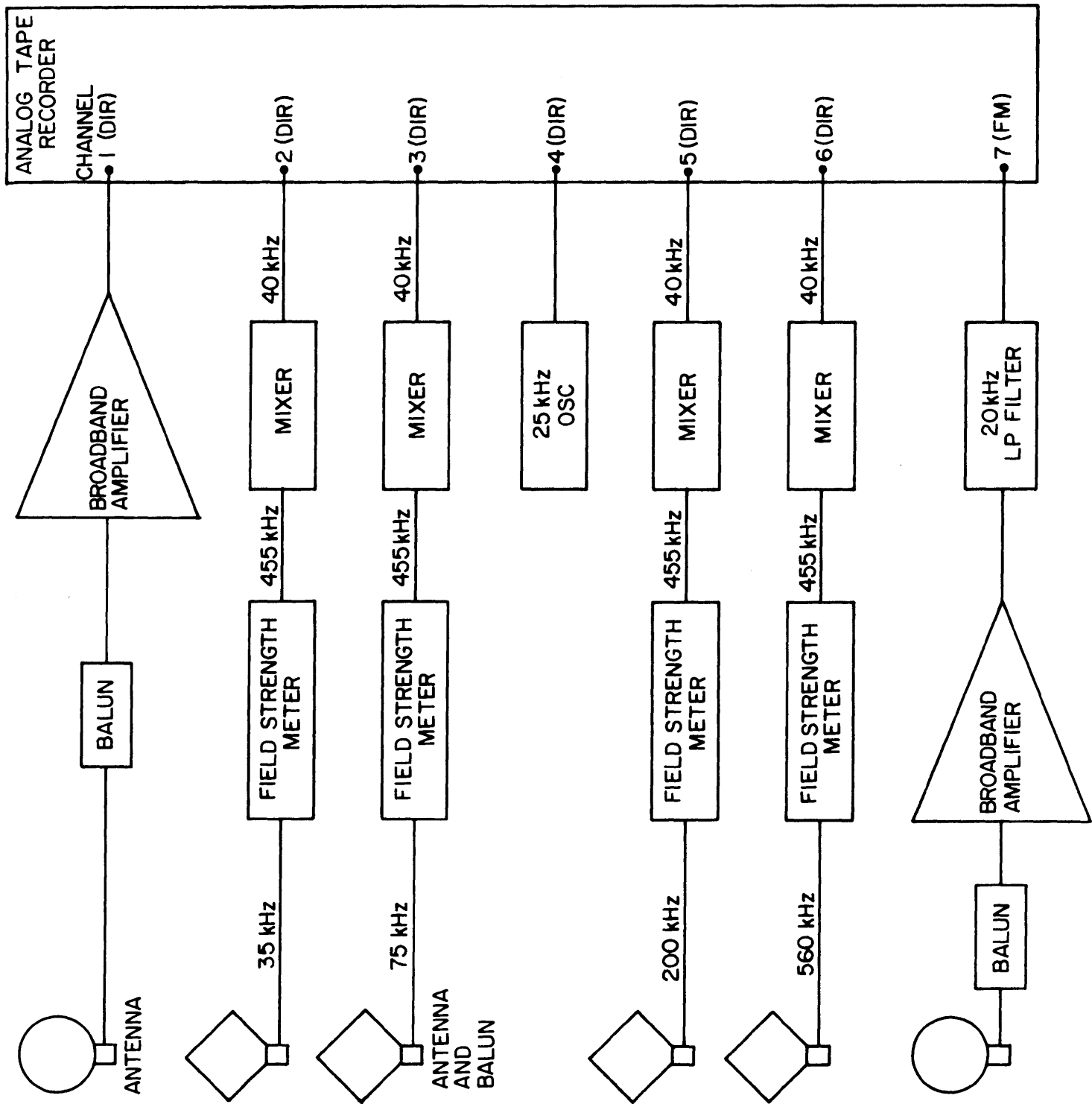
Figure 2-4 Second field recording system, third configuration; it recorded data for APD's on 3650 level.
