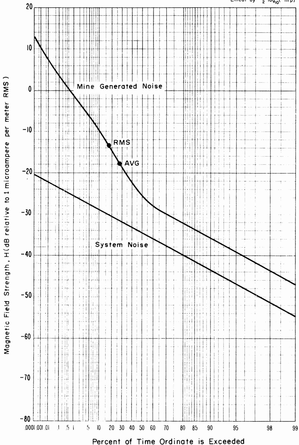
Figure 4-6 APD, Magnetic field strength, 70 kHz, Vertical component, Headframe, Lucky Friday Mine, 1 kHz predetection bandwidth. Time was 10:30 a.m., August 27, 1973.
