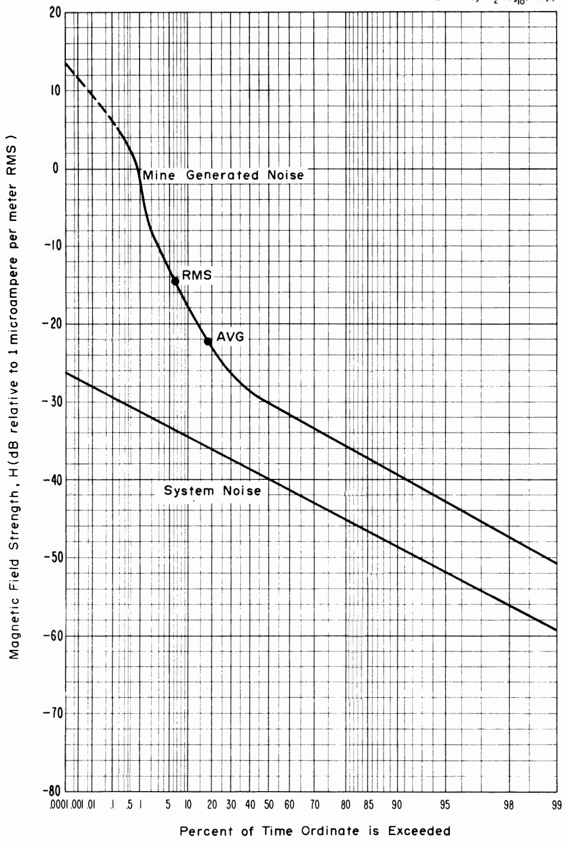
Figure 4-18 APD, Magnetic field strength, 70 kHz, Horizontal (North-South) component, 3050 level, Lucky Friday Mine, 1 kHz predetection bandwidth. Time was 3:00 p.m., August 27, 1973.
