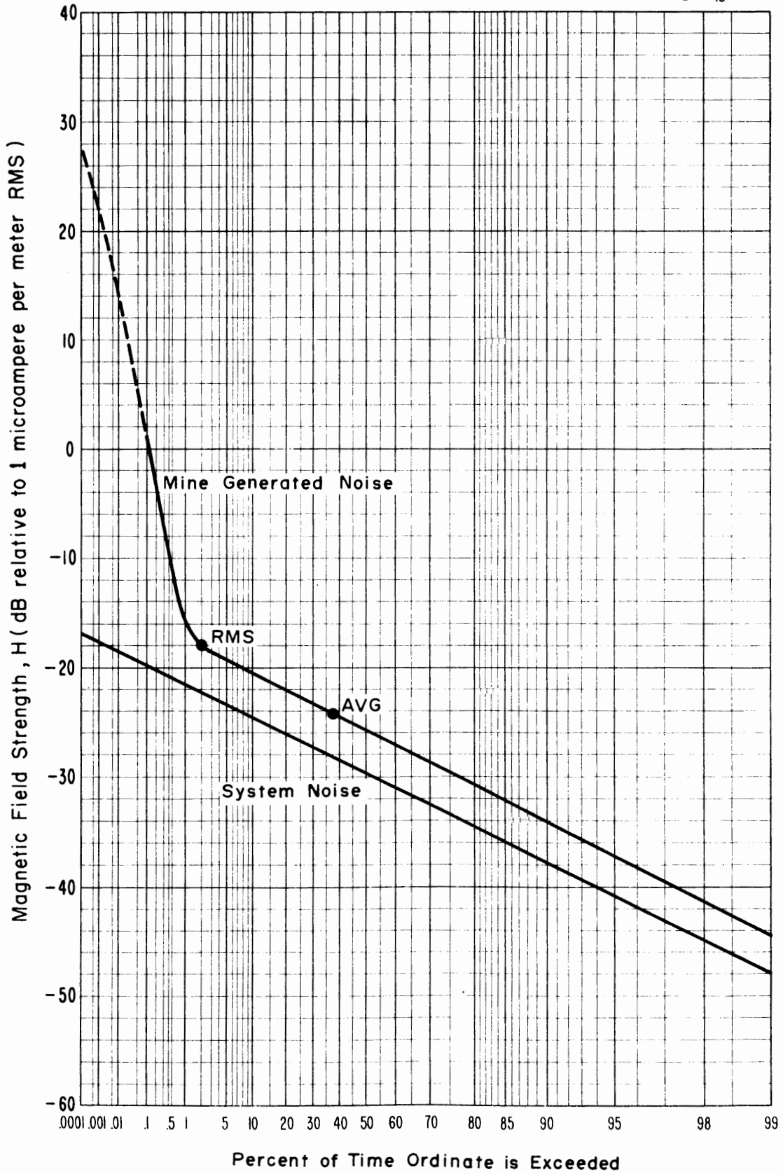
Figure 4-26 APD, Magnetic field strength, 35 kHz, Vertical component, 3650 level, Lucky Friday Mine, 1 kHz predetection bandwidth. Time was 10:30 a.m., February 8, 1974.
