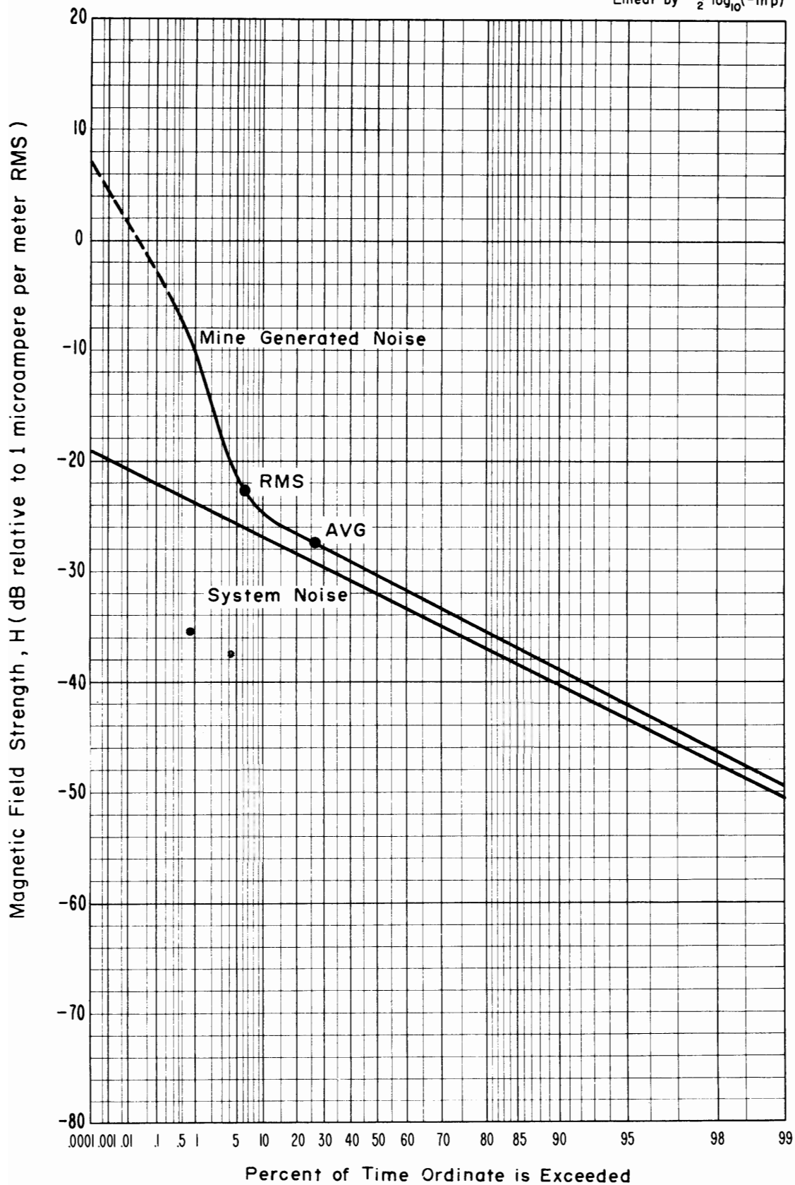
Figure 4-19 APD, Magnetic field strength, 150 kHz, Horizontal (North-South) component, 3050 level, Lucky Friday Mine, 1.2 kHz predetection bandwidth. Time was 3:00 p.m., August 27, 1973.
