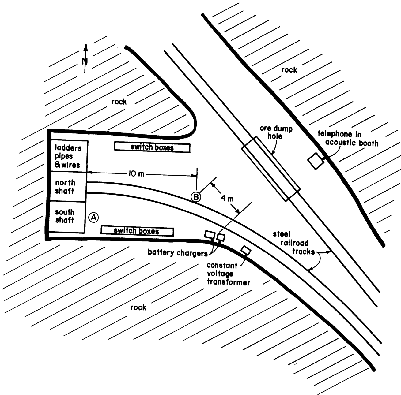
Figure 3-19 Plan view of portion of 4050 level, Lucky Friday Mine. Antennas were located at A and B.
