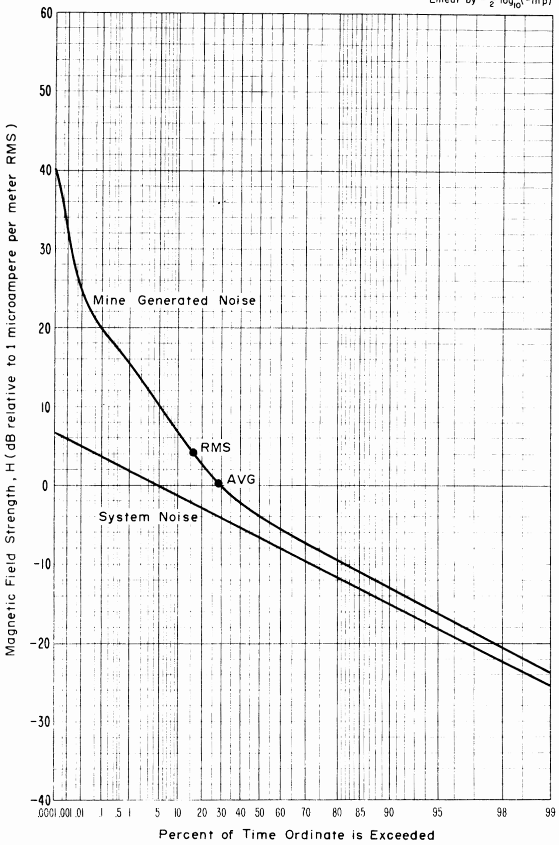
Figure 4-1 APD, Magnetic field strength, 30 kHz, Horizontal (North-South) component, Headframe, Lucky Friday Mine, 1 kHz predetection bandwidth. Time was 11:00 a.m., August 27, 1973.
