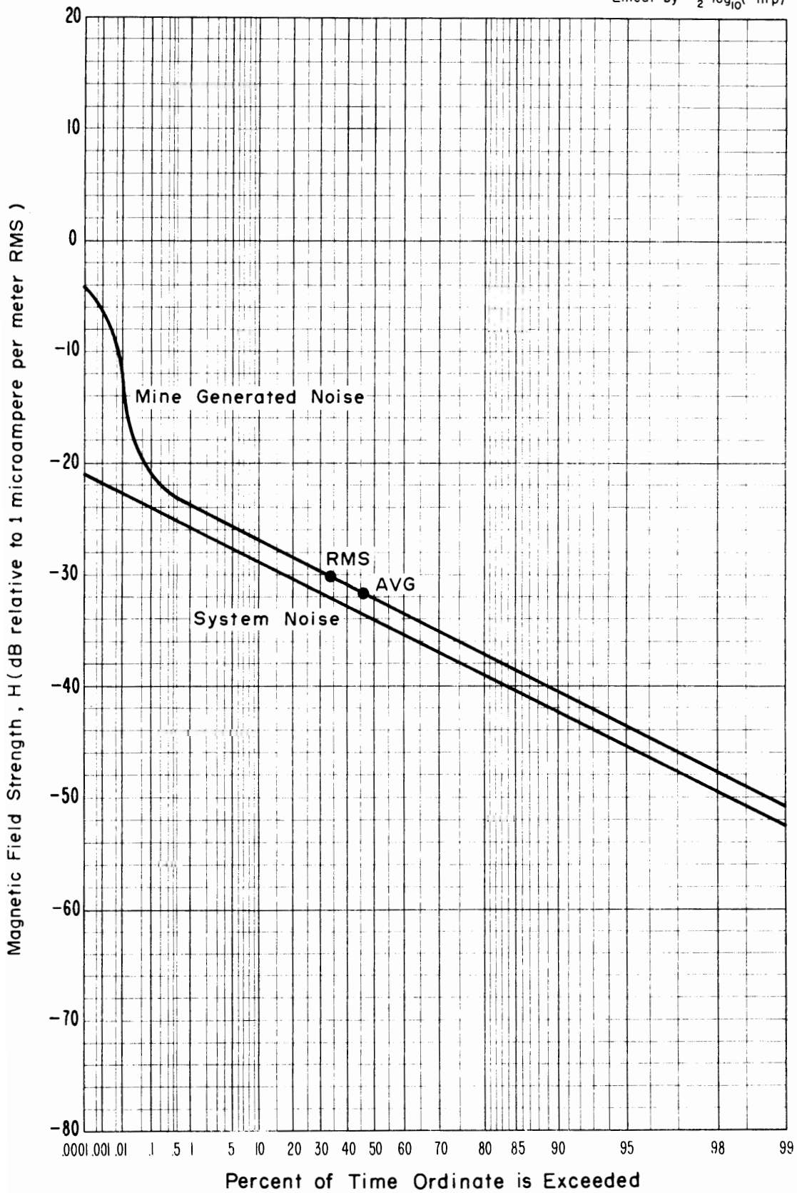
Figure 4-11 APD, Magnetic field strength, 150 kHz, Vertical component, 1450 level, Lucky Friday Mine, 1.2 kHz predetection bandwidth. Time was 1:00 p.m., August 27, 1973.
