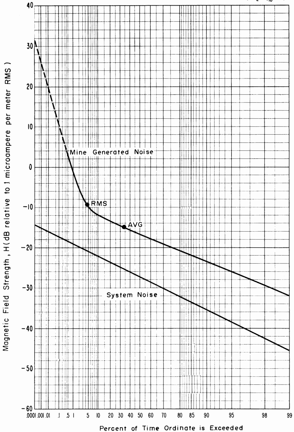
Figure 4-20 APD, Magnetic field strength, 30 kHz, Vertical component, 3050 level, Lucky Friday Mine, 1 kHz predetection bandwidth. Time was 2:30 p.m., August 27, 1973.
