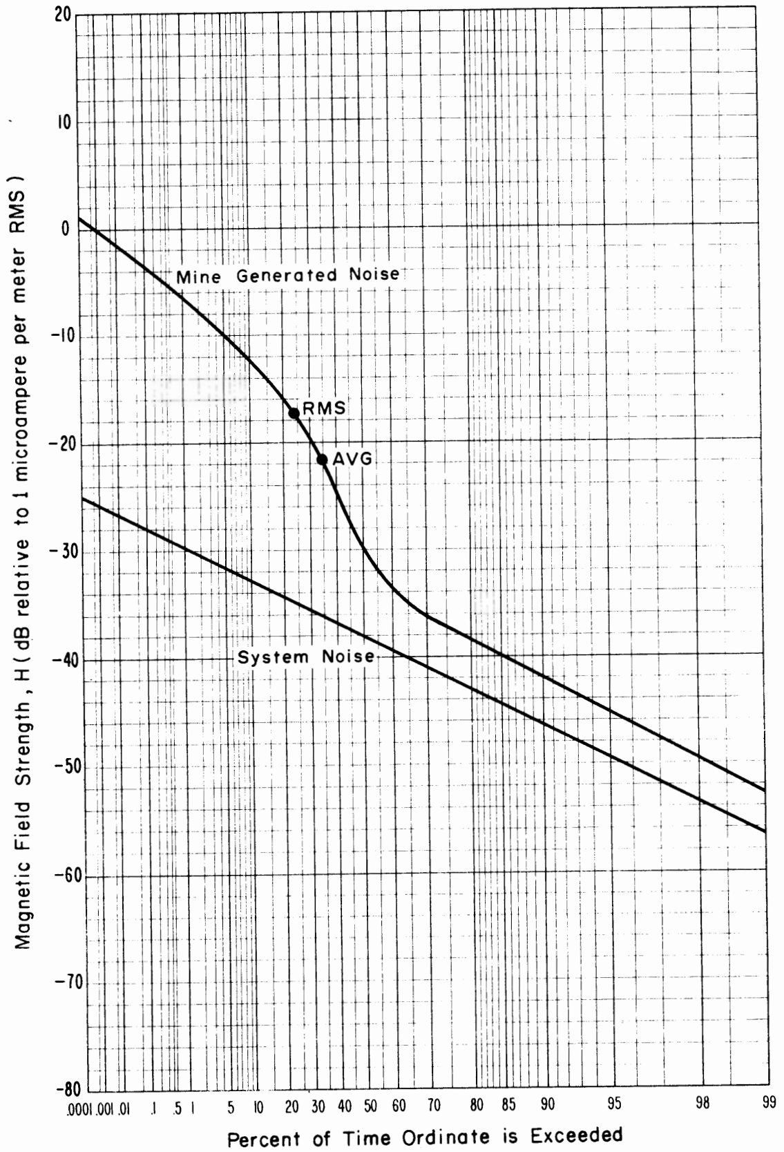
Figure 4-10 APD, Magnetic field strength, 70 kHz, Vertical component, 1450 level, Lucky Friday Mine, 1 kHz predetection bandwidth. Time was 1:00 p.m., August 27, 1973.
