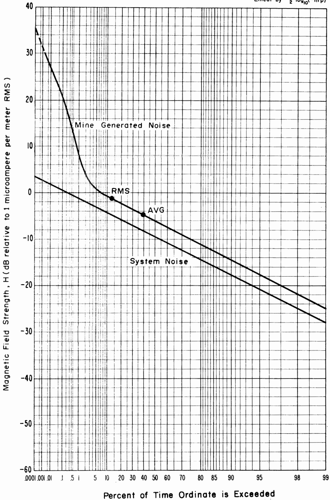
Figure 4-25 APD, Magnetic field strength, 200 kHz, Horizontal (North-South) component, 3650 level, Lucky Friday Mine, 1.2 kHz predetection bandwidth. Time was 10:00 a.m., February 8, 1974.
