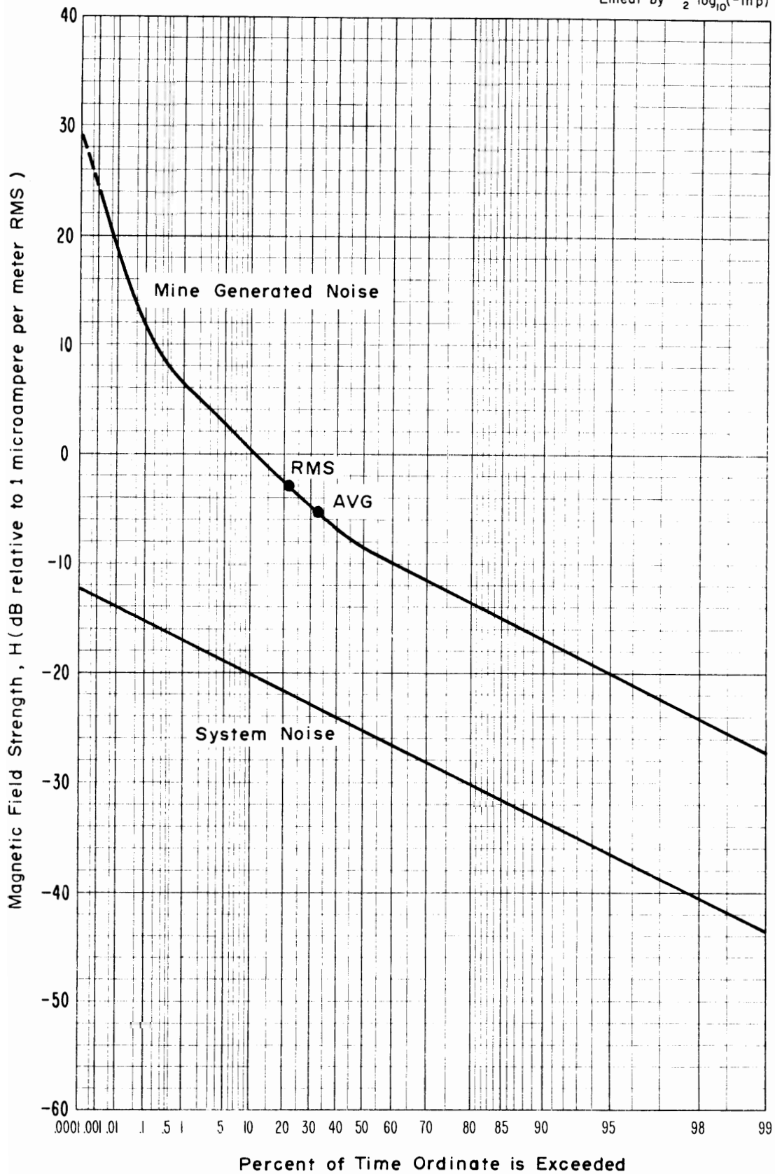
Figure 4-13 APD, Magnetic field strength, 30 kHz, Horizontal (North-South) component, 1450 level, Lucky Friday Mine, 1 kHz predetection bandwidth. Time was 1:30 p.m., August 27, 1973.
