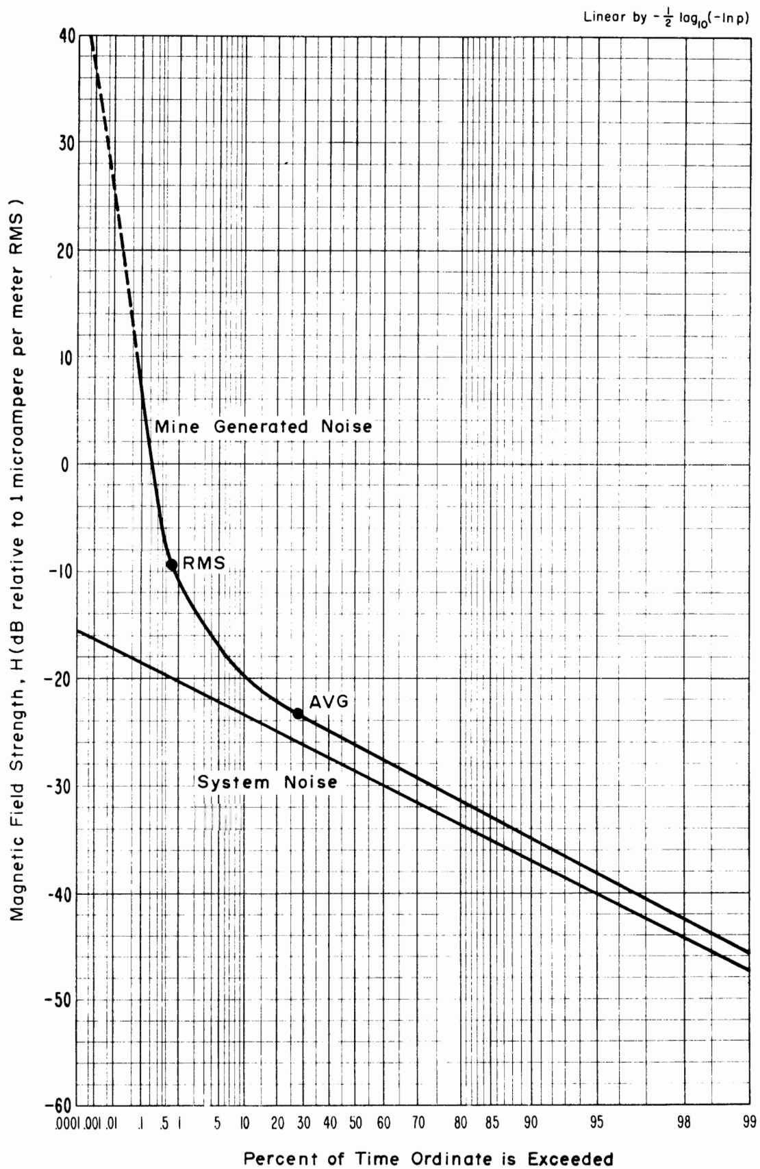
Figure 4-27 APD, Magnetic field strength, 75 kHz, Vertical component, 3650 level, Lucky Friday Mine, 1 kHz predetection bandwidth. Time was 10:30 a.m., February 8, 1974.
