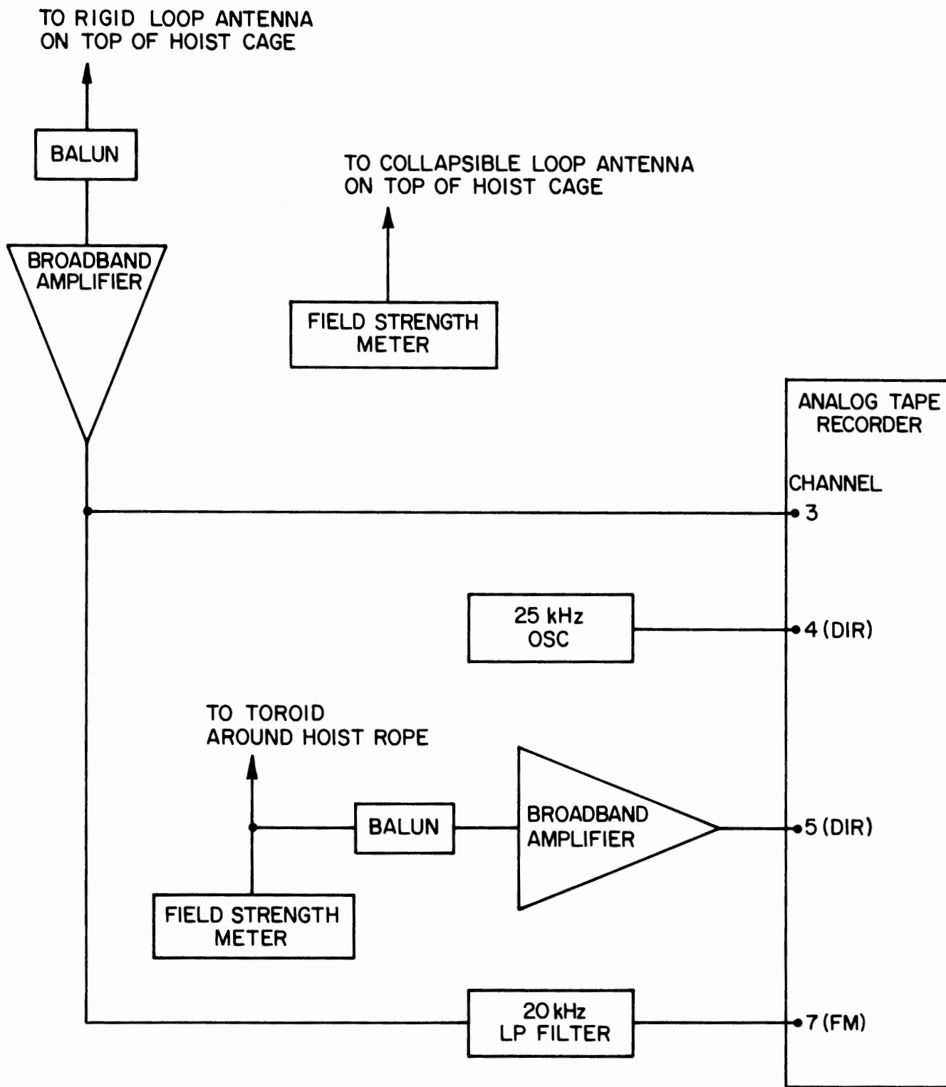
Figure 2-5 Second field recording system, fourth configuration; it was used on hoist runs up and down shaft.
