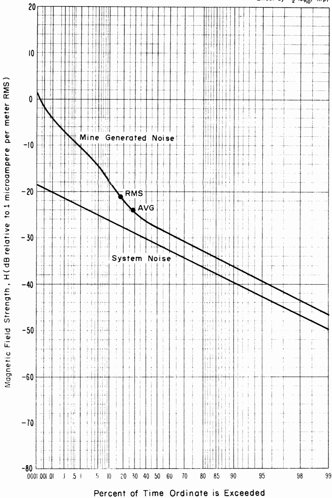
Figure 4-7 APD, Magnetic field strength, 150 kHz, Vertical component, Headframe, Lucky Friday Mine, 1.2 kHz predetection bandwidth. Time was 10:30 a.m., August 27, 1973.
