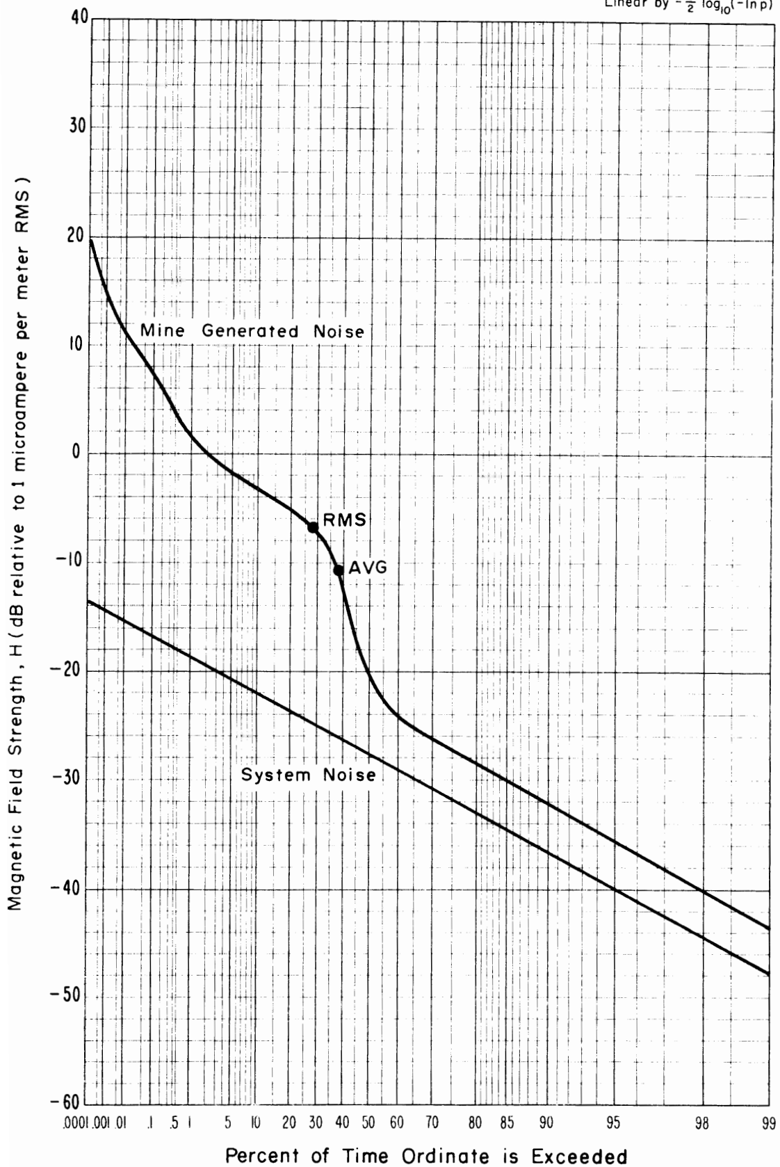
Figure 4-9 APD, Magnetic field strength, 30 kHz, Vertical component, 1450 level, Lucky Friday Mine, 1 kHz predetection bandwidth. Time was 1:00 p.m., August 27, 1973.
