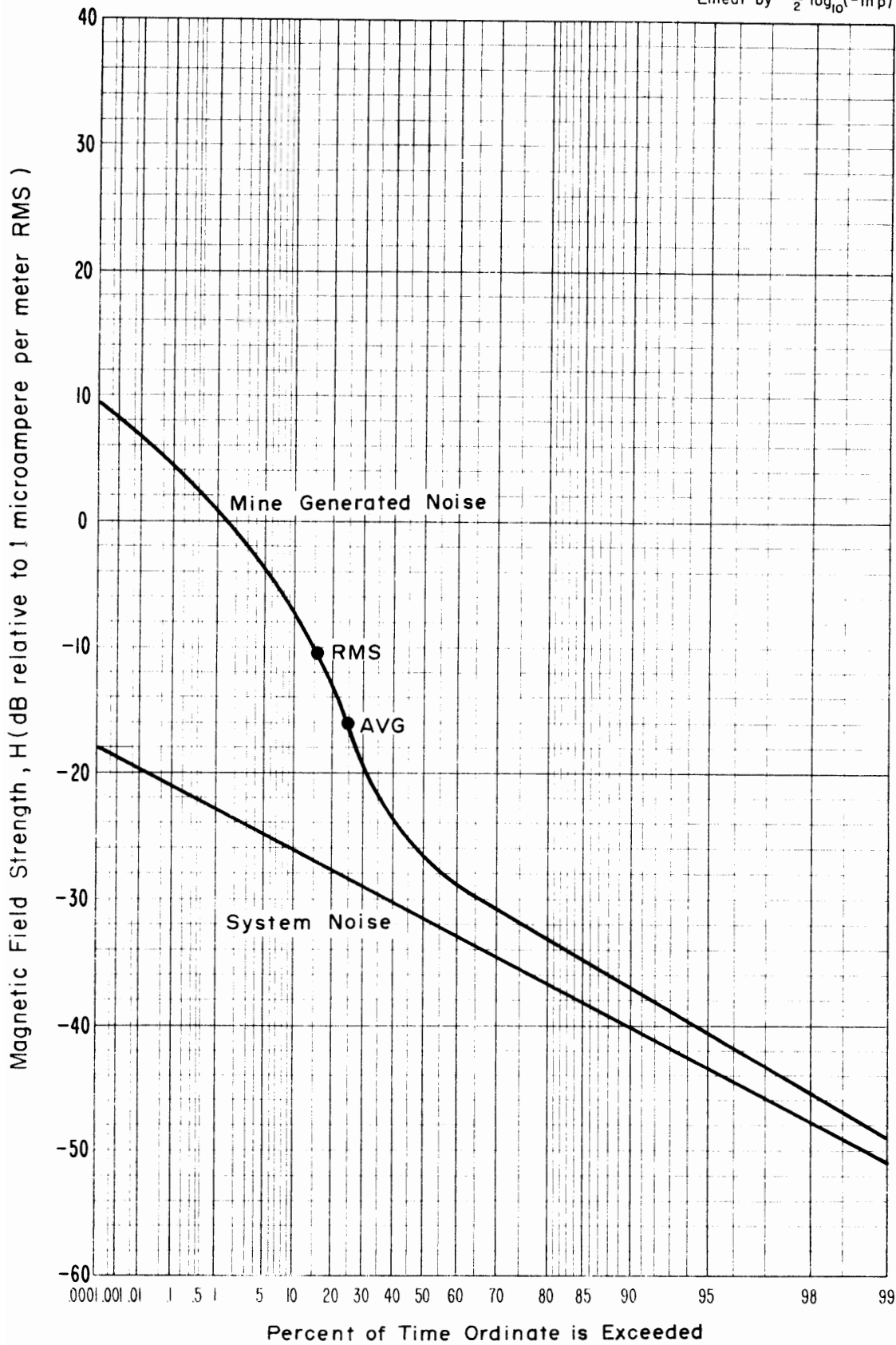
Figure 4-3 APD, Magnetic field strength, 150 kHz, Horizontal (North-South) component, Headframe, Lucky Friday Mine, 1.2 kHz predetection bandwidth. Time was 11:00 a.m., August 27, 1973.
