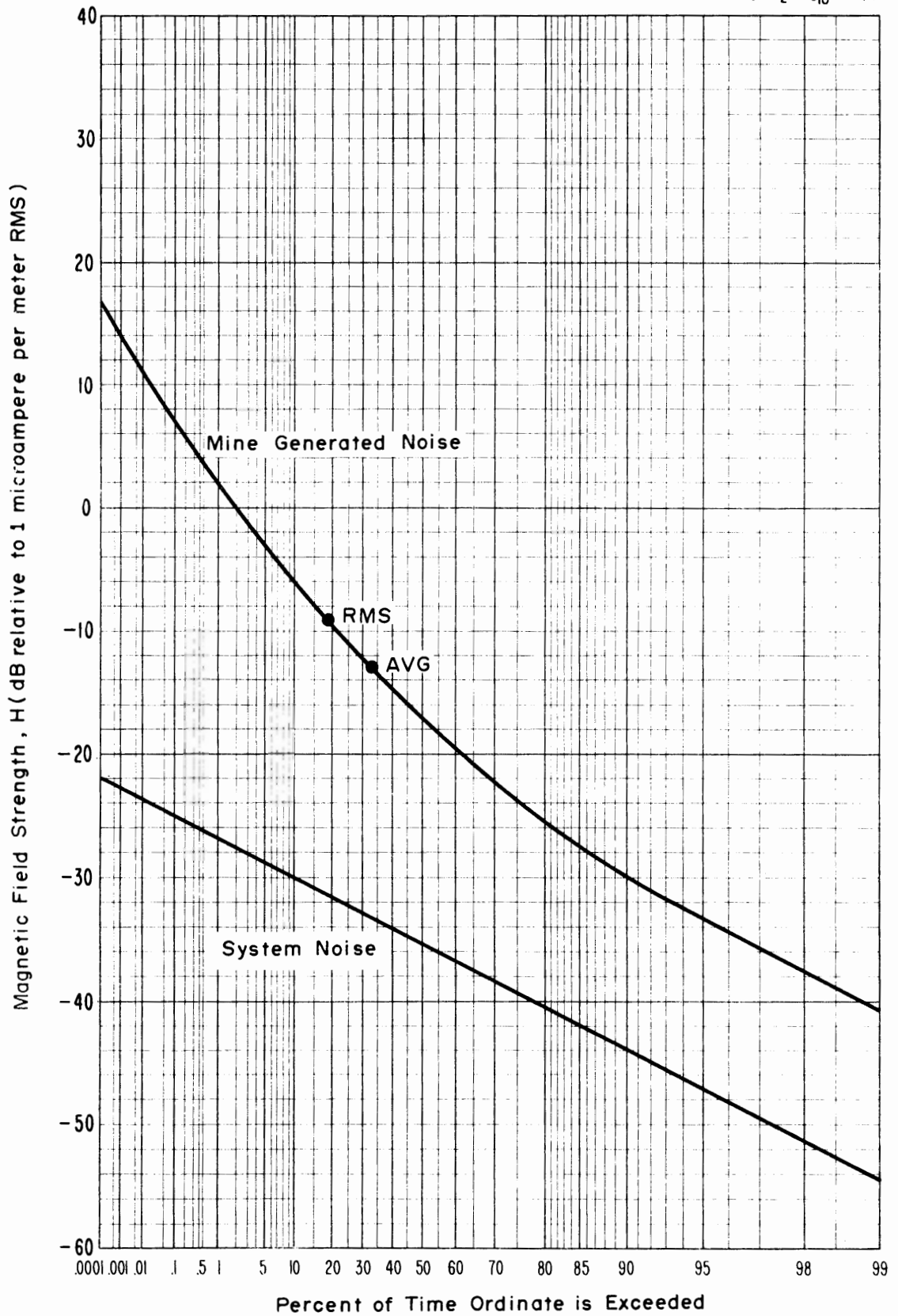
Figure 4-14 APD, Magnetic field strength, 70 kHz, Horizontal (North-South) component, 1450 level, Lucky Friday Mine, 1 kHz predetection bandwidth. Time was 1:30 p.m., August 27, 1974.
