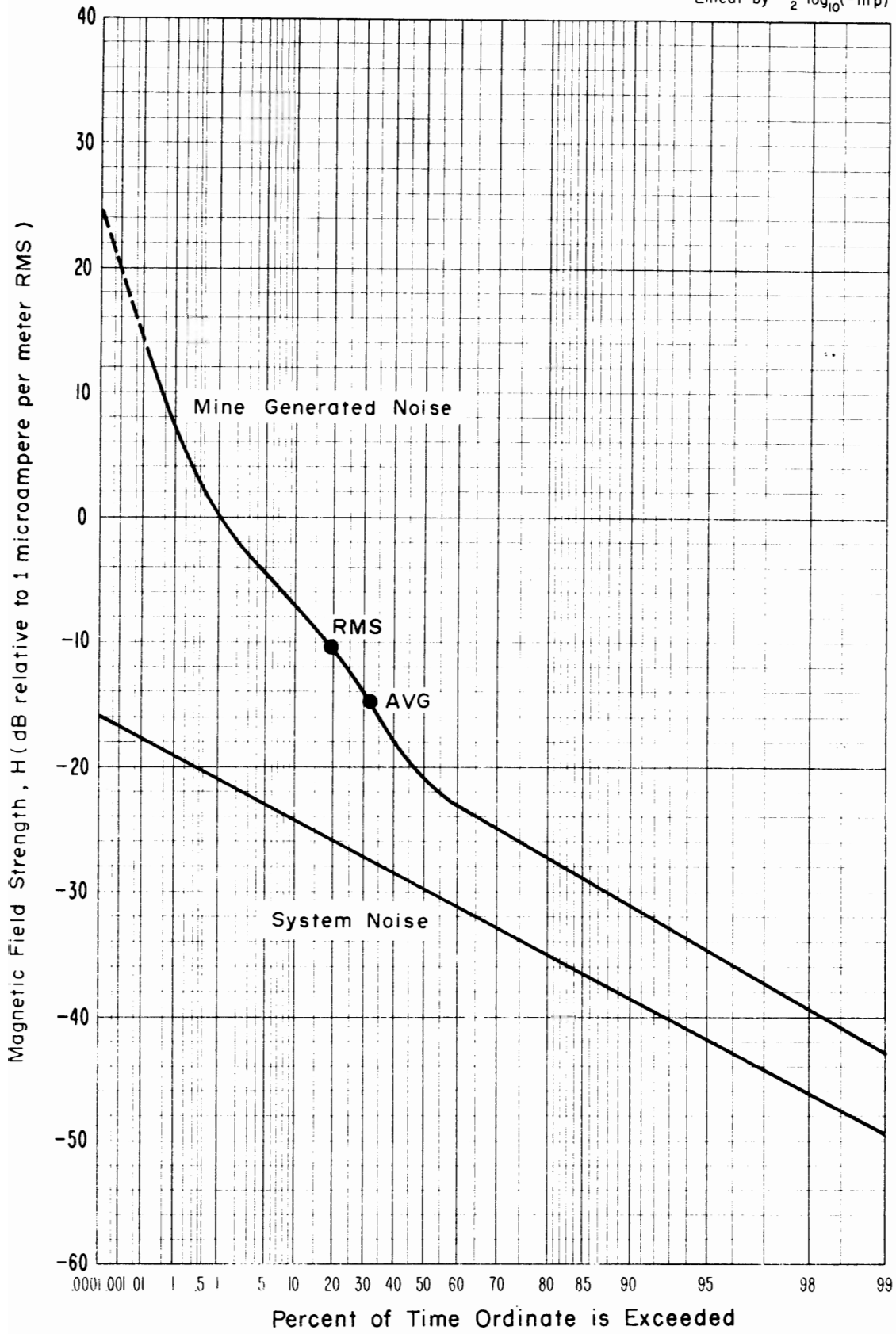
Figure 4-5 APD, Magnetic field strength, 30 kHz, Vertical component, Headframe, Lucky Friday Mine, 1 kHz predetection bandwidth. Time was 10:30 a.m., August 27, 1973.
