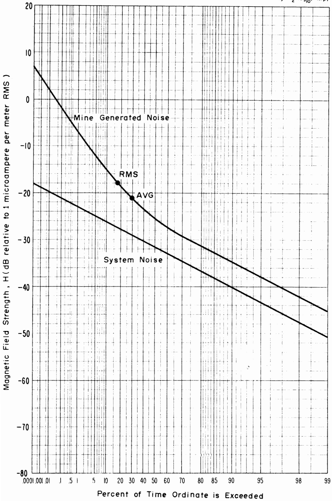
Figure 4-15 APD, Magnetic field strength, 150 kHz, Horizontal (North-South) component, 1450 level, Lucky Friday Mine, 1.2 kHz predetection bandwidth. Time was 1:30 p.m., August 27, 1973.
