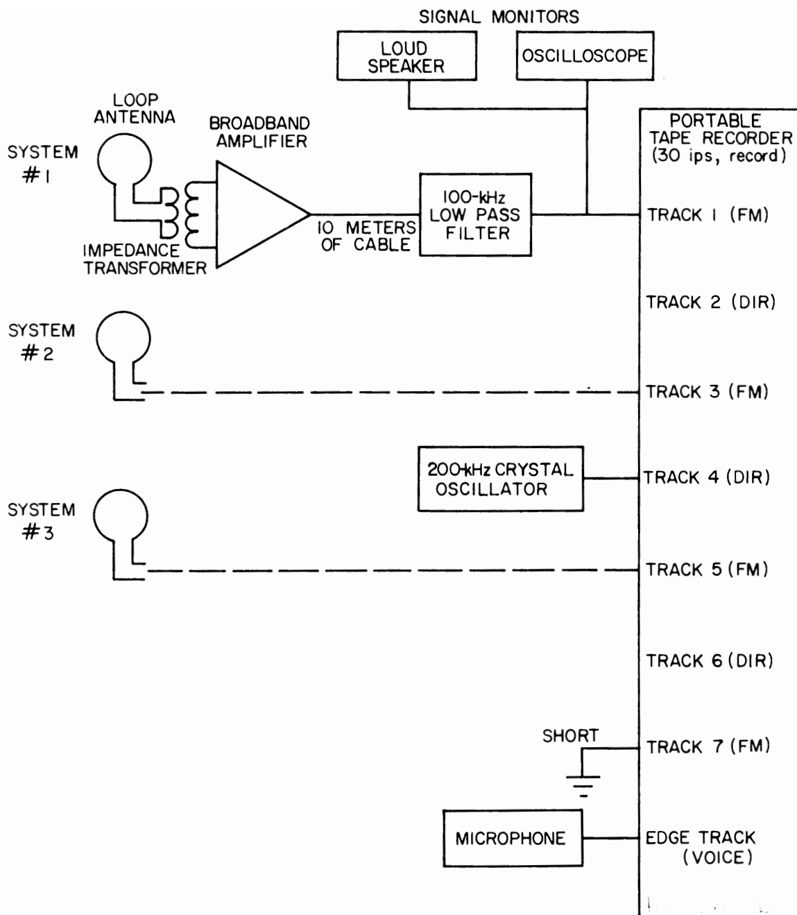
Figure 2-1 Block diagram of portable instrumentation, first system. FM tracks are used to record from 100 Hz to 100 kHz; direct tracks are used from 3 kHz to 320 kHz. Systems 2 and 3 are identical to system 1. When the direct tracks are used, the 100-kHz low pass filters are eliminated, and the amplifier bandwidth is increased from 100 kHz to 300 kHz. The microphone is used for occasional vocal comments by the operator.
