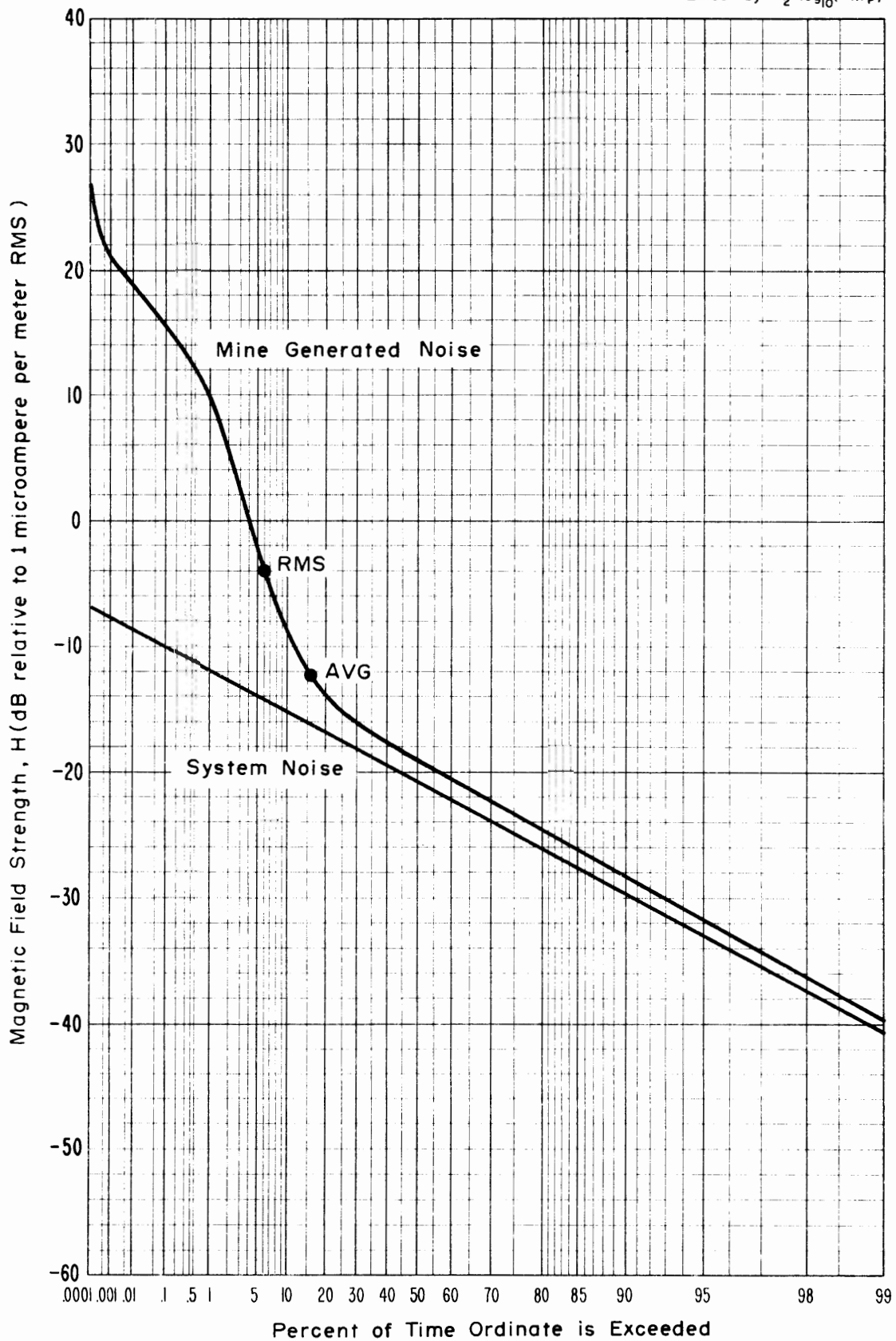
Figure 4-4 APD, Magnetic field strength, 250 kHz, Horizontal (North-South) component, Headframe, Lucky Friday Mine, 1.2 kHz predetection bandwidth. Time was 11:00 a.m., August 27, 1973
