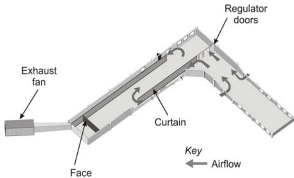
Figure 2. Ventilation Test Gallery.
