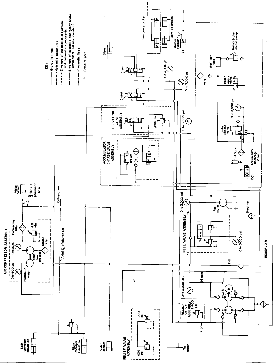
Figure 9.—Modified SC hydraulic system.
