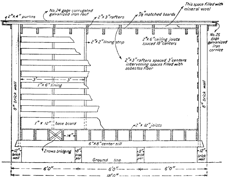
FIGURE 12.—Sections of magazine: A, section at line CD in fig. 11, B; B, section at line AB in fig. 12, A.
