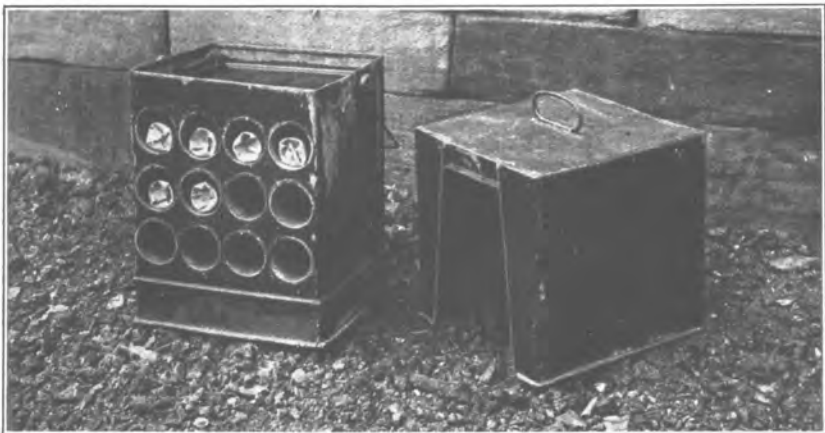
C. THAWER FOR FROZEN EXPLOSIVES.
