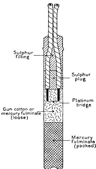
FIGURE 3.—Electric detonator, showing its component parts.
