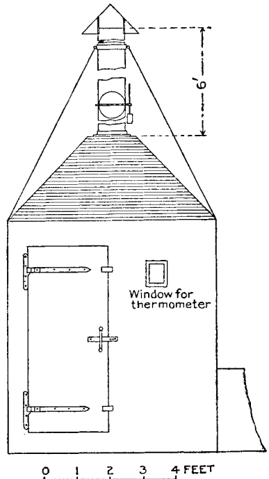
FIGURE 1.—Thaw house for frozen explosives: elevation.
