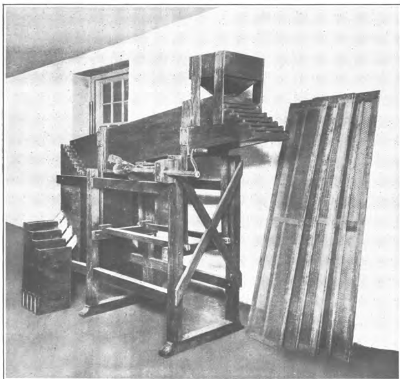
B. SCREENS FOR SEPARATING DIFFERENT-SIZED POWDER GRAINS.
