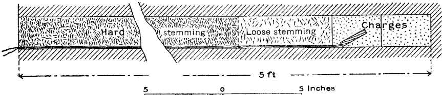
FIGURE 9.—Bore hole ready for firing.
