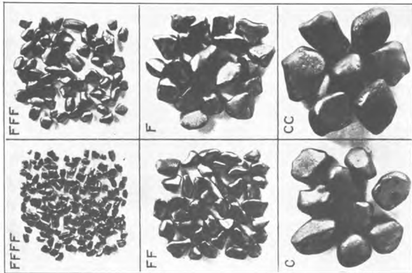
4. GRAINS OF BLACK BLASTING POWDER.
