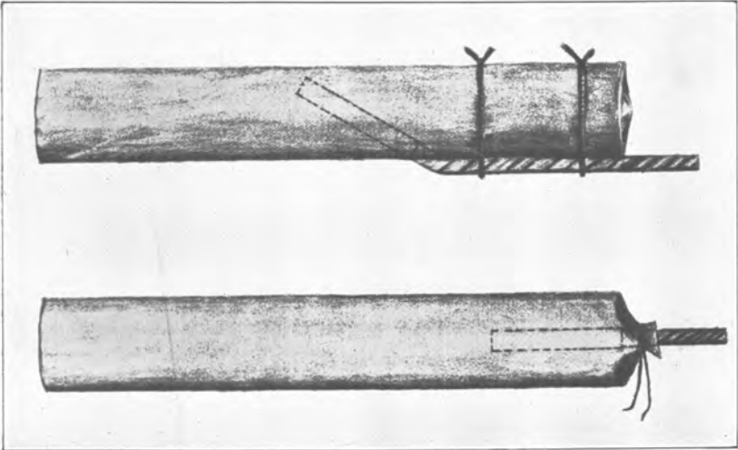
A. FUSE AND DETONATOR FITTED INTO PRIMER.
