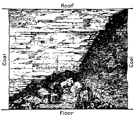
FIGURE 6.—Snubbing shot.
