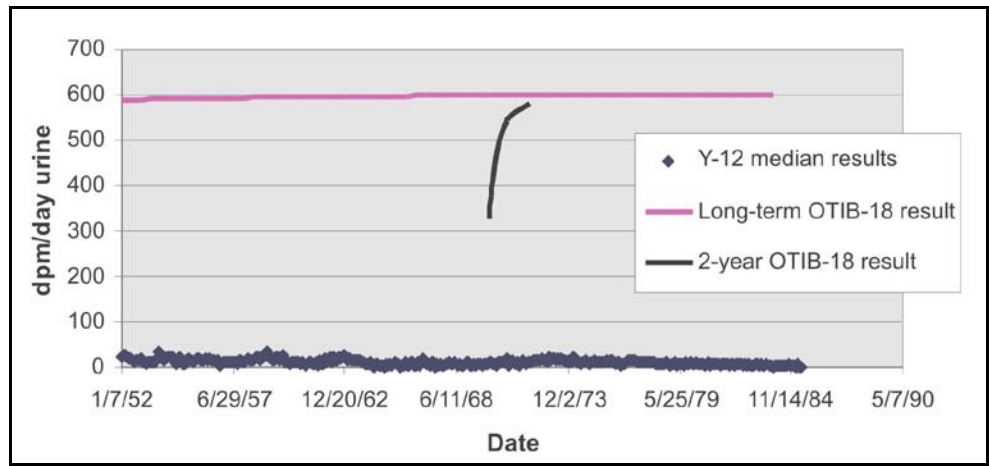
Figure B-1. Y-12 versus OTIB-18 uranium (type M).
