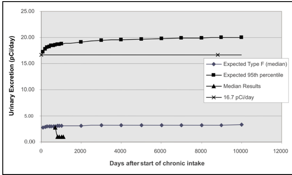
Figure B-5. Hanford Sr-90 expected urine versus actual results.
