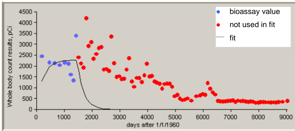
Figure C-33. 50th-percentile zinc whole-body counting data for inhalation intakes of Type S material, 1960 to 1963.
