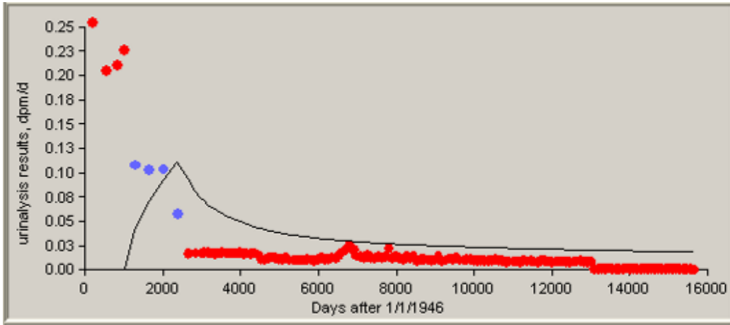
Figure C-8. 50th-percentile plutonium urinalysis data for intakes of Type M material, 1949 to 1952.
