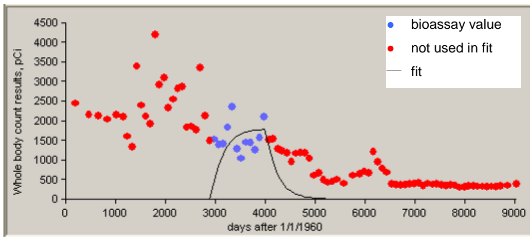
Figure C-35. 50th-percentile zinc whole-body counting data for inhalation intakes of Type S material, 1968 to 1970.
