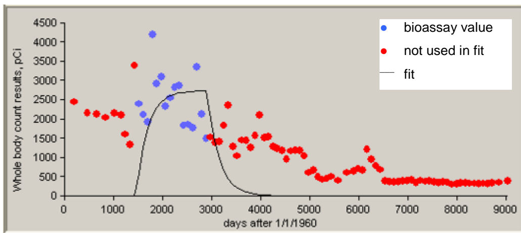
Figure C-34. 50th-percentile zinc whole-body counting data for inhalation intakes of Type S material, 1964 to 1967.
