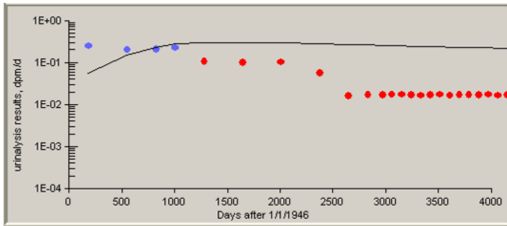
Figure C-12. 50th-percentile plutonium urinalysis data for intakes of Type S material, 1946 to 1948.
