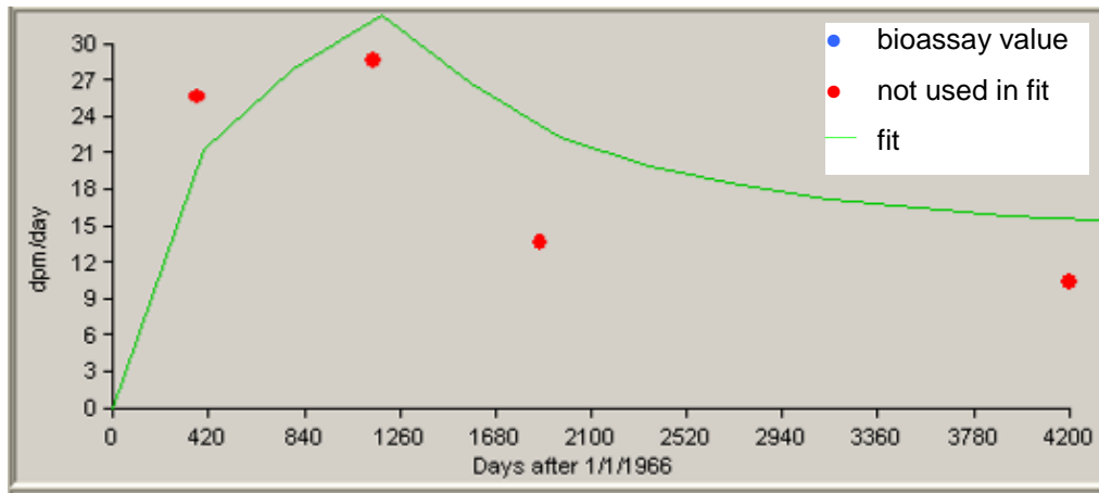
Figure C-29. Predicted 50th-percentile urinary excretion of Type M promethium from 1966 to 1979 based on two independent intakes, compared to bioassay data.
