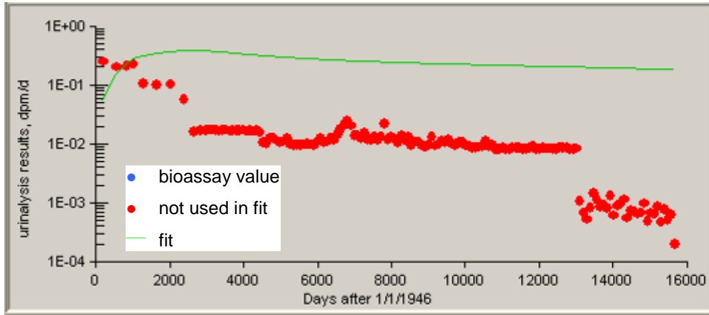
Figure C-16. Predicted 50th-percentile urinary excretion of Type S plutonium from 1946 to 1988 based on four independent intakes, compared to bioassay data.
