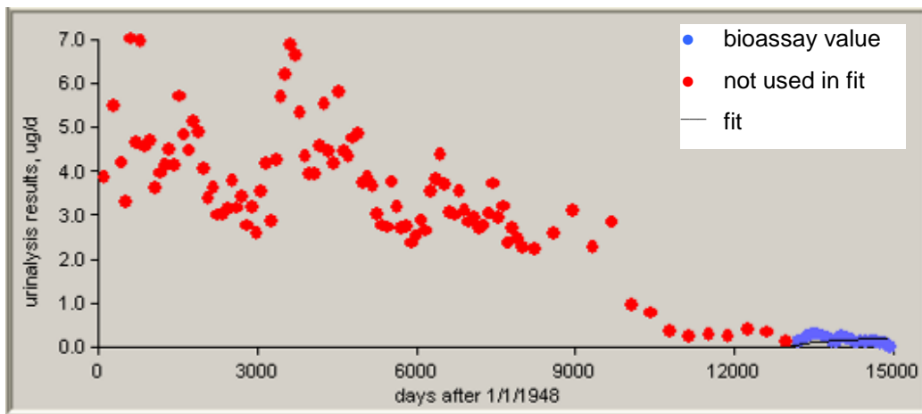
Figure C-24. 50th-percentile uranium urinalysis data for intakes of Type S material, 1984 to 1988.
