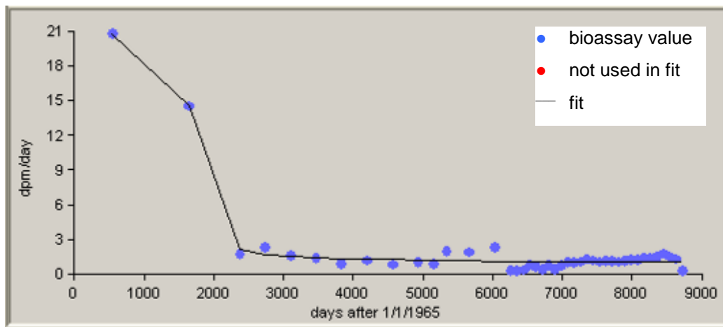
Figure C-26. 50th-percentile strontium urinalysis data for intakes of Type F material, 1965 to 1988.
