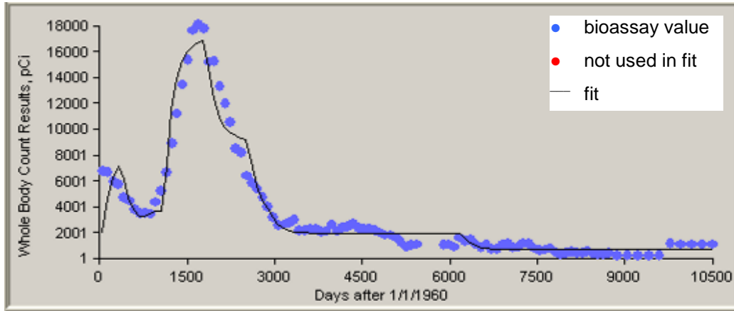
Figure C-43. 50th-percentile 137 Cs whole-body counting data for inhalation intakes of Type F material, 1960 to 1988.
