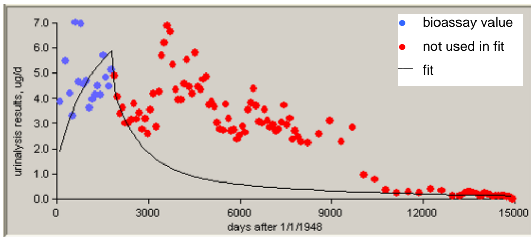
Figure C-19. 50th-percentile uranium urinalysis data for intakes of Type S material, 1948 to 1952.
