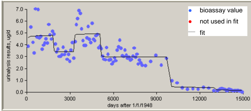
Figure C-17. 50th-percentile uranium urinalysis data for intakes of Type F material, 1948 to 1988.
