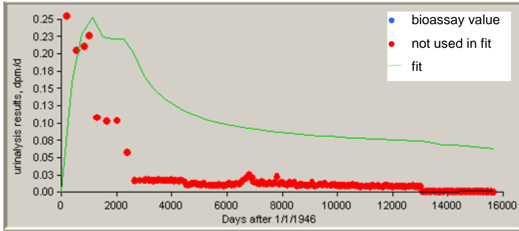
Figure C-11. Predicted 50th-percentile urinary excretion of Type M plutonium from 1946 to 1988 based on four independent intakes, compared to bioassay data.
