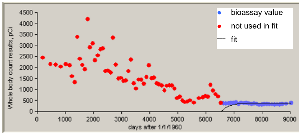
Figure C-38. 50th-percentile zinc whole-body counting data for inhalation intakes of Type S material, 1978 to 1984.
