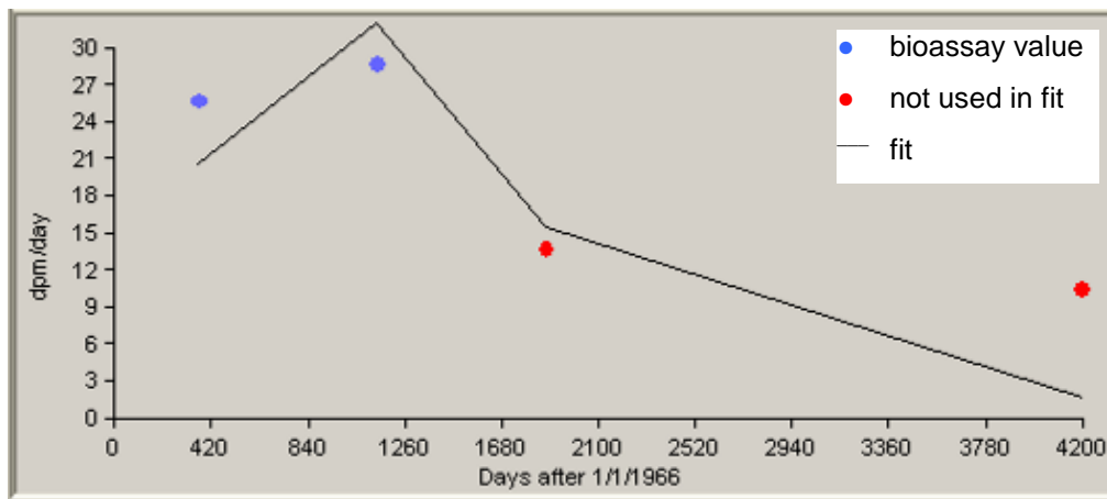
Figure C-27. 50th-percentile promethium urinalysis data for intakes of Type M material, 1966 to 1969.
