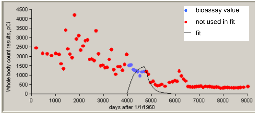
Figure C-36. 50th-percentile zinc whole-body counting data for inhalation intakes of Type S material, 1971 to 1972.
