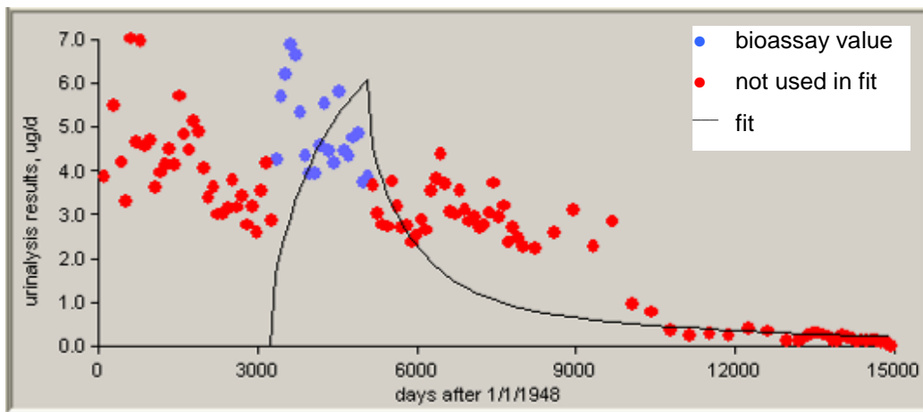
Figure C-21. 50th-percentile uranium urinalysis data for intakes of Type S material, 1957 to 1961.
