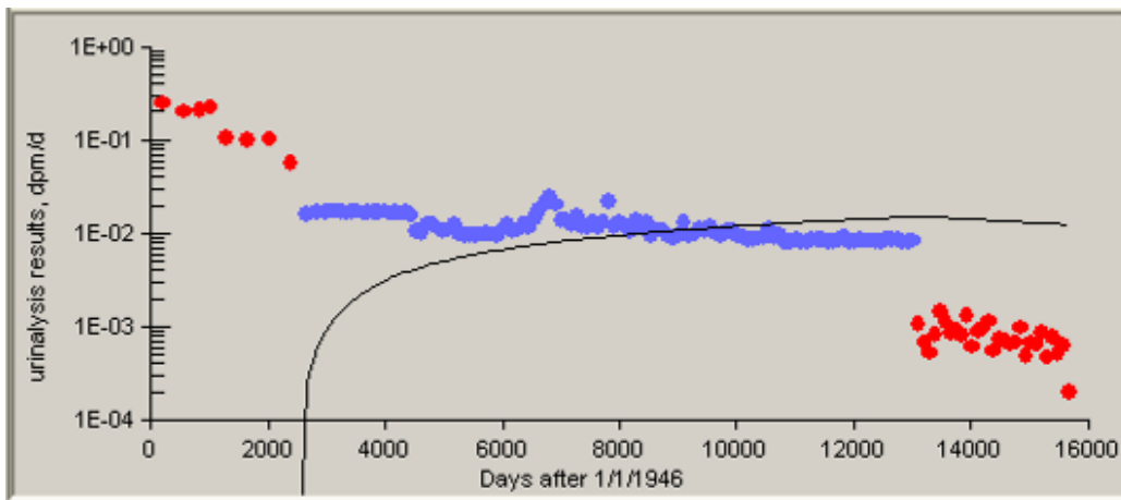
Figure C-14. 50th-percentile plutonium urinalysis data for intakes of Type S material, 1953 to 1981.
