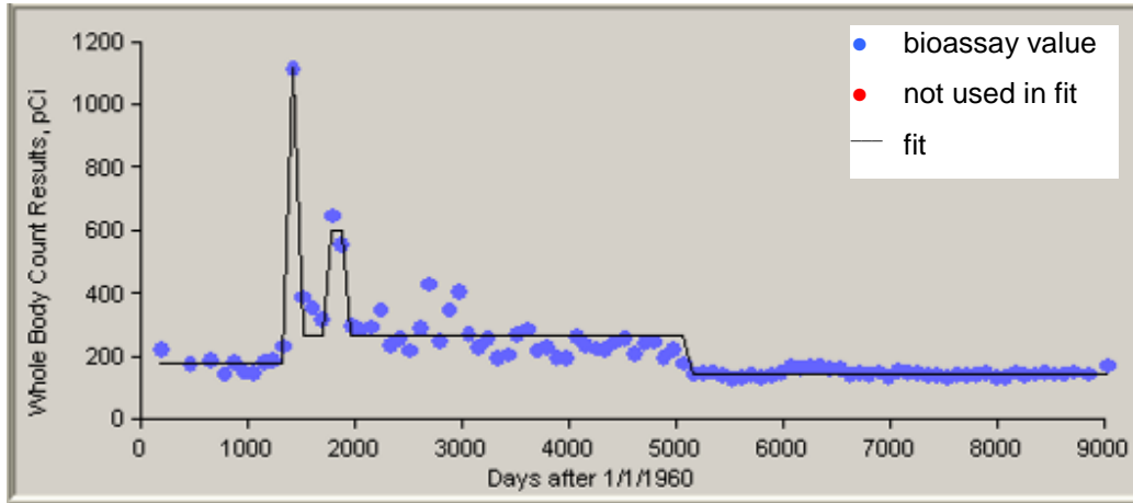
Figure C-41. 50th-percentile sodium whole-body counting data for inhalation intakes of Type F material, 1960 to 1984.
