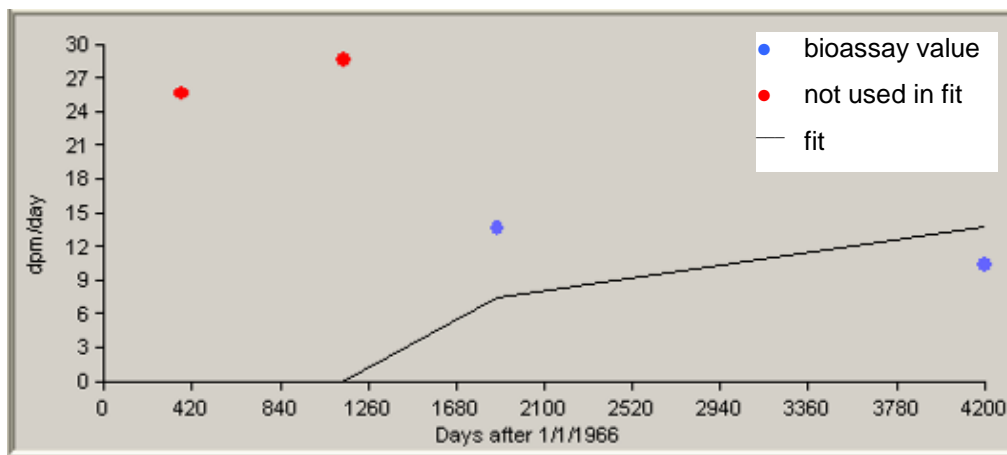
Figure C-28. 50th-percentile promethium urinalysis data for intakes of Type M material, 1970 to 1979.
