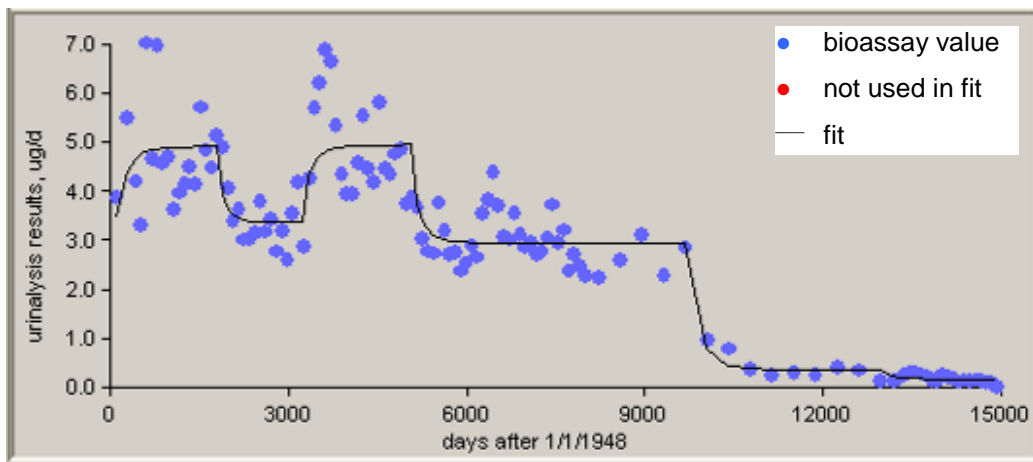
Figure C-18. 50th-percentile uranium urinalysis data for intakes of Type M material, 1948 to 1988.
