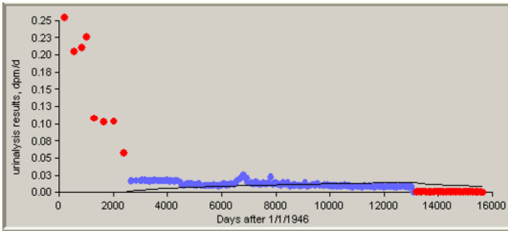
Figure C-9. 50th-percentile plutonium urinalysis data for intakes of Type M material, 1953 to 1981.
