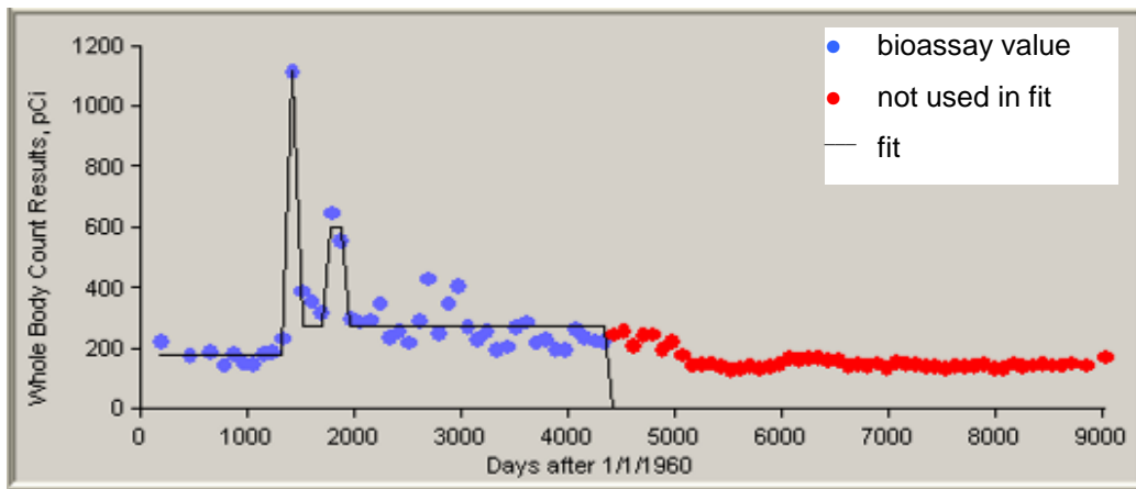
Figure C-42. 50th-percentile sodium whole-body counting data for ingestion intakes, 1960 to 1984.
