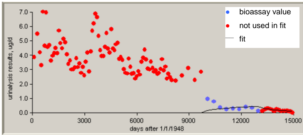
Figure C-23. 50th-percentile uranium urinalysis data for intakes of Type S material, 1975 to 1983.
