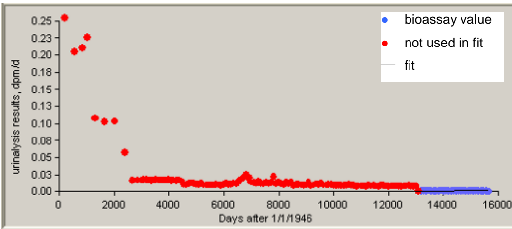
Figure C-10. 50th-percentile plutonium urinalysis data for intakes of Type M material, 1982 to 1988.
