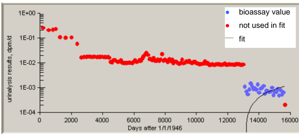
Figure C-15. 50th-percentile plutonium urinalysis data for intakes of Type S material, 1982 to 1988.
