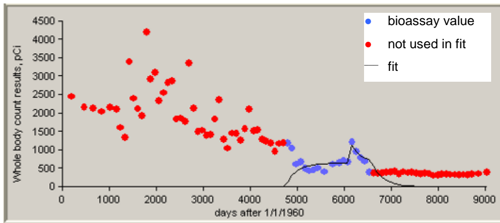
Figure C-37. 50th-percentile zinc whole-body counting data for inhalation intakes of Type S material, 1973 to 1977.
