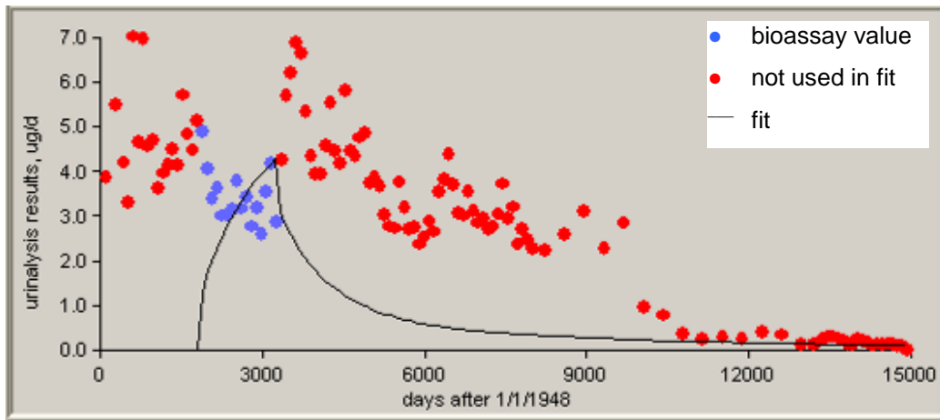
Figure C-20. 50th-percentile uranium urinalysis data for intakes of Type S material, 1953 to 1956.
