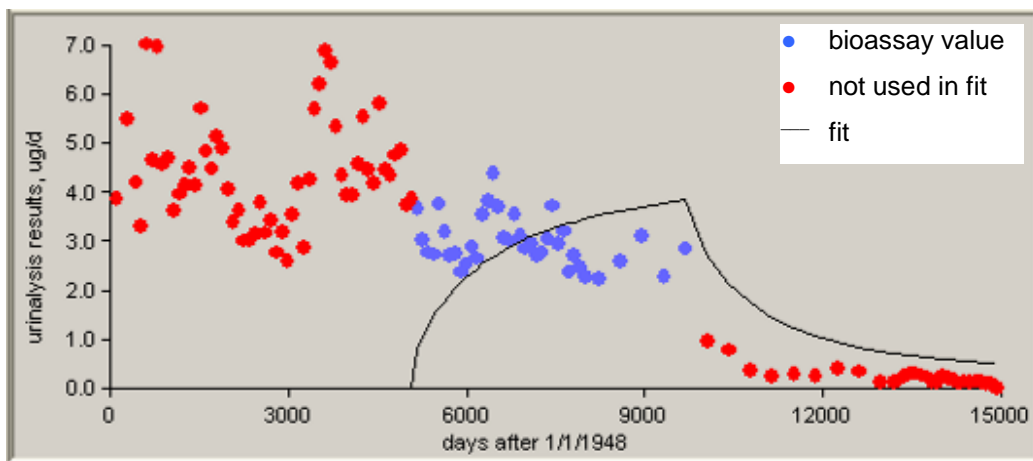
Figure C-22. 50th-percentile uranium urinalysis data for intakes of Type S material, 1962 to 1974.
