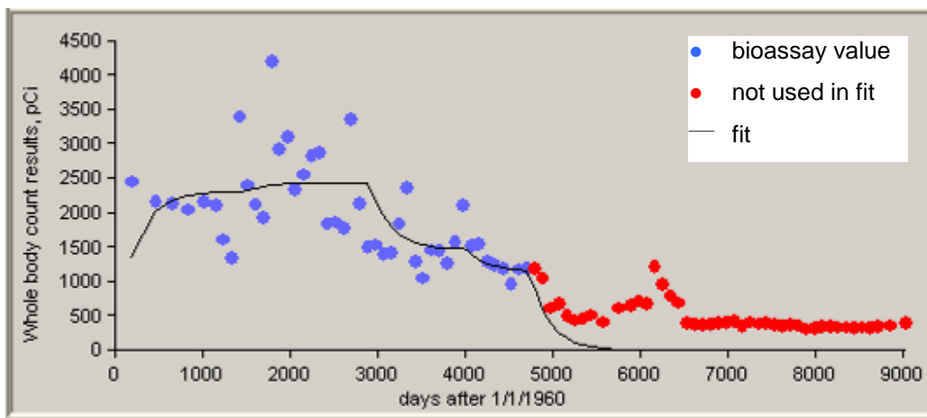
Figure C-40. 50th-percentile zinc whole-body counting data for ingestion intakes, 1960 to 1984.
