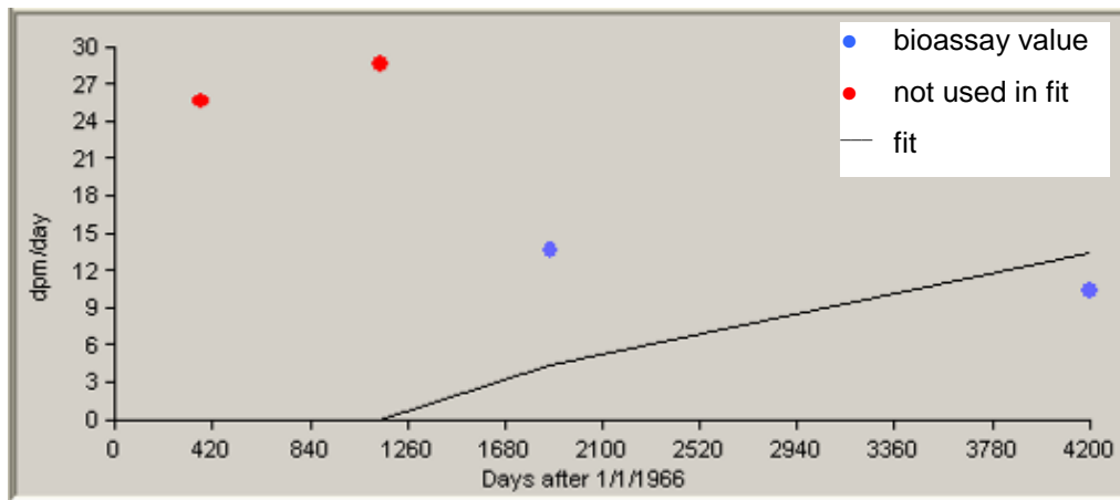
Figure C-31. 50th-percentile promethium urinalysis data for intakes of Type S material, 1970 to 1979.
