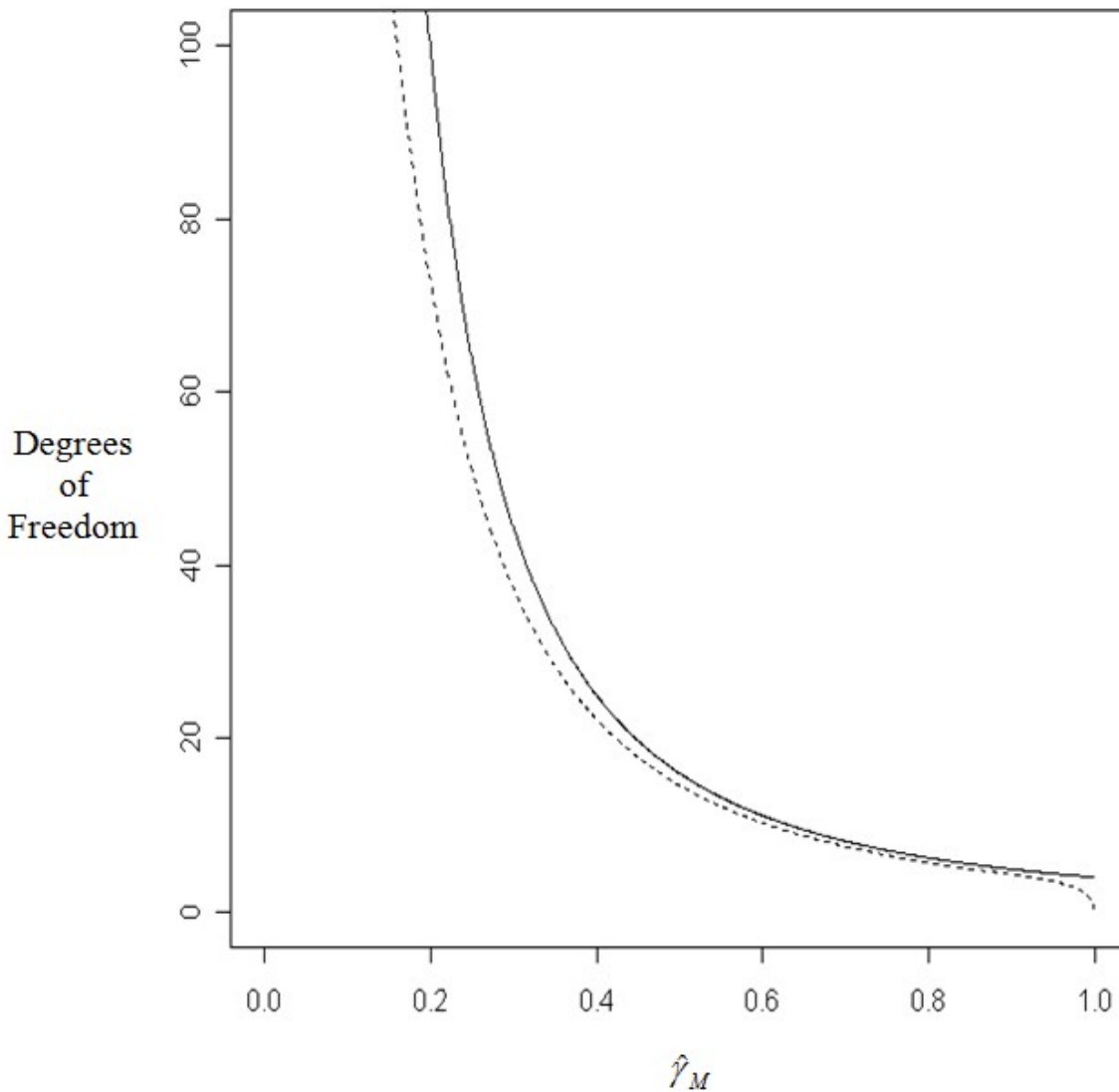
Figure 6 Rubin-Schenker (solid curve) and Barnard-Rubin (dashed curve) degrees of freedom as a function of the approximate fraction of missing information \hat{\gamma}_M , when the complete-data degrees of freedom are equal to 339
