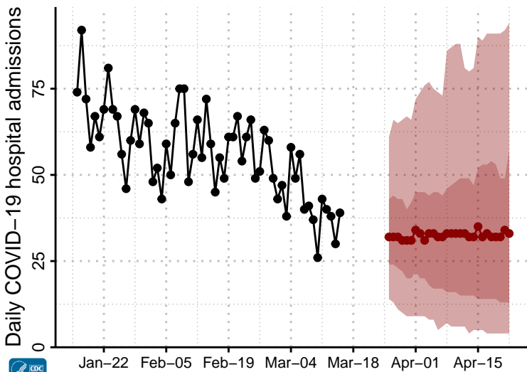
Ensemble forecast
