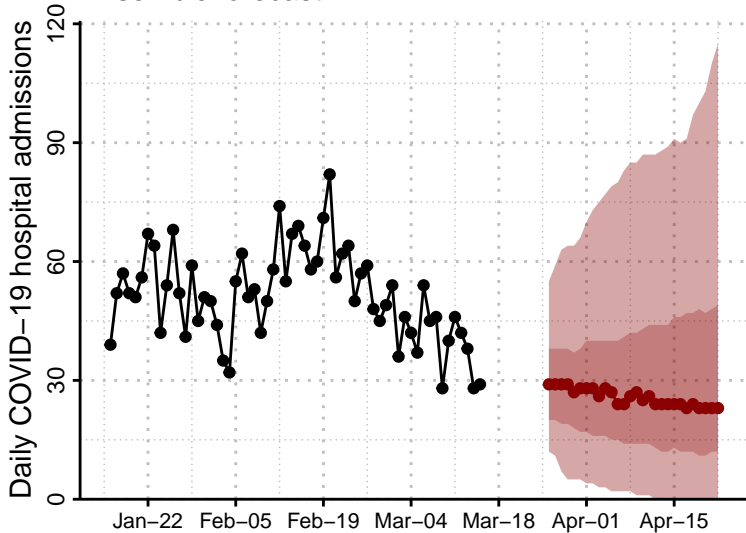
Ensemble forecast
