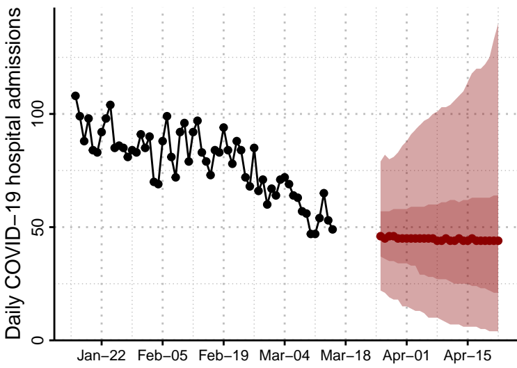
Ensemble forecast
