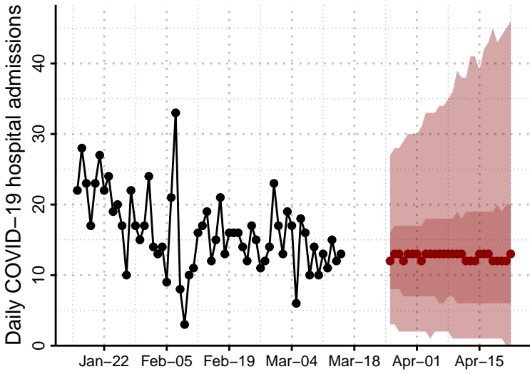
Ensemble forecast
