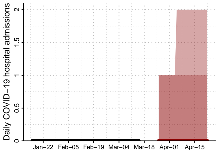
Ensemble forecast
