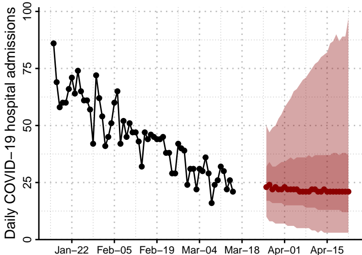
Ensemble forecast
