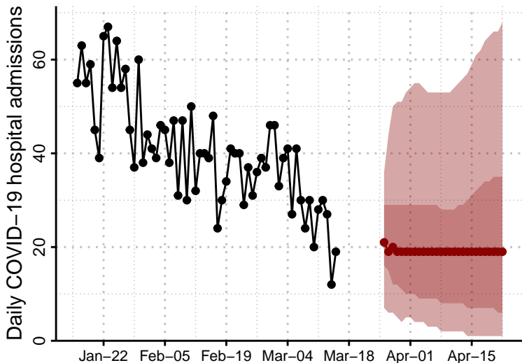
Ensemble forecast
