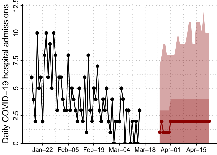
Ensemble forecast
