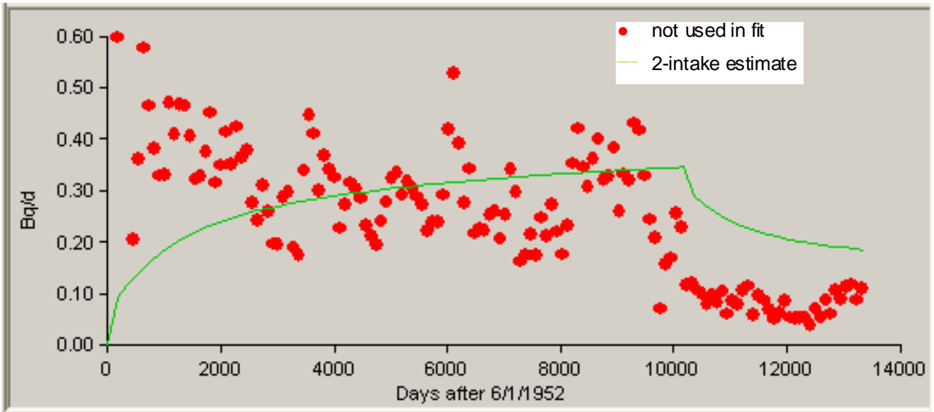
Figure A-7. Predicted 50th-percentile urinary excretion of Type S uranium from 1952 to 1988 based on two independent intakes, compared to bioassay data.
