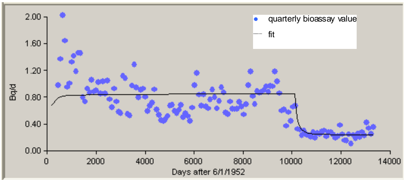
Figure A-4. 84th-percentile uranium urinalysis data used to estimate intakes of Type M uranium occurring 6/1/52 to 12/31/88.
