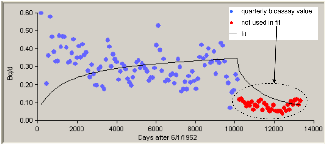
Figure A-5. 50th-percentile uranium urinalysis data used to estimate intakes of Type S uranium occurring 6/1/52 to 3/31/80.
