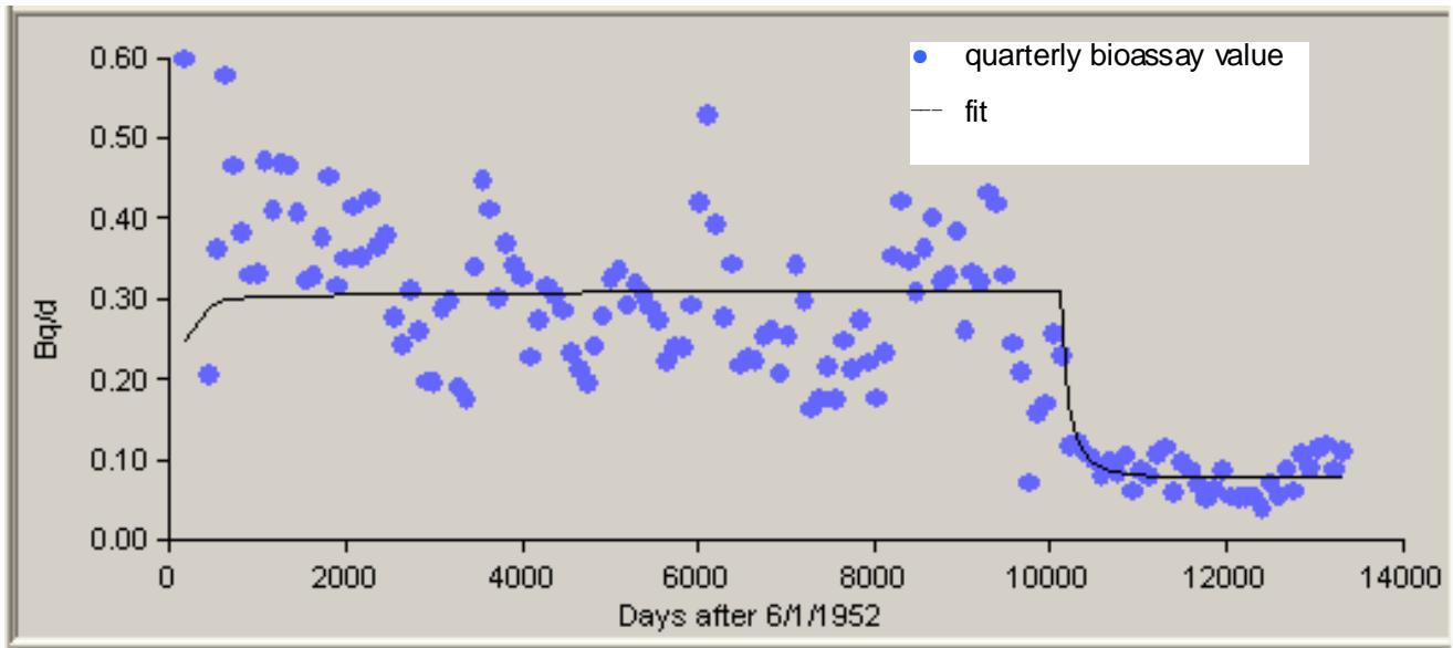
Figure A-3. 50th-percentile uranium urinalysis data used to estimate intakes of Type M uranium occurring 6/1/52 to 12/31/88.
