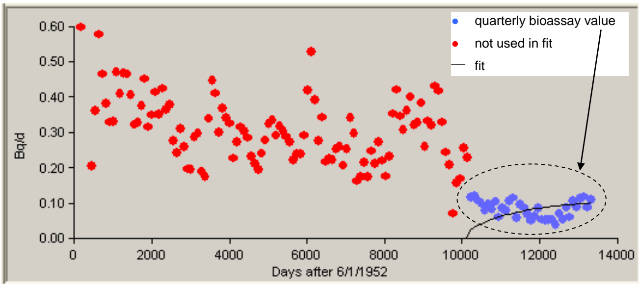
Figure A-6. 50th-percentile uranium urinalysis data used to estimate intakes of Type S uranium occurring 4/1/80 to 12/31/88.
