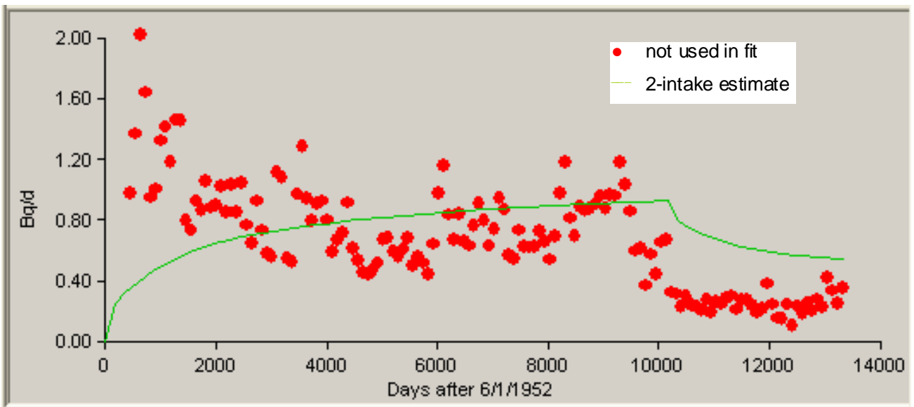
Figure A-8. Predicted 84th-percentile urinary excretion of Type S uranium from 1952 to 1988 based on two independent intakes, compared to bioassay data.
