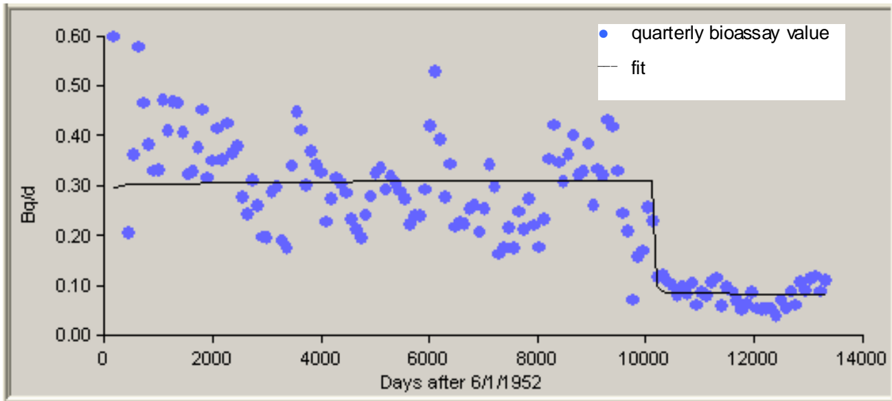
Figure A-1. 50th-percentile uranium urinalysis data used to estimate intakes of Type F uranium occurring 6/1/52 to 12/31/88.
