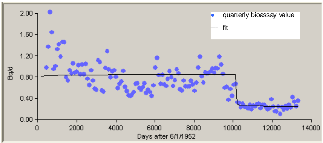
Figure A-2. 84th-percentile uranium urinalysis data used to estimate intakes of Type F uranium occurring 6/1/52 to 12/31/88.
