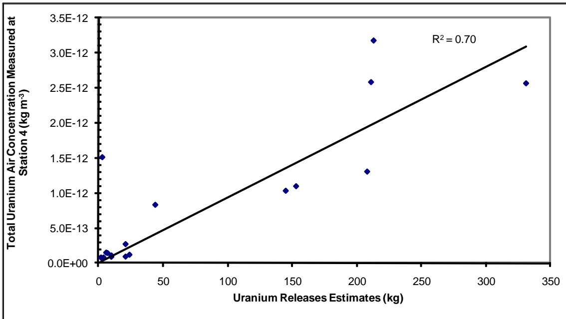
Figure 4.2.5-2. Plot of annual total uranium air concentration measured at Station 4 versus estimated uranium releases. Correlation coefficient R^2 = 0.70 .
