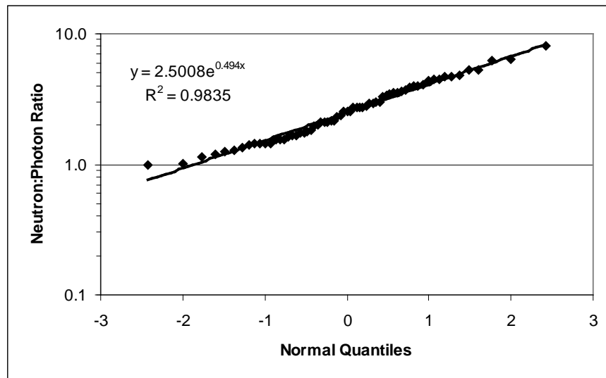
Figure 6-21. Normal probability plot for Group 3 neutron-to-photon dose ratios [41].
