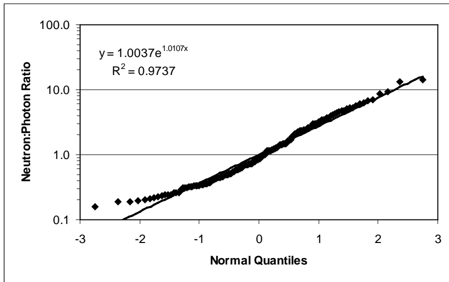
Figure 6-27. Normal probability plot for Group 9 neutron-to-photon dose ratios [47].
