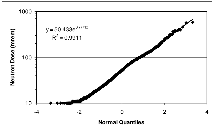
Figure 6-18. Normal probability plot for Group 2 neutron doses [38].
