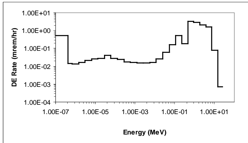
Figure 6-5. Neutron energy spectrum in the RADCAL beta/X-ray irradiation room with a bare ^{252}\text{Cf} source exposed in the adjacent neutron irradiation room [11].
