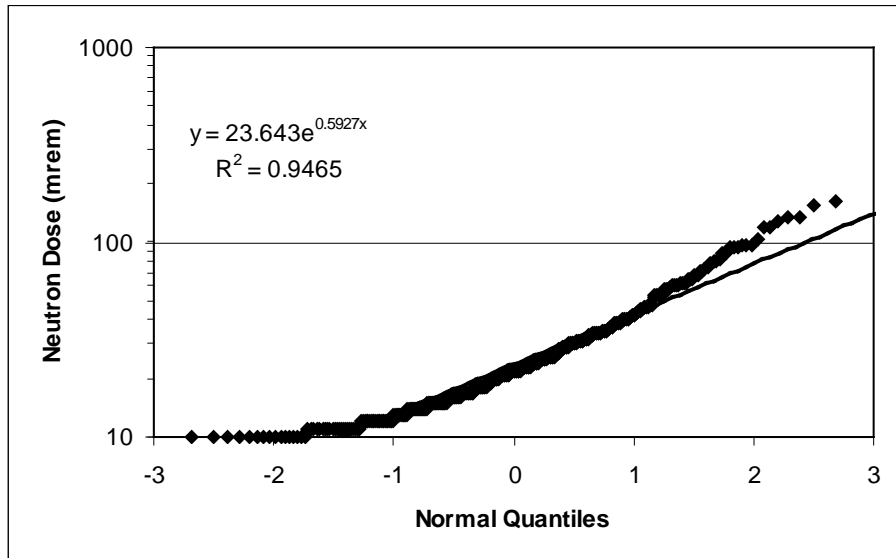
Figure 6-28. Normal probability plot for Group 9 neutron doses [48].
