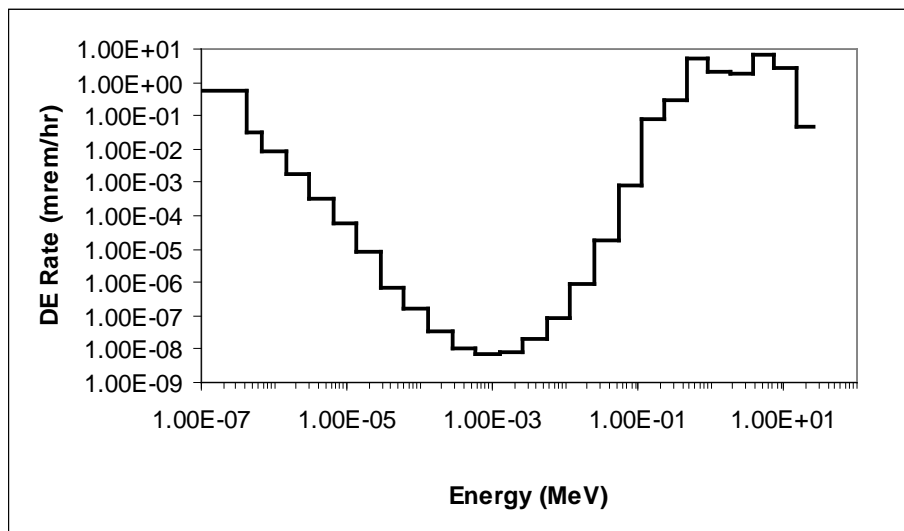
Figure 6-2. Neutron spectrum measured by PNL for ^{238}\text{Pu}:\text{Be} and ^{252}\text{Cf} sources in a water-shielded drum in Building 3038 [5].
