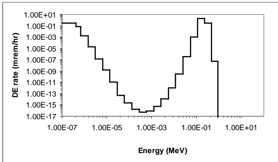
Figure 6-12. Neutron energy spectrum for the REDC TDF containing 12 mg ^{252}\text{Cf} [26].
