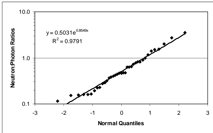
Figure 6-32. Normal probability plot for Group 13 neutron-to-photon dose ratios [52].
