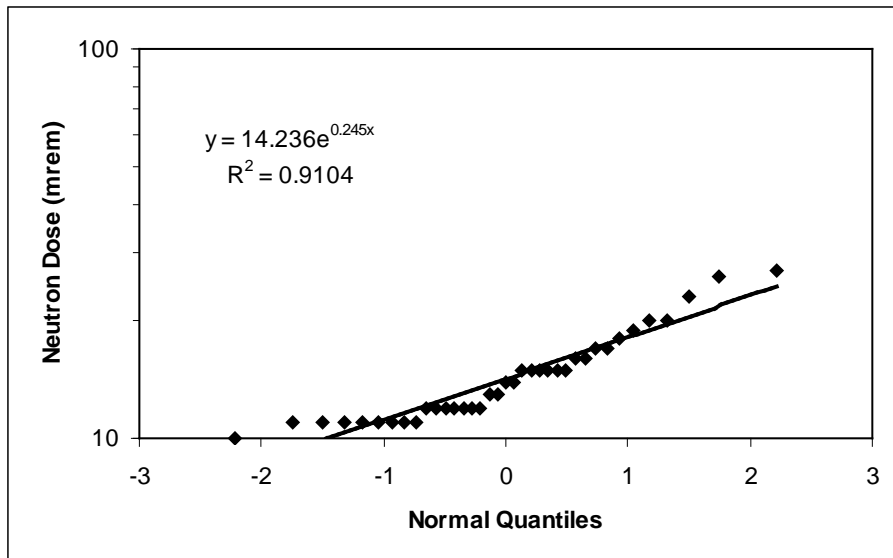
Figure 6-26. Normal probability plot for Group 7 neutron doses [46].
