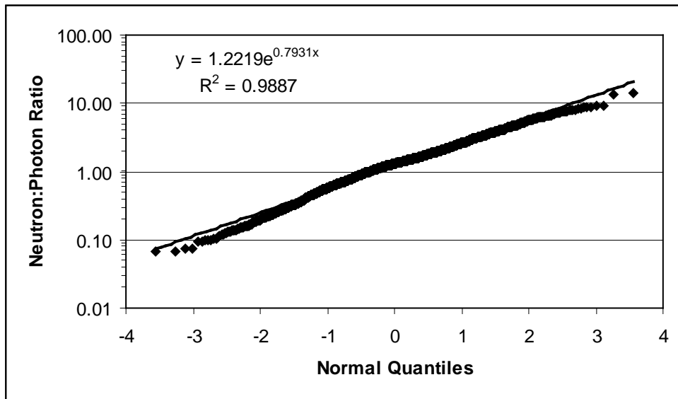
Figure 6-36. Normal probability plot for neutron-to-photon dose ratios derived from ORNL personnel neutron monitoring records for 1990 – 2004 [56].
