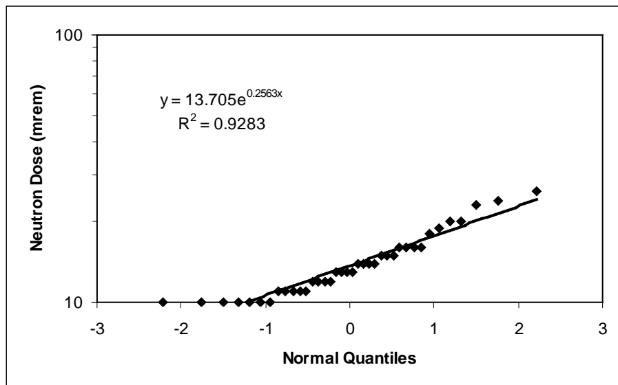
Figure 6-29. Normal probability plot for Group 11 neutron doses [49].
