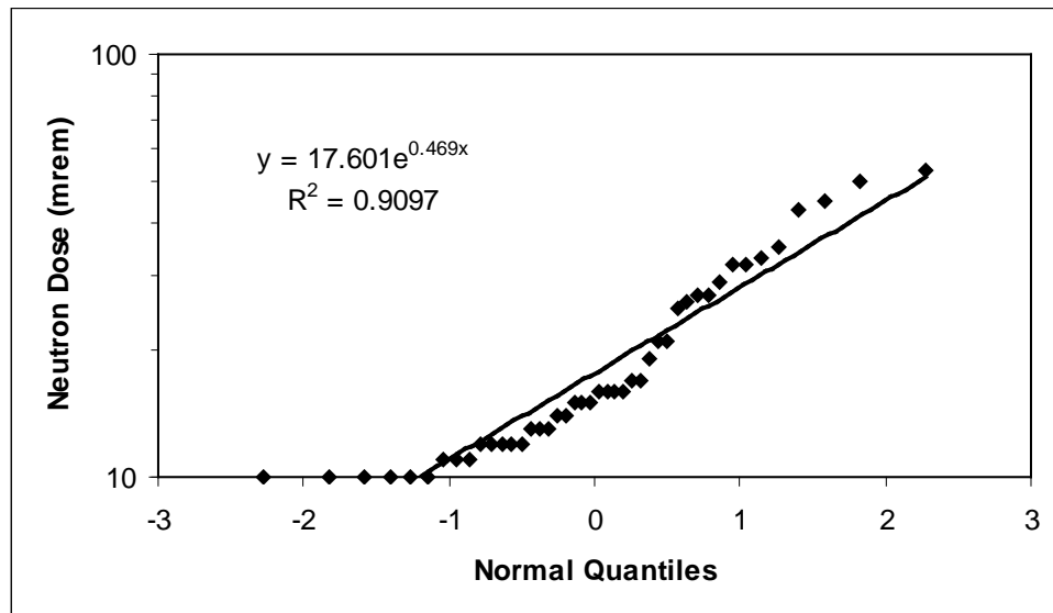
Figure 6-33. Normal probability plot for Group 13 neutron doses [53].
