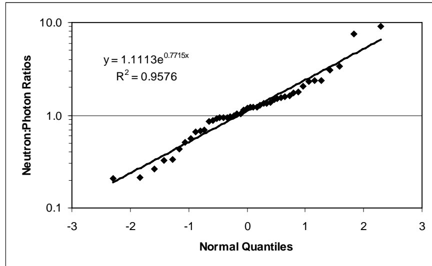
Figure 6-34. Normal probability plot for Group 14 neutron-to-photon dose ratios [54].
