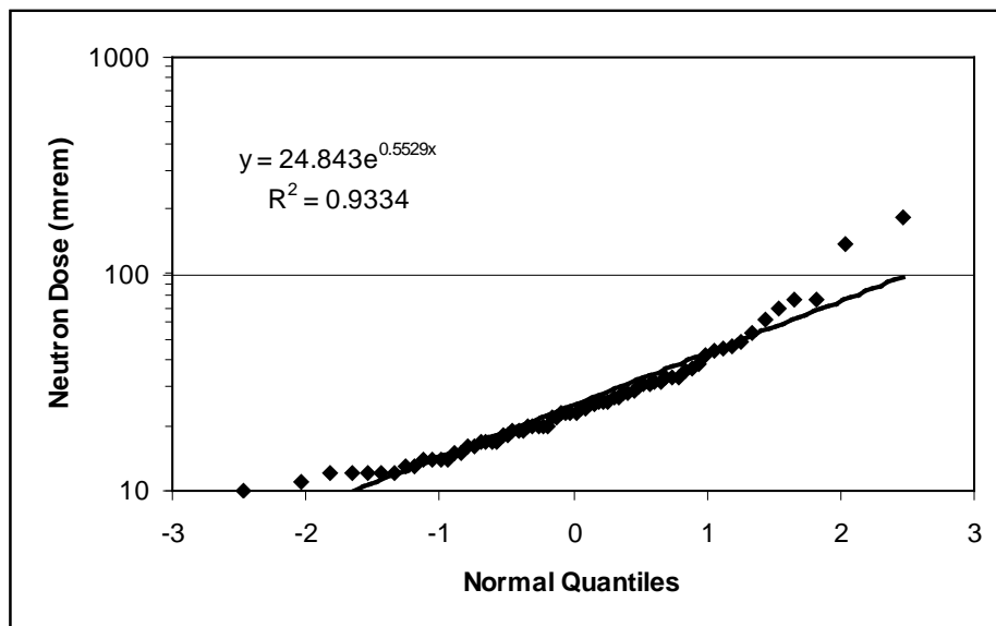
Figure 6-35. Normal probability plot for Group 14 neutron doses [55].
