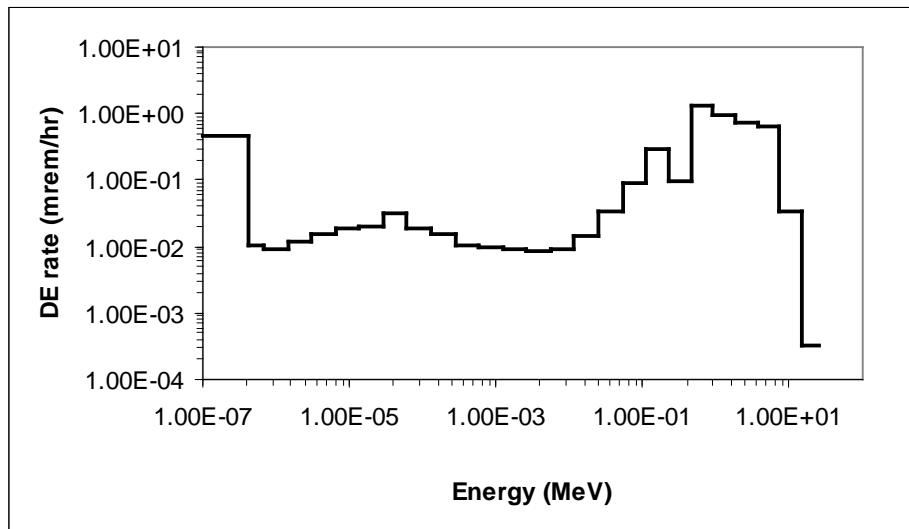
Figure 6-13. Neutron energy spectrum for a waste cask in the REDC Limited Access Area [28].
