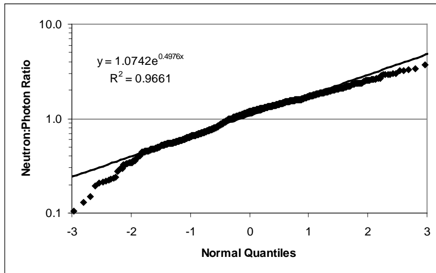
Figure 6-19. Normal probability plot for Group 4 neutron-to-photon dose ratios [39].
