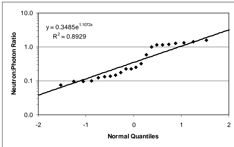
Figure 6-25. Normal probability plot for Group 7 neutron-to-photon dose ratios [45].
