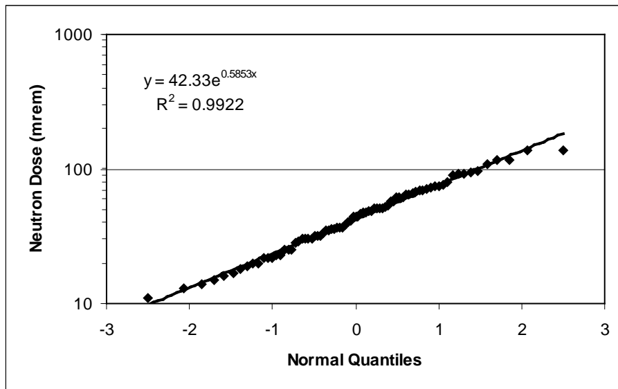
Figure 6-22. Normal probability plot for Group 3 neutron doses [42].
