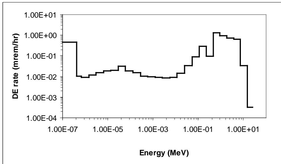
Figure 6-14. Neutron energy spectrum for contamination on the walls of the REDC WTA transfer tunnel [30].
