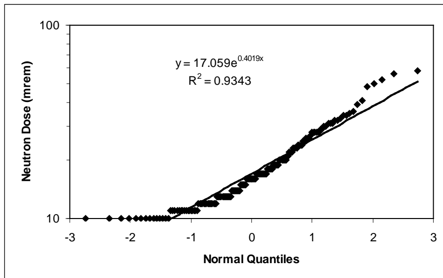
Figure 6-31. Normal probability plot for Group 21 neutron doses [51].
