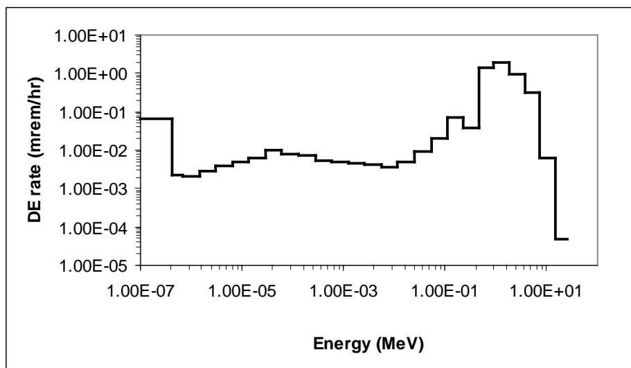
Figure 6-10. Neutron energy spectrum measured by PNL in REDC Room 111 at 37 cm from a glovebox containing ^{252}\text{Cf} [22].
