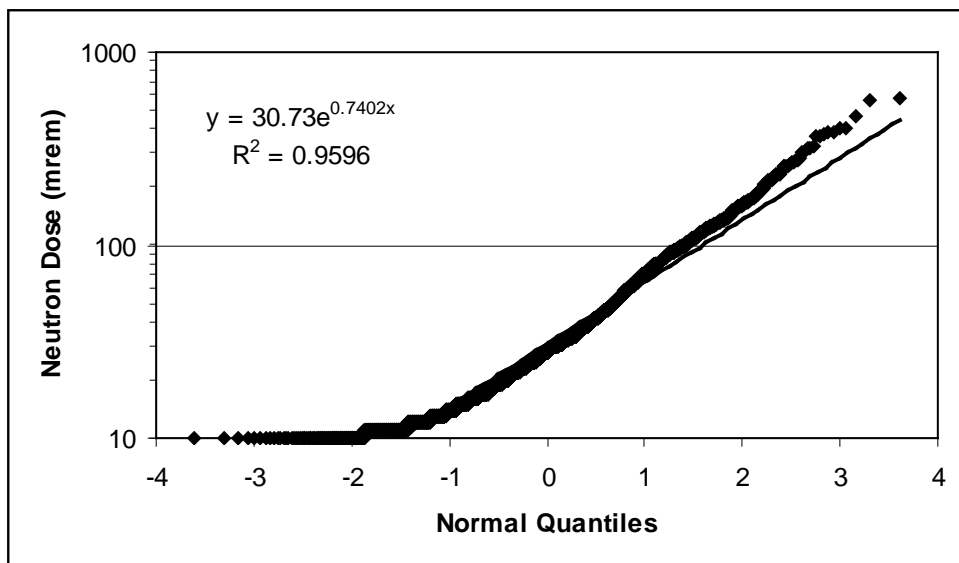
Figure 6-37. Normal probability plot for neutron doses \geq 10 mrem for ORNL workers in the period from 1990 – 2004 [57].
