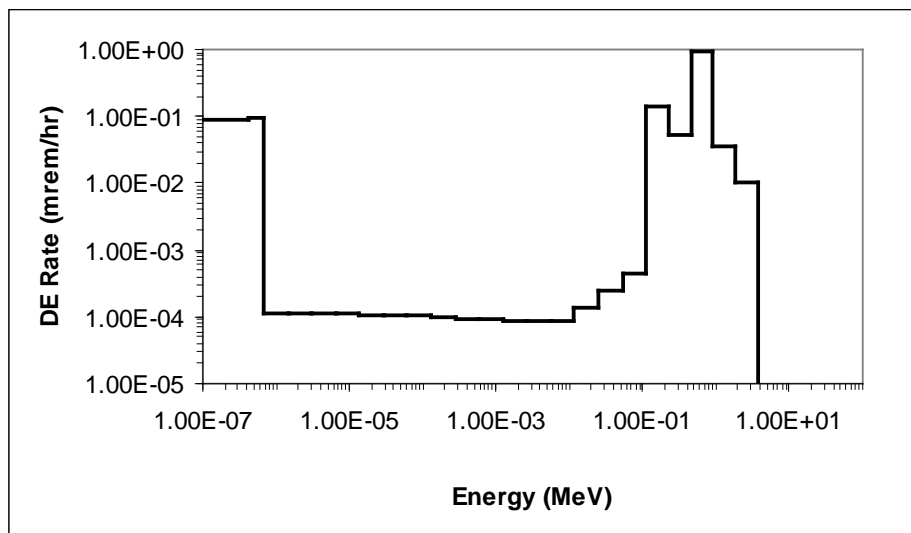
Figure 6-4. Neutron energy spectrum at the west entrance to the ORELA room [9].
