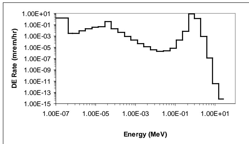
Figure 6-6. Neutron energy spectrum in the RADCAL beta/X-ray irradiation room with a moderated ^{252}\text{Cf} source exposed in the adjacent neutron irradiation room [12].
