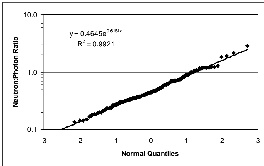
Figure 6-30. Normal probability plot for Group 21 neutron-to-photon dose ratios [50].
