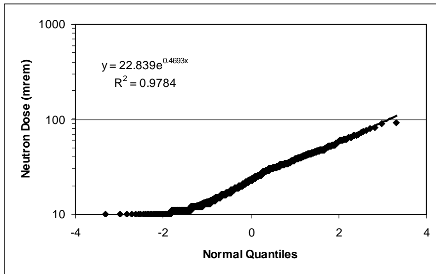
Figure 6-20. Normal probability plot for Group 4 neutron doses [40].
