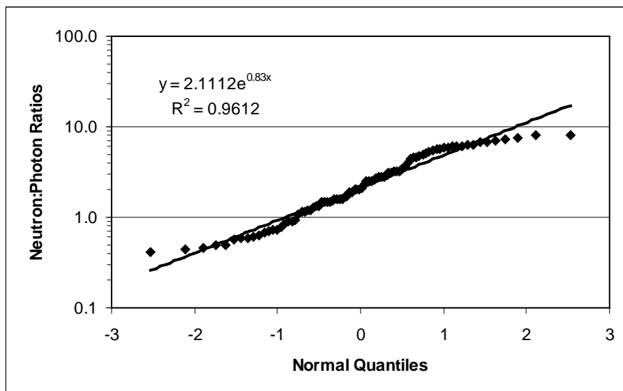
Figure 6-23. Normal probability plot for Group 17 neutron-to-photon dose ratios [43].
