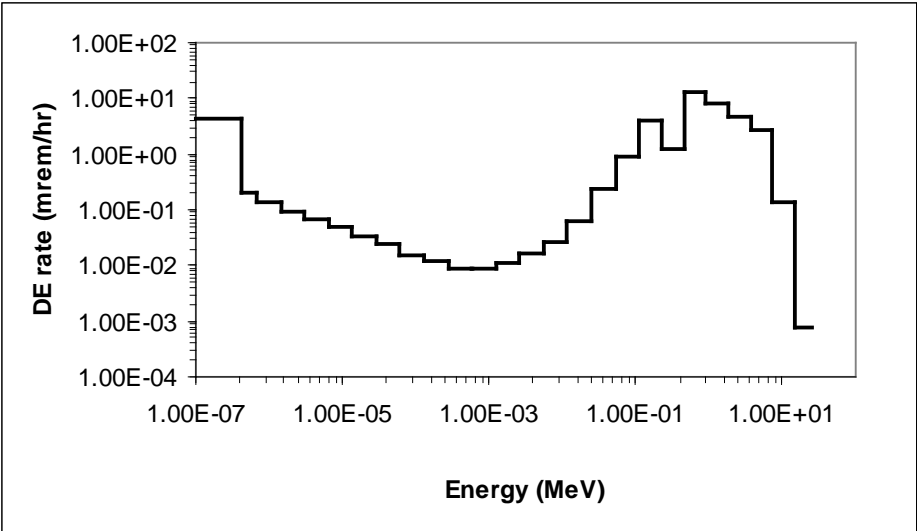
Figure 6-15. Neutron energy spectrum for waste casks in the SWSA 5 TRU storage bunker [33].
