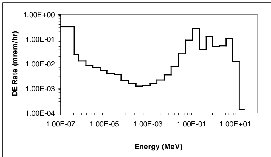
Figure 6-7. Neutron energy spectrum in the hallway outside the RADCAL neutron irradiation room with a moderated ^{252}\text{Cf} source exposed [15].
