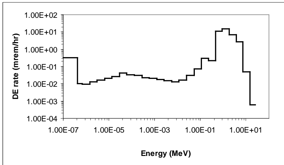
Figure 6-11. Neutron energy spectrum in REDC Room 211 at 32 cm from the end of a glovebox bank [24].
