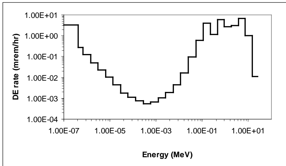
Figure 6-16. Neutron energy spectrum at a wall shared between two adjacent TRU storage bunkers at SWSA 5 [35].
