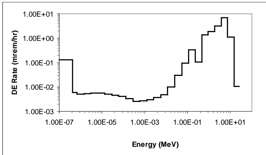
Figure 6-9. Neutron energy spectrum in RASCAL Room 102 at 130 cm from the ^{238}\text{Pu}:\text{Be} neutron calibration source [20].
