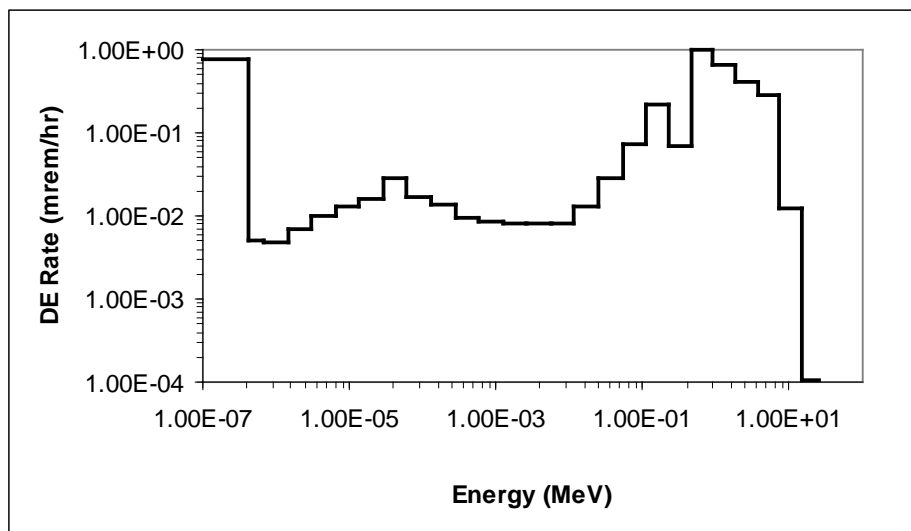
Figure 6-8. Neutron energy spectrum in the RADCAL equipment room with a moderated ^{252}\text{Cf} source exposed in the adjacent neutron irradiation room [17].
