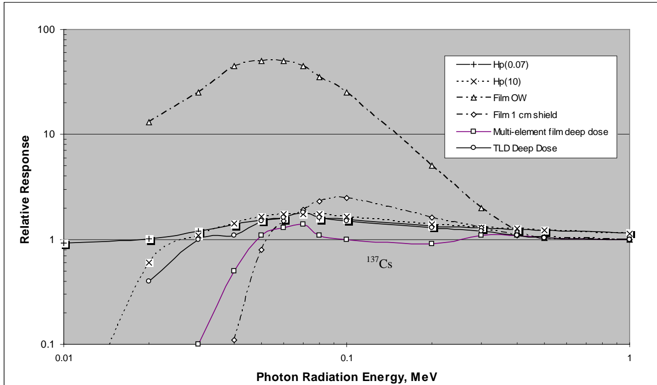
Figure 6-1. Typical two-element, multi-element film and TL dosimeter photon response compared to Hp(0.07) and Hp(10).
