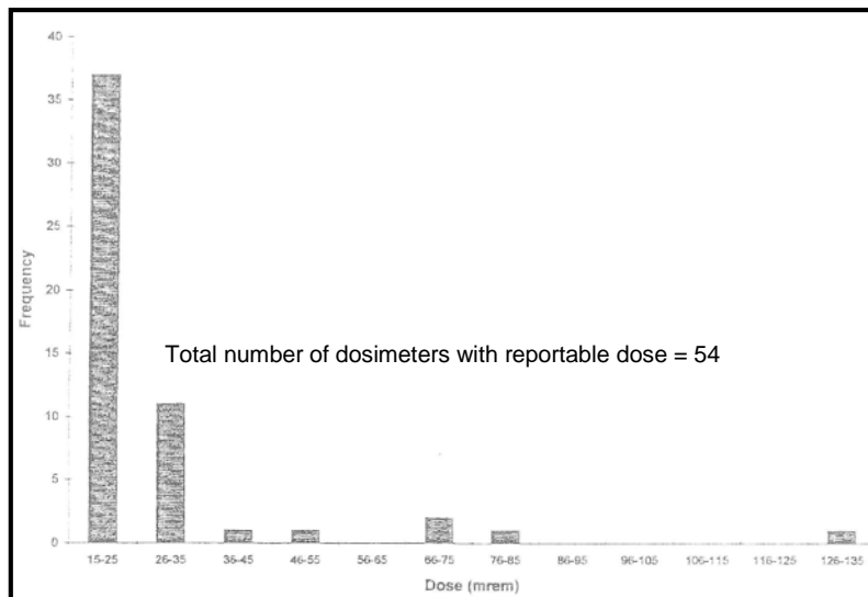
Figure 6-14. Distribution of reportable neutron dose for the first 9 months of 1995. Of 1,461 dosimeters, 1,407 were below the 15-mrem reporting level (Gesell et al. 1996).
