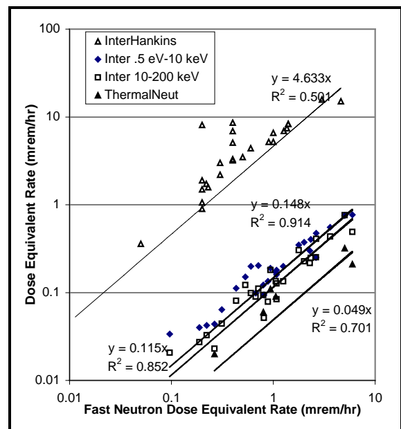
Figure 6-18. MTR neutron field components (ORAUT 2006a).
