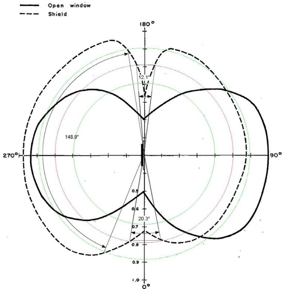
Figure 7-4: Directional Response of Savannah River Plant Film Badge (Gamma) (Wright, 1958)
