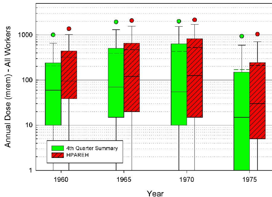
Figure 6-2: Comparison of Annual Dose Distributions for Construction Trades Workers in HPAREH and the 4 th Quarter Reports
