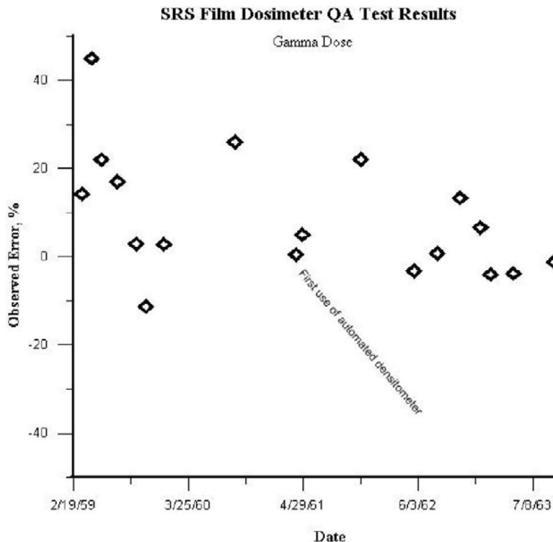
Figure 7-5: SRS Film Dosimeter Audit Results for March 1959 through September 1963
