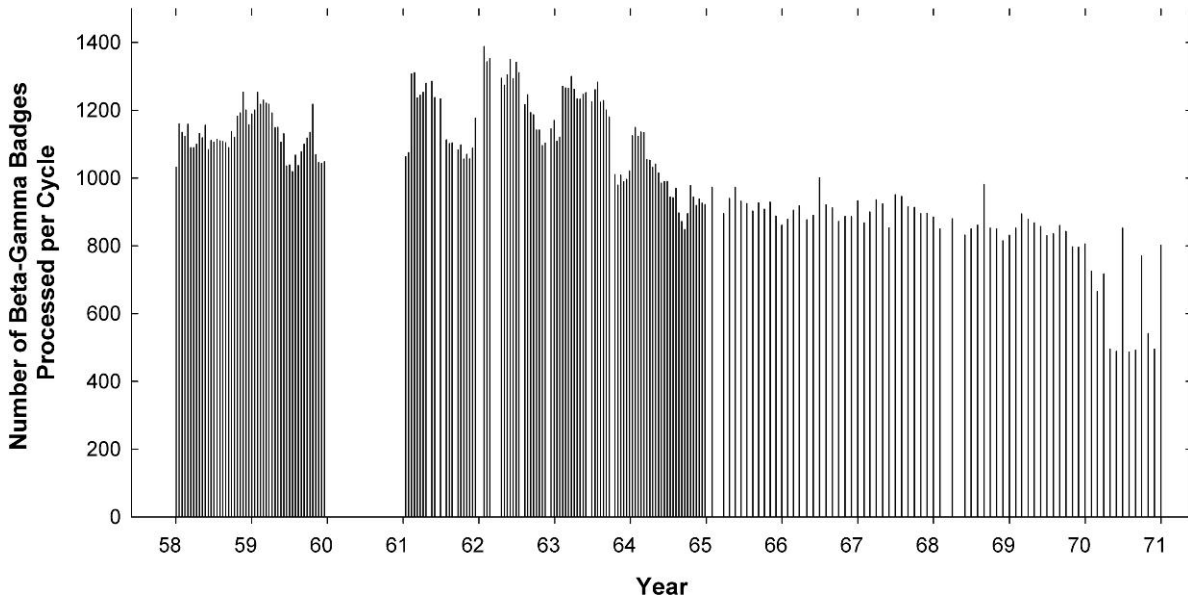
Figure 7-2: Number of Beta/Gamma (Photon) Film Dosimeter Badges Processed per Cycle for the 200-F Area.
