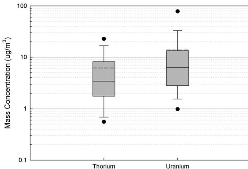
Figure 7-1: Comparison of SRS Thorium and Uranium Air Sample Data
