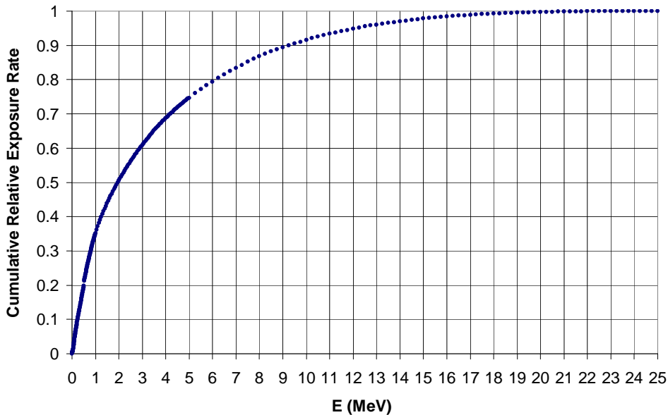
Figure 4. Cumulative Exposure Rate vs. Photon Energy in Restroom (location #6 in Figure 2)
