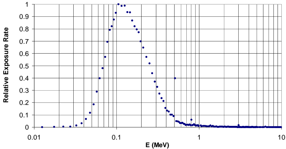
Figure 3. Exposure Rate vs. Photon Energy in Control Room (location #1 in Figure 2)
