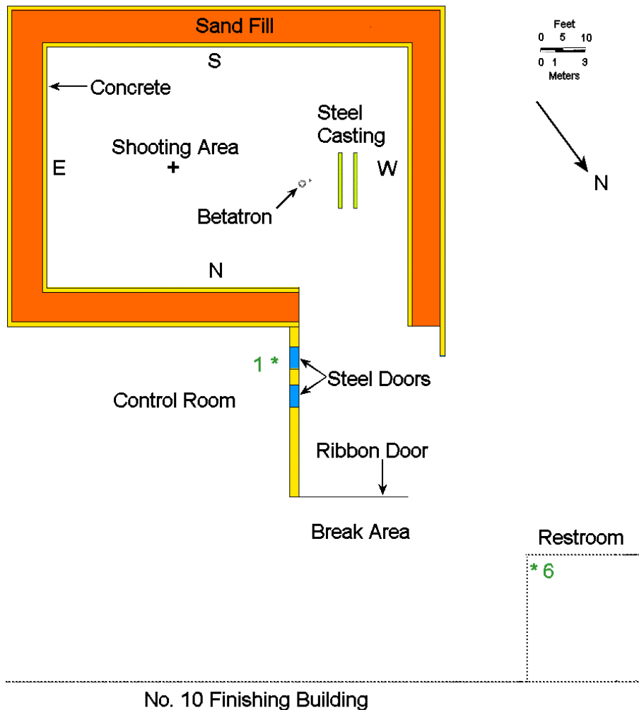
Figure 2. MCNP Model of New Betatron Building, Showing Locations of Exposure Assessments
