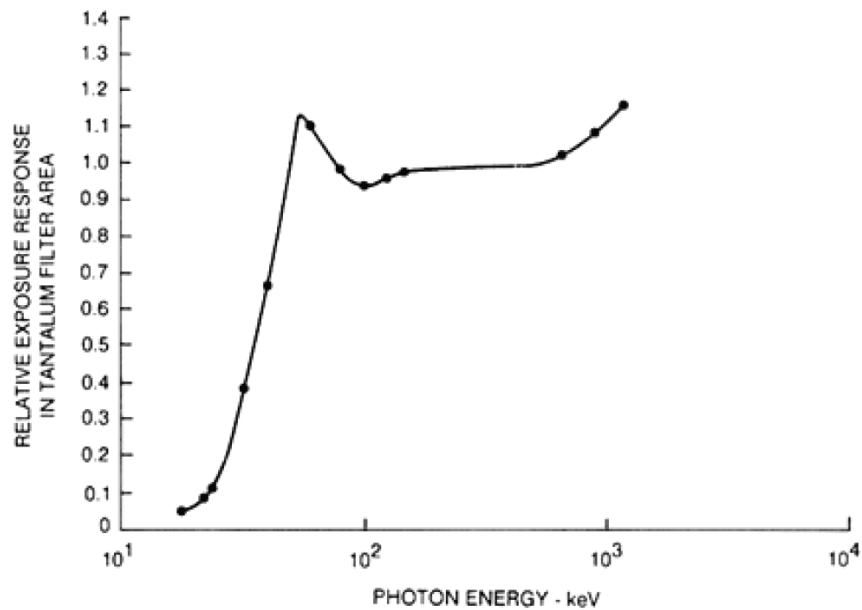
Figure 1. Film Response with 0.020-inch Tantalum Filter (adapted from Brady and Iverson, 1968) (Lalos 1989, Figure 2-5)
