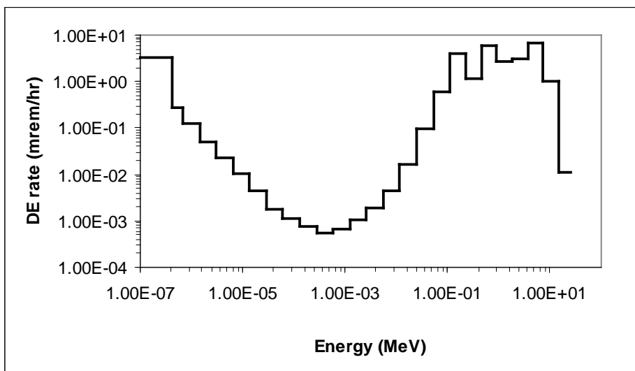
Figure 6-16. Neutron energy spectrum at a wall shared between two adjacent TRU storage bunkers at SWSA 5.
