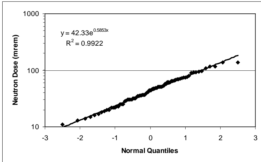
Figure 6-22. Normal probability plot for Group 3 neutron doses.
