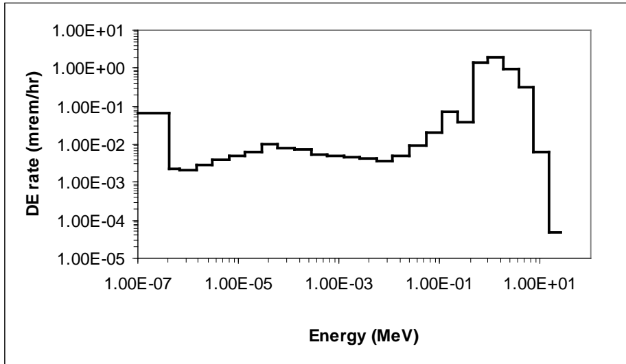
Figure 6-10. Neutron energy spectrum measured by PNL in REDC Room 111 at 37 cm from a glovebox containing 252 Cf.
