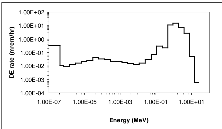
Figure 6-11. Neutron energy spectrum in REDC Room 211 at 32 cm from the end of a glovebox bank.
