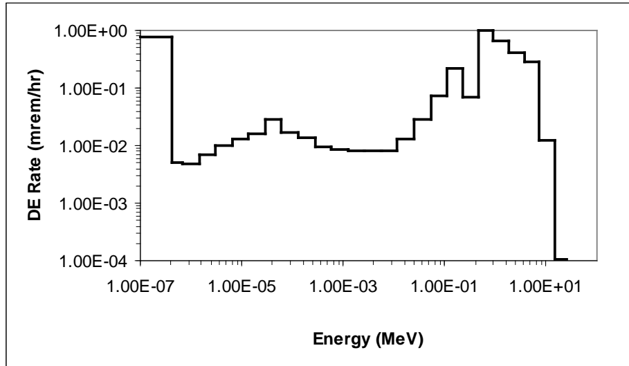
Figure 6-8. Neutron energy spectrum in the RADCAL equipment room with a moderated ^{252}\text{Cf} source exposed in the adjacent neutron irradiation room.
