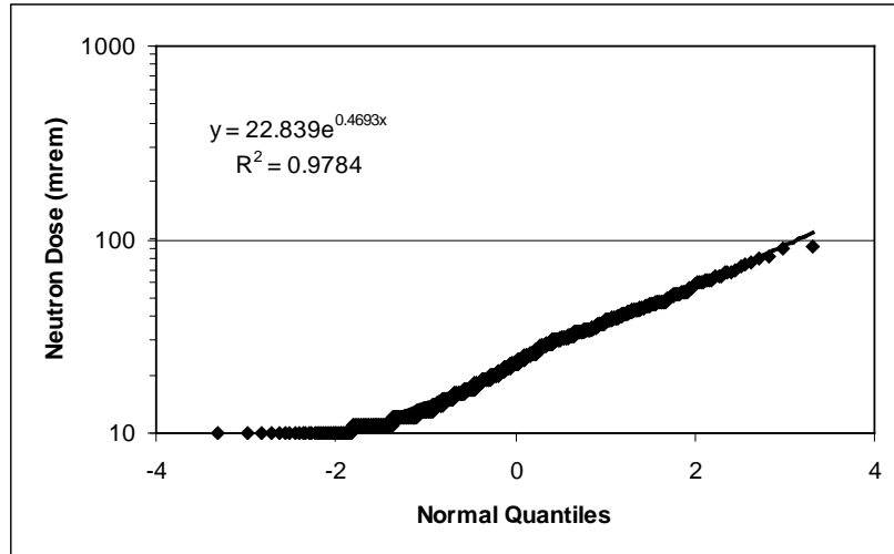
Figure 6-20. Normal probability plot for Group 4 neutron doses.
