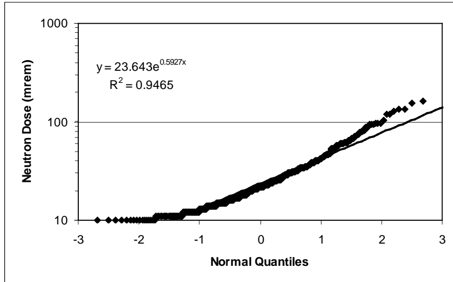
Figure 6-28. Normal probability plot for Group 9 neutron doses.
