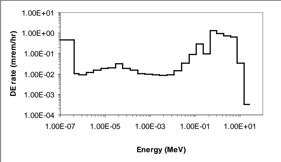
Figure 6-14. Neutron energy spectrum for contamination on the walls of the REDC WTA transfer tunnel.
