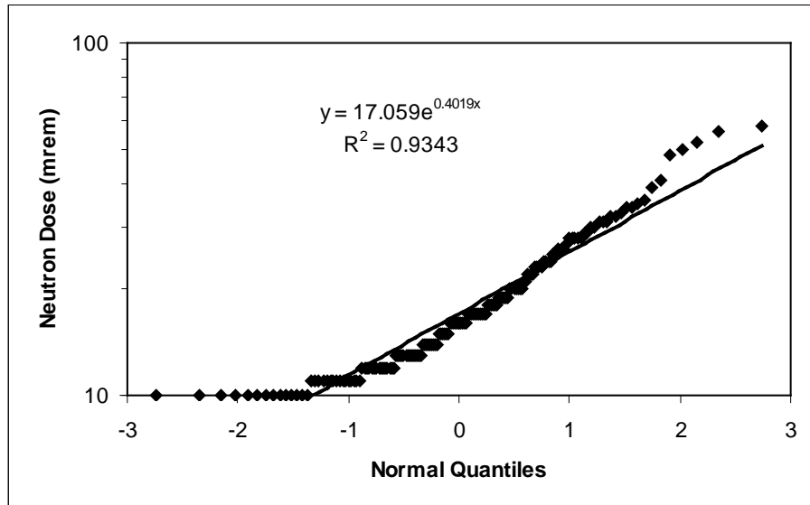
Figure 6-31. Normal probability plot for Group 21 neutron doses.
