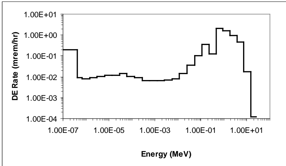
Figure 6-3. Neutron energy spectrum measured by PNL for drums of 241 Am-oxide in Building 3100.
