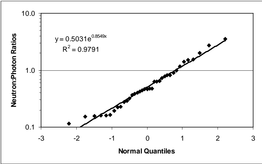
Figure 6-32. Normal probability plot for Group 13 neutron-to-photon dose ratios.
