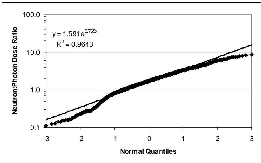
Figure 6-17. Normal probability plot for Group 2 neutron-to-photon dose ratios.
