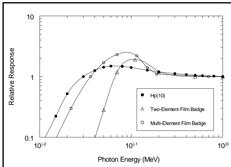
Figure 6-1. Comparison of Hp(10) for photons with the energy responses for a sensitive DuPont 502 emulsion in a two-element film badge (Pardue, Goldstein, and Wollan 1944) and a sensitive DuPont 555 emulsion in a multielement film badge (Thornton, Davis, and Gupton 1961).
