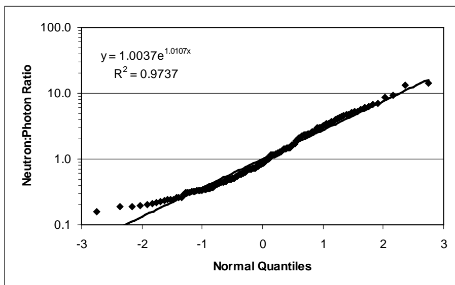
Figure 6-27. Normal probability plot for Group 9 neutron-to-photon dose ratios.
