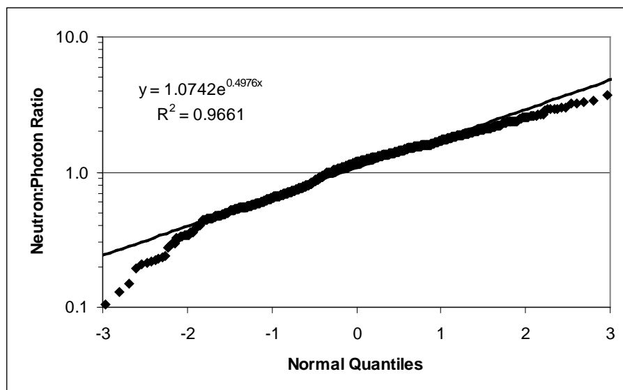
Figure 6-19. Normal probability plot for Group 4 neutron-to-photon dose ratios.
