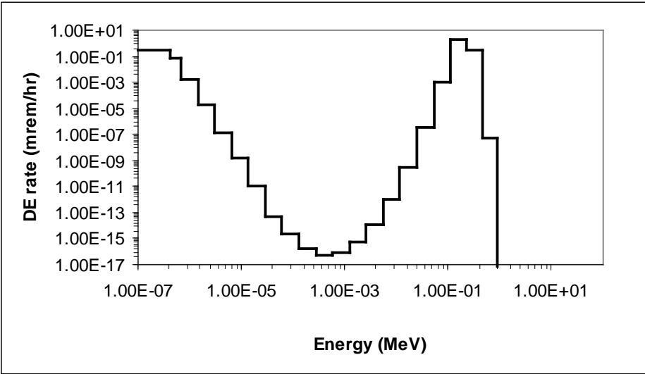
Figure 6-12. Neutron energy spectrum for the REDC TDF containing 12 mg 252 Cf.
