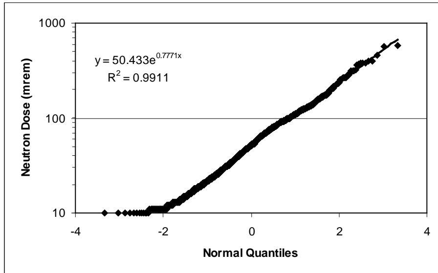
Figure 6-18. Normal probability plot for Group 2 neutron doses.
