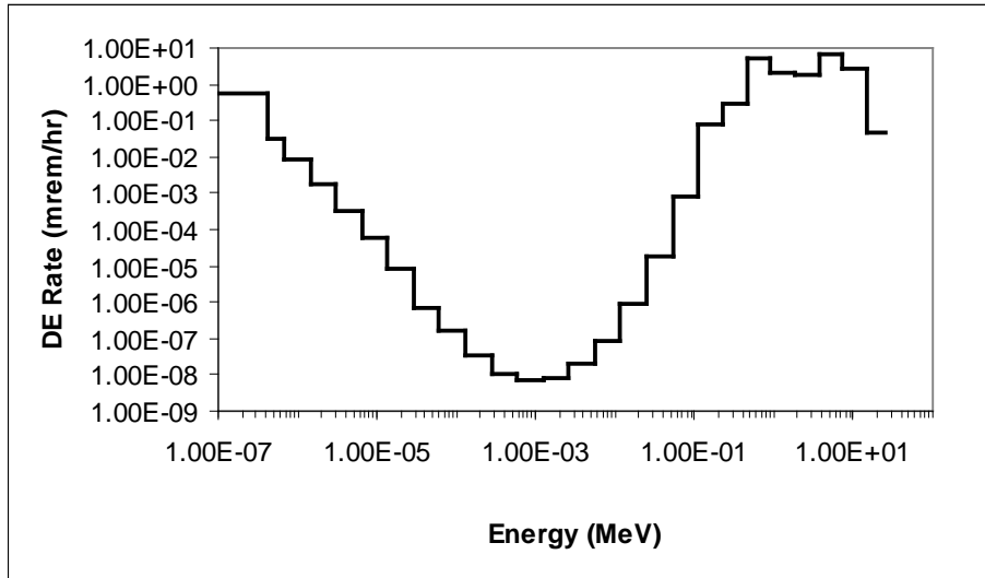
Figure 6-2. Neutron spectrum measured by PNL for ^{238}\text{Pu}:\text{Be} and ^{252}\text{Cf} sources in a water-shielded drum in Building 3038.
