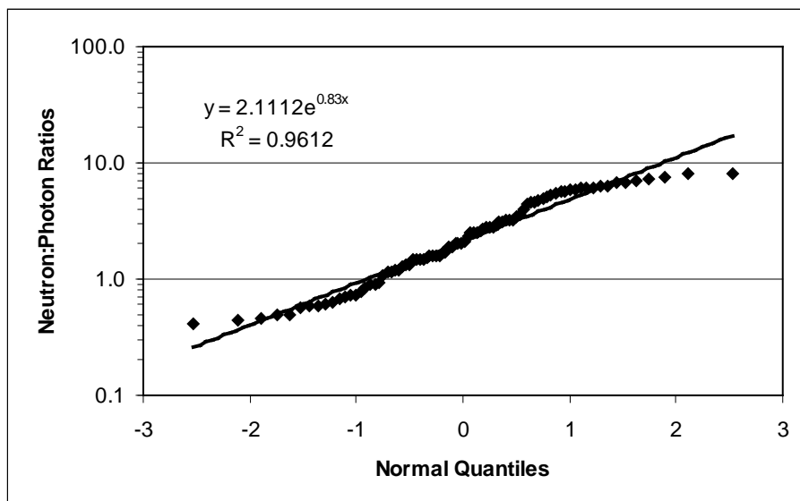
Figure 6-23. Normal probability plot for Group 17 neutron-to-photon dose ratios.
