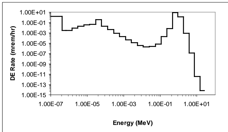
Figure 6-6. Neutron energy spectrum in the RADCAL beta/X-ray irradiation room with a moderated ^{252}\text{Cf} source exposed in the adjacent neutron irradiation room.
