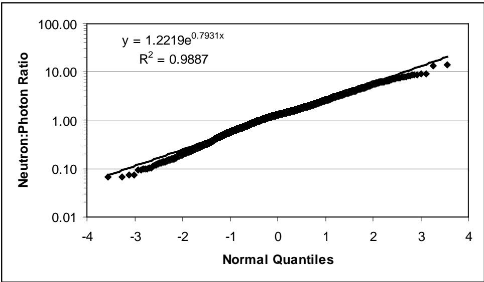
Figure 6-36. Normal probability plot for neutron-to-photon dose ratios derived from ORNL personnel neutron monitoring records for 1990 – 2004.
