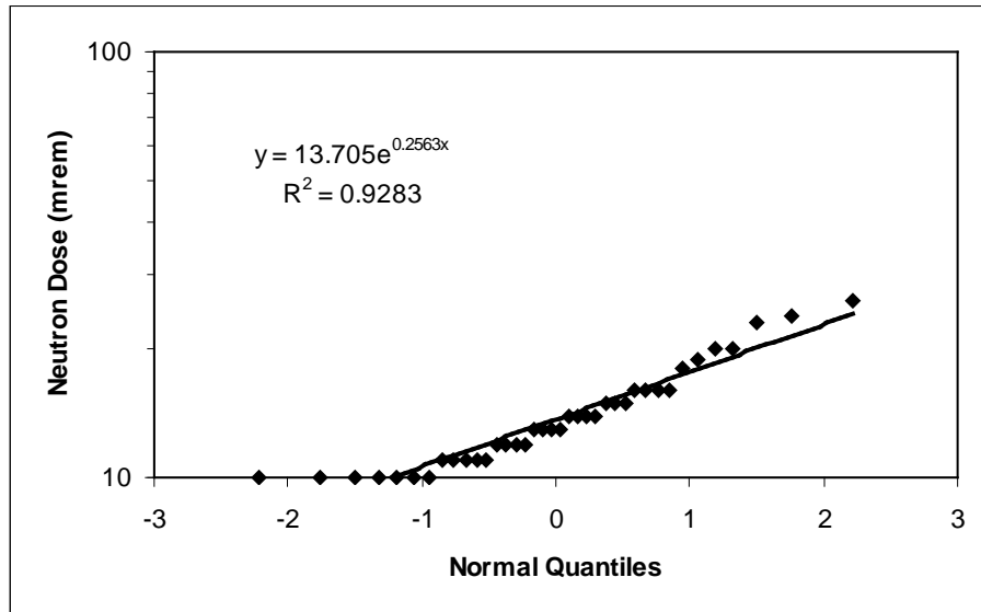
Figure 6-29. Normal probability plot for Group 11 neutron doses.
