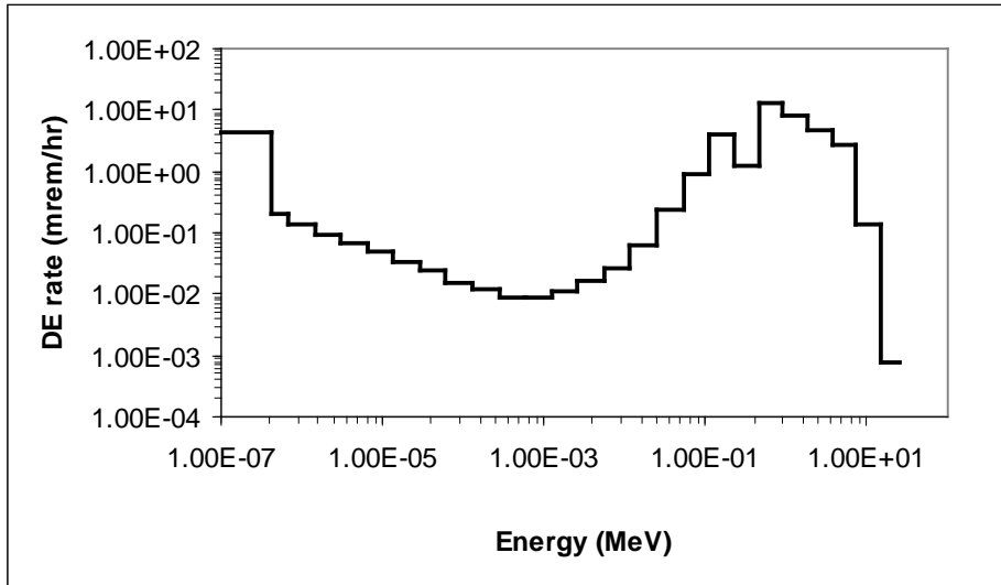
Figure 6-15. Neutron energy spectrum for waste casks in the SWSA 5 TRU storage bunker.
