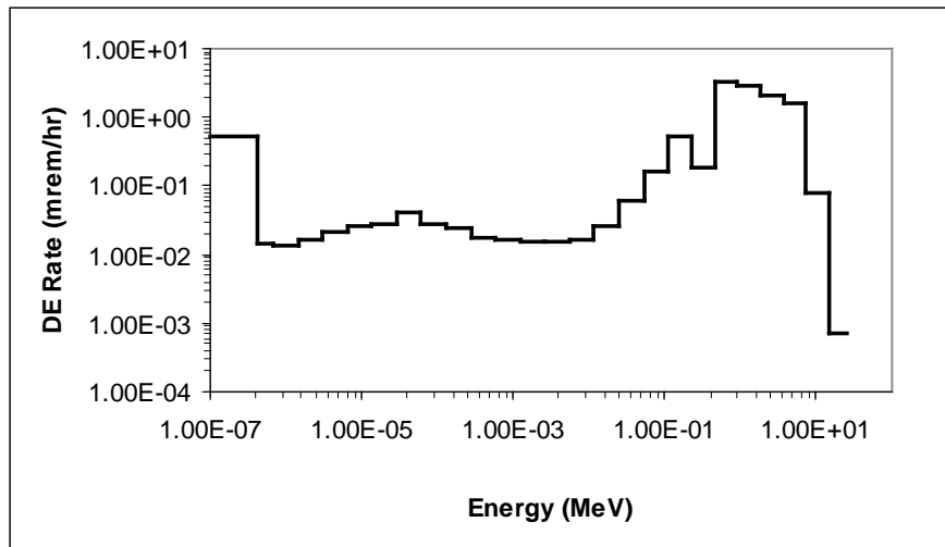
Figure 6-5. Neutron energy spectrum in the RADCAL beta/X-ray irradiation room with a bare ^{252}\text{Cf} source exposed in the adjacent neutron irradiation room.
