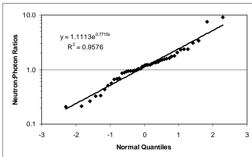
Figure 6-34. Normal probability plot for Group 14 neutron-to-photon dose ratios.
