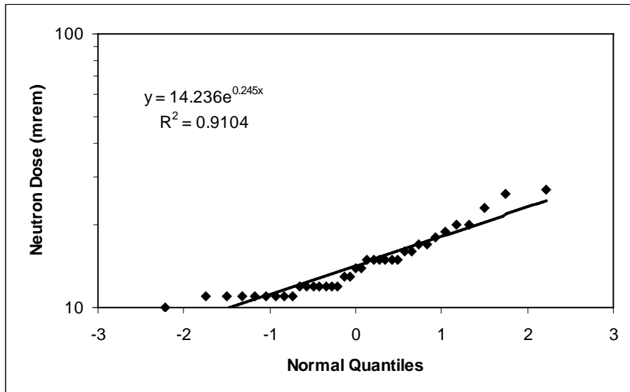
Figure 6-26. Normal probability plot for Group 7 neutron doses.
