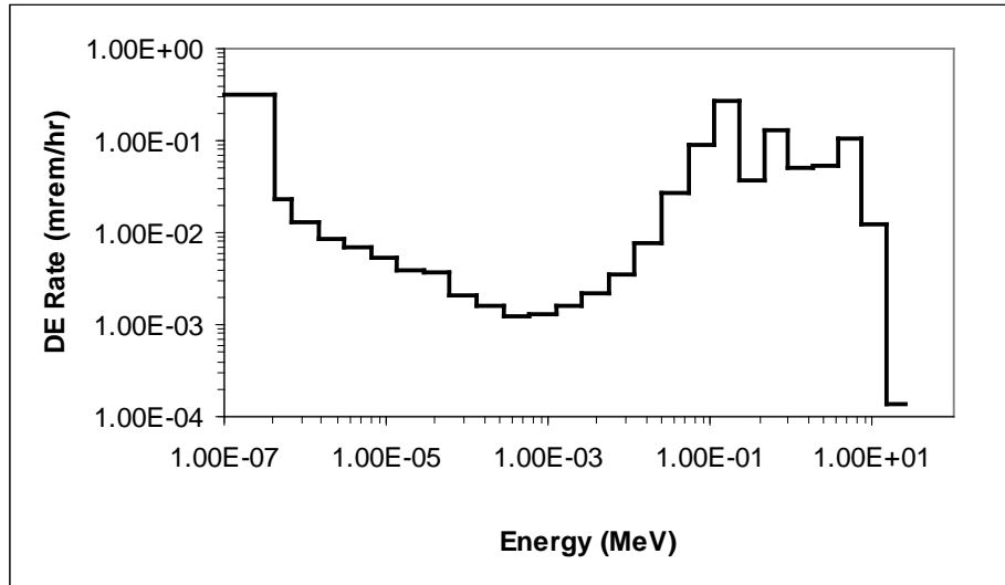
Figure 6-7. Neutron energy spectrum in the hallway outside the RADCAL neutron irradiation room with a moderated ^{252}\text{Cf} source exposed.
