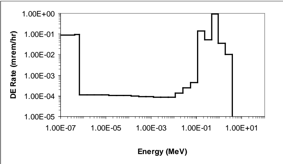
Figure 6-4. Neutron energy spectrum at the west entrance to the ORELA room.
