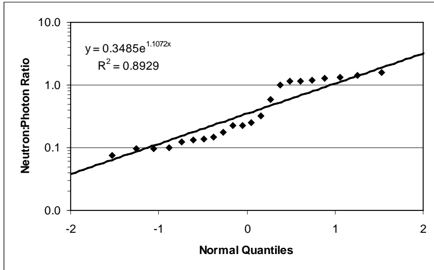
Figure 6-25. Normal probability plot for Group 7 neutron-to-photon dose ratios.
