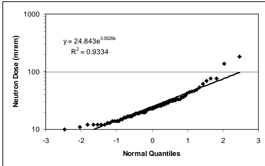
Figure 6-35. Normal probability plot for Group 14 neutron doses.
