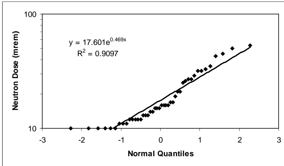
Figure 6-33. Normal probability plot for Group 13 neutron doses.
