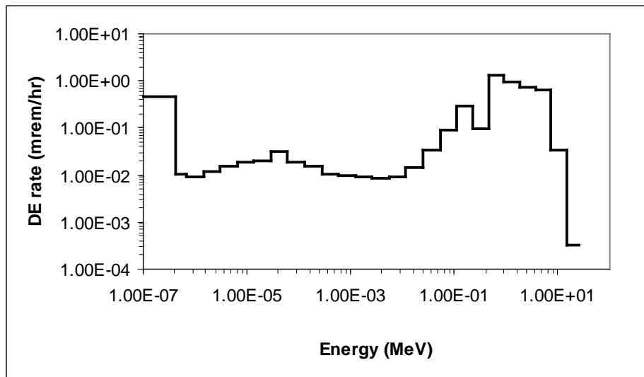
Figure 6-13. Neutron energy spectrum for a waste cask in the REDC Limited Access Area.
