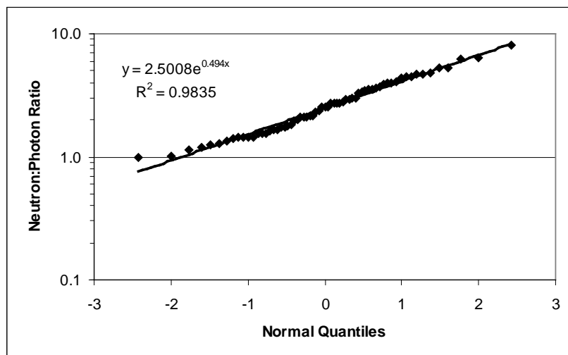
Figure 6-21. Normal probability plot for Group 3 neutron-to-photon dose ratios.
