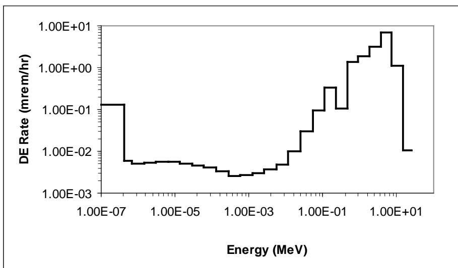
Figure 6-9. Neutron energy spectrum in RASCAL Room 102 at 130 cm from the ^{238}\text{Pu}:\text{Be} neutron calibration source.
