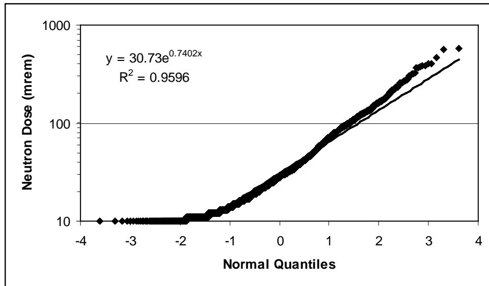
Figure 6-37. Normal probability plot for neutron doses \geq 10 mrem for ORNL workers in the period from 1990 – 2004.
