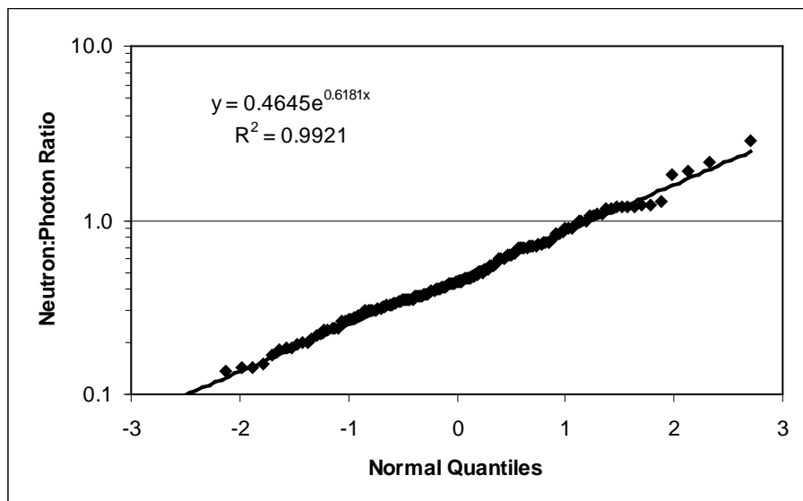
Figure 6-30. Normal probability plot for Group 21 neutron-to-photon dose ratios.
