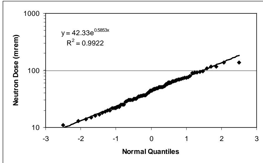
Figure 6-24. Normal probability plot for Group 17 neutron doses.
