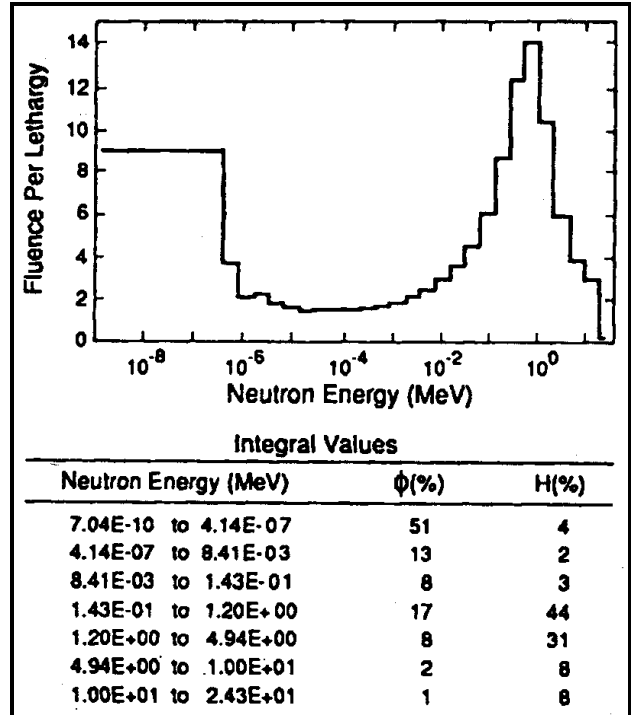
4 Figure 6-6. Neutron spectrum of ^{238}\text{Pu} Ball 5 Milling Process at LANL Plutonium Facility 6 (Harvey and Hajnal 1993).
