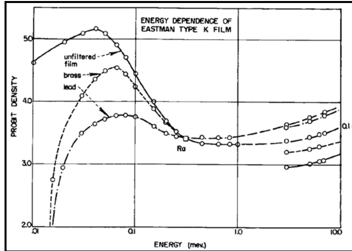
Figure 6-4. Energy dependence of Eastman Kodak Type K Film for exposure of 0.10 R (Storm 1951)
