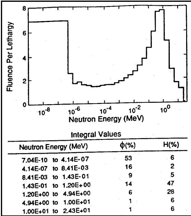
1 Figure 6-5. Neutron spectrum of 2 hydrofluorination of ^{239}\text{PuO}_2 at LANL Plutonium 3 Facility (Harvey and Hajnal 1993).
