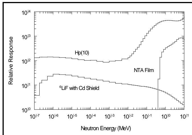
Figure 6-2. Comparison of Hp(10) for neutrons with energy responses of NTA film and neutron albedo dosimeter containing a TLND chip made of ^6\text{LiF} and shielded by cadmium (IAEA 1990).
