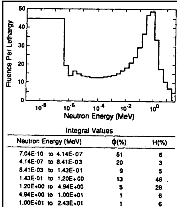
Figure 6-7. Neutron spectrum near door K in SNM Vault at LANL Plutonium Facility (Harvey and Hajnal 1993).
