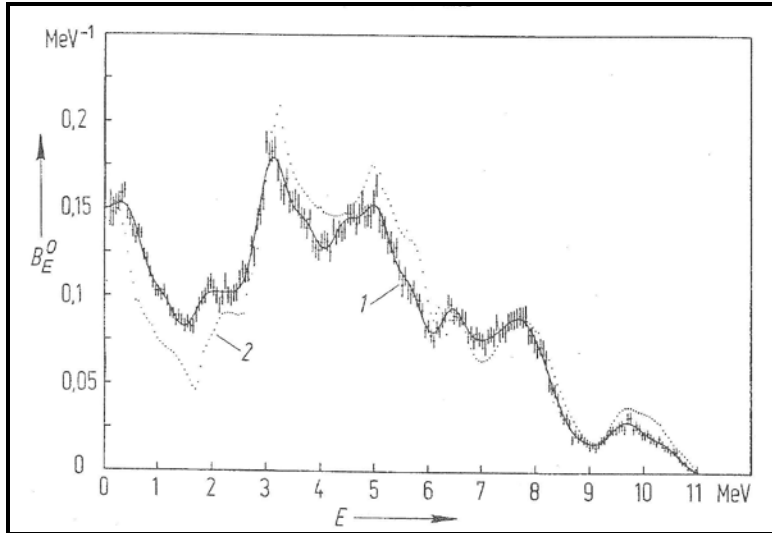
Figure 6-8. Probability density of neutron spectrum from an ^{241}\text{AmBe} ( \alpha, n ) source (Kluge and Weiss 1982).
