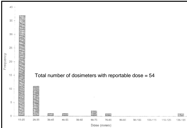
Figure 6-11. Distribution of reportable neutron dose at the INEEL for the first 9 months of 1995. Of 1461 dosimeters, 1407 were below the 15 mrem reporting level.
