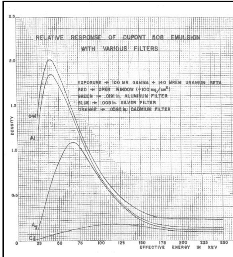
Figure 6-7. Response of Dupont 508 film with various filters to 140 mrem uranium beta and 100 mR of different energy photon irradiation provided by NBS. The original badge used the open window and cadmium shielded films. The multiple filter badge used all three filters plus the open window (Cipperley and Gammill 1959).
