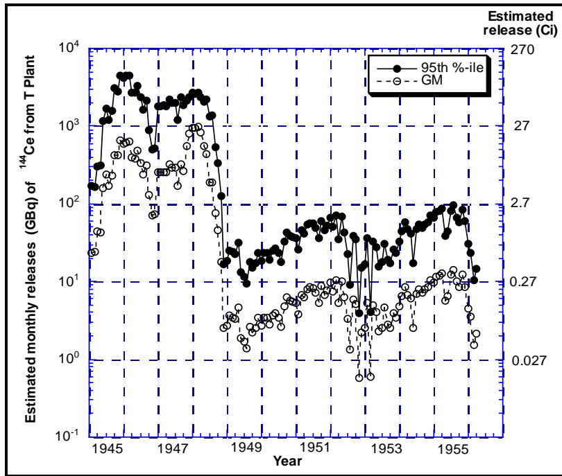
Figure 4-4. Estimated releases of ^{144}\text{Ce} from T Plant (Till et al. 2002).
