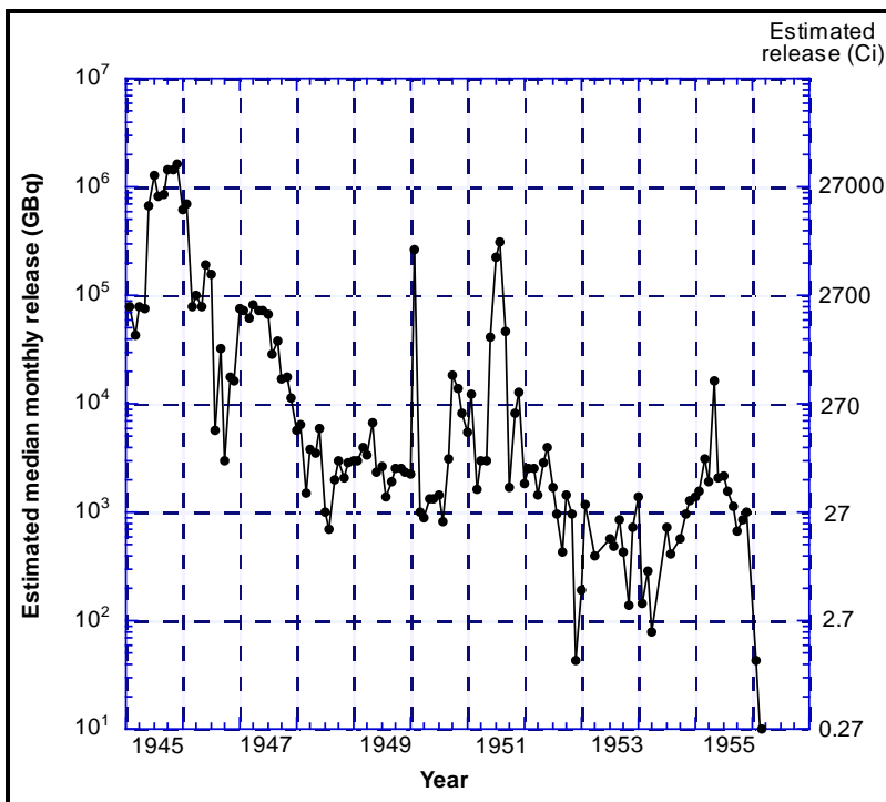
Figure 4-5. Estimated releases of ^{131}\text{I} from T Plant. Heeb (1994) and Napier (2002) provided estimates (Till et al. 2002).
