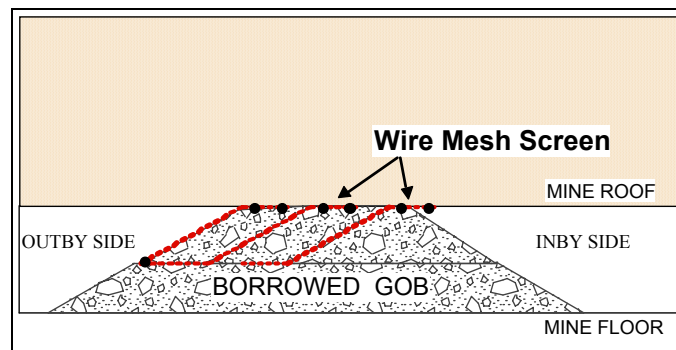
Figure 2. The "fully-stowed" alternate Attenuator design with sections of corrosion resistant wire roof mesh to provide confinement and passive reinforcement to minimize material erosion during the pressure blow down. This design was tested and evaluated in full-scale explosion tests at the NIOSH Lake Lynn Experimental Mine, but without the wire mesh screen.
