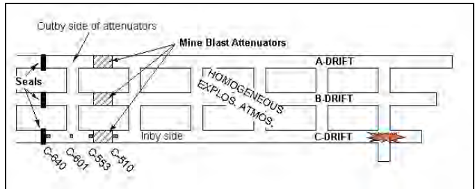
Figure 4. Lake Lynn Experimental Mine layout of a Passive Mine Blast Attenuator used in SHAMRC numerical detonation simulations.
