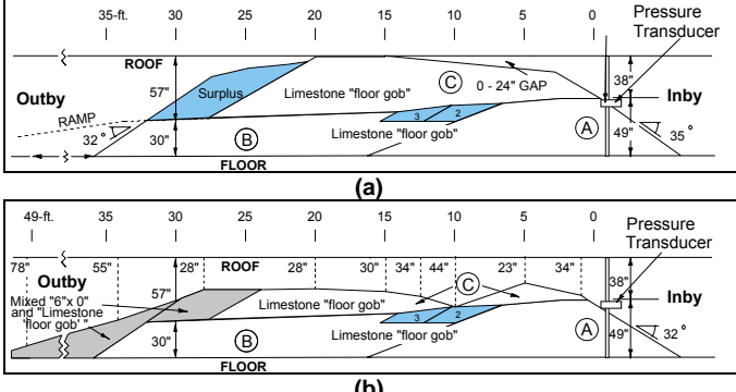
Figure 13. Configuration of Mine Blast Attenuator before (a) and after (b) the third test (LLEM Test #527).
