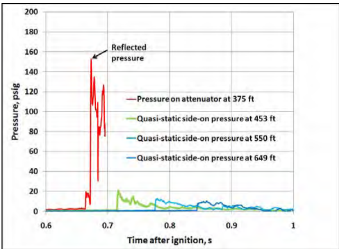
Figure 12. Reflected explosion pressure inby the Attenuator and the quasi-static pressure 78, 175, 274 and 432 ft outby the Attenuator during the second test (LLEM Test #526).
