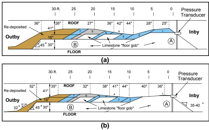
Figure 10. Configuration of Mine Blast Attenuator before (a) and after (b) the second test (LLEM Test #526).
