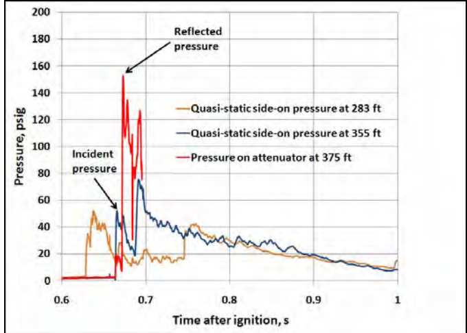
Figure 11. Incident quasi-static pressures inby the Attenuator (A-283, A-355) and reflected explosion pressure at the Attenuator (A-375) during the second test (LLEM Test #526).
