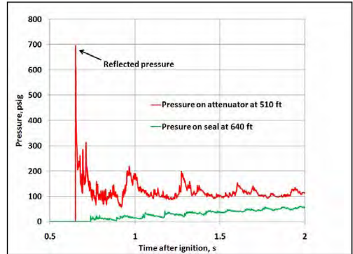
Figure 5. SHAMRC-calculated pressures just inby the simulated Attenuator (C-510) and just inby the simulated seal (C-640) located in C-drift of the Lake Lynn Experimental Mine (see Figure 4).
