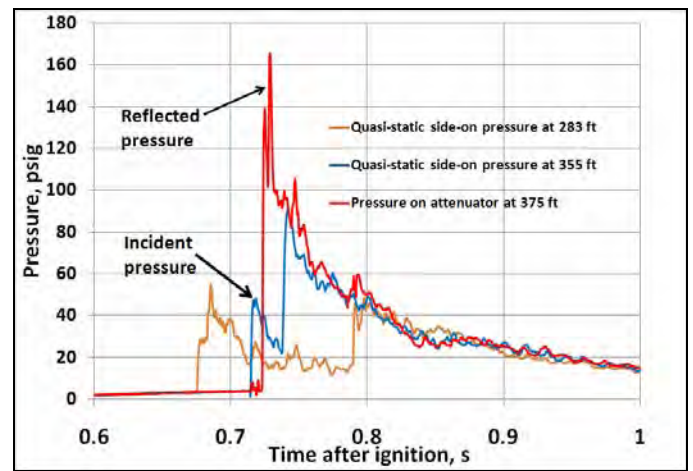
Figure 8. Quasi-static side-on pressures inby the Attenuator (A-283, A-355) and reflected explosion pressure at the Attenuator (A-375) during the first test (LLEM Test #525) (see Figure 6).
