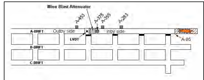
Figure 6. Lake Lynn Experimental Mine layout of the Mine Blast Attenuator tested against rather small methane-air deflagrations in A-drift.
