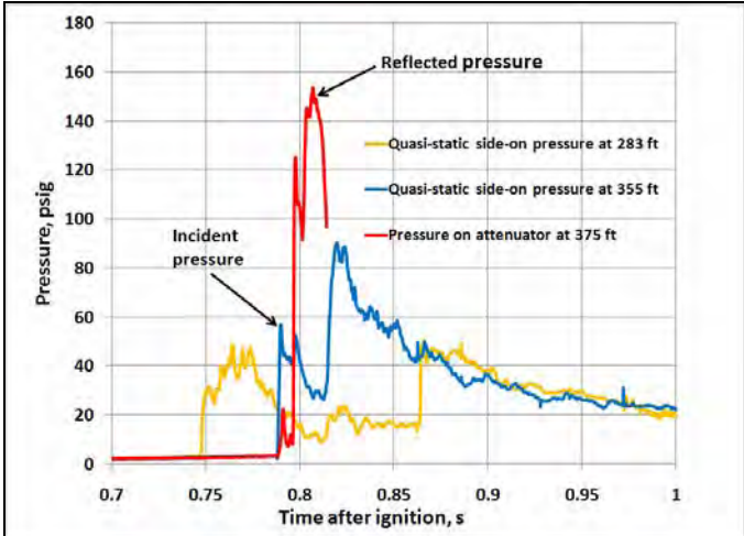
Figure 14. Incident quasi-static pressures inby the Attenuator (A-283, A-355) and reflected explosion pressure at the Attenuator (A-375) during the third test (LLEM Test #527).
