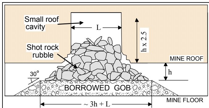
Figure 1. The "shot-rock" optimum Attenuator design where a section of the mine roof is shot down with explosives using holes drilled prior to placement of an optional foundation layer of borrowed gob material.
