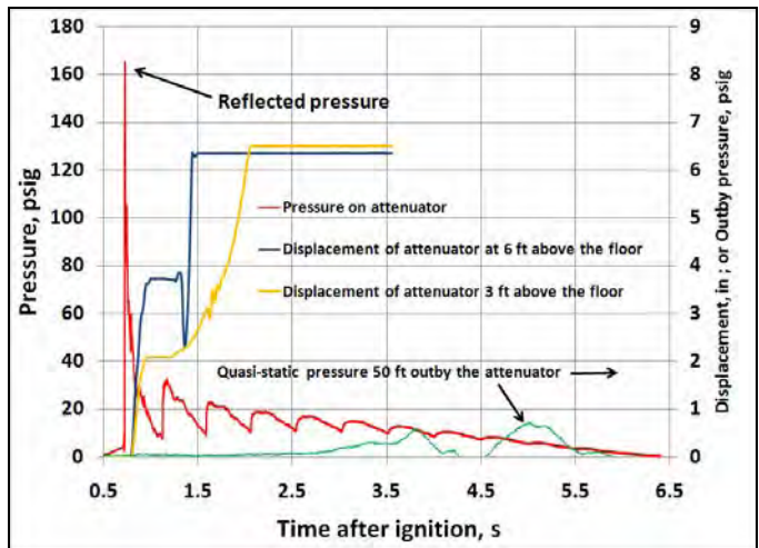
Figure 9. Reflected explosion pressure inby the Attenuator (A-375) and the quasi-static pressure 15 m (50 ft) outby the Attenuator (A-453) during the first test (LLEM Test #525). Displacement of the Attenuator as measured with LVDTs is also shown.
