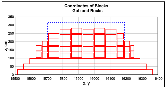
Figure 3. The Attenuator configuration used in the SHAMRC calculations. The lower one meter is assumed to be well packed gob material and the upper composed of large rocks with 20% void spaces.
