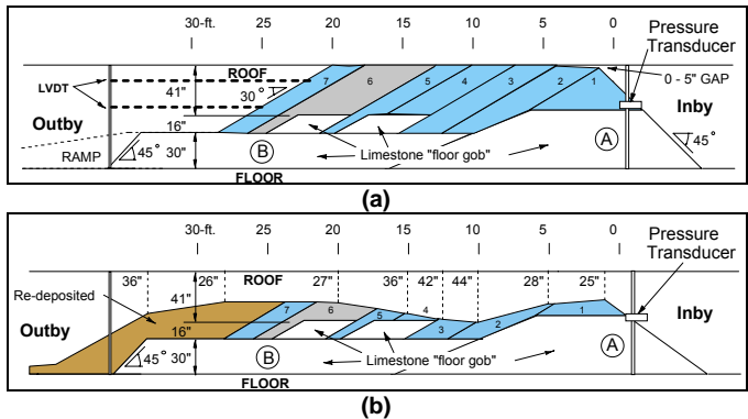
Figure 7. Configuration of Mine Blast Attenuator before (a) and after (b) the first test (LLEM Test #525). White: 46-cm (18-in.) x 0 limestone rubble, Blue: 15-cm (6-in.) x 0 crusher-run limestone, Gray: Mixed 15-cm (6-in) x 0 and Limestone, Brown: Re-deposited material (undifferentiated).
