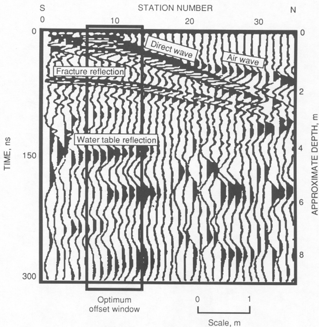
Figure 8.—WARR sounding conducted at abandoned Duluth gabbro quarry site in northeastern Minnesota.
