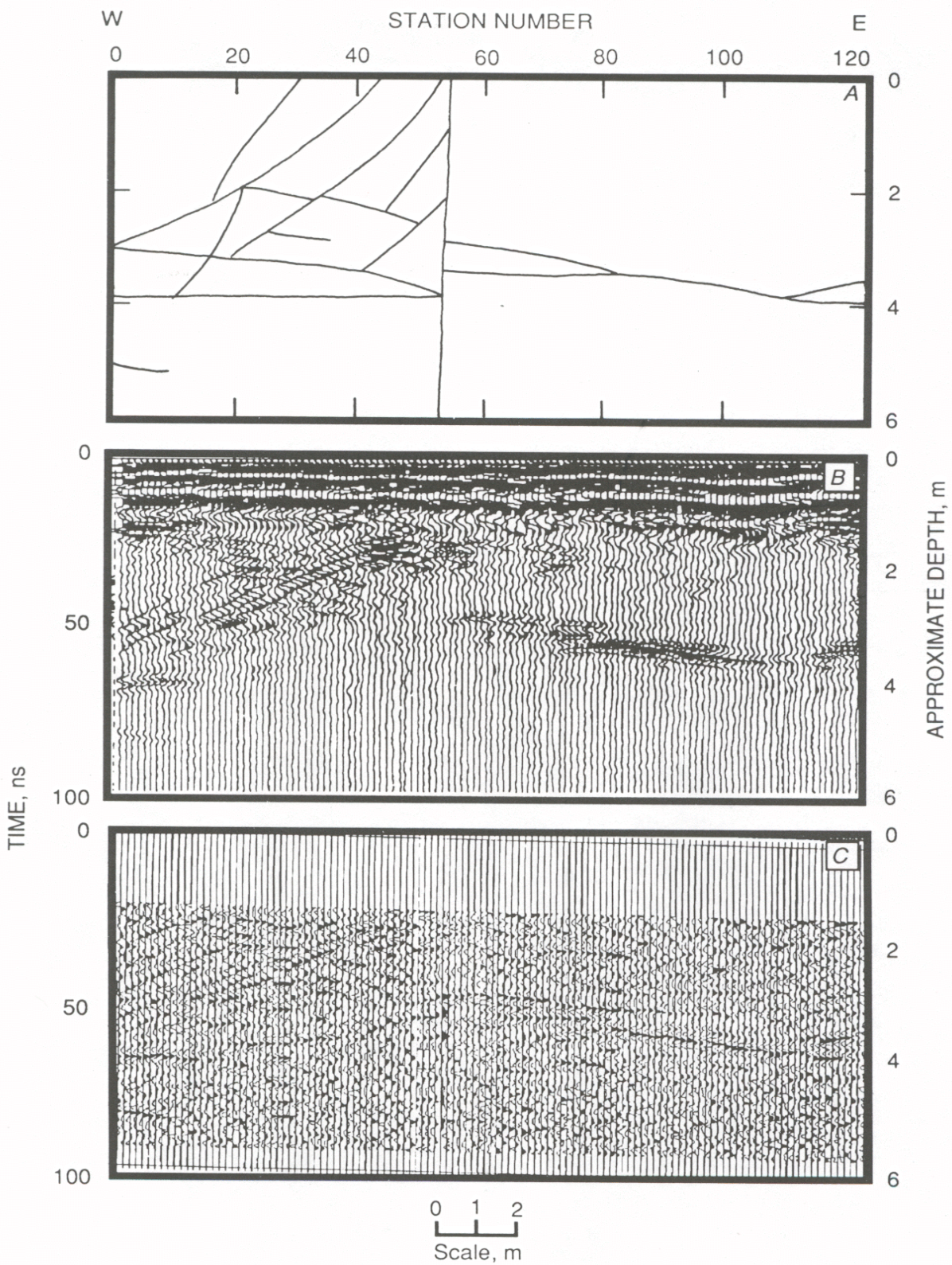
Figure 4.—Vertical analysis of fractures exposed along north face of Charcoal granite quarry No. 3. A, Mapped highwall fracture distribution; B, unprocessed vertical common offset radar profile; C, processed vertical common offset radar profile.
