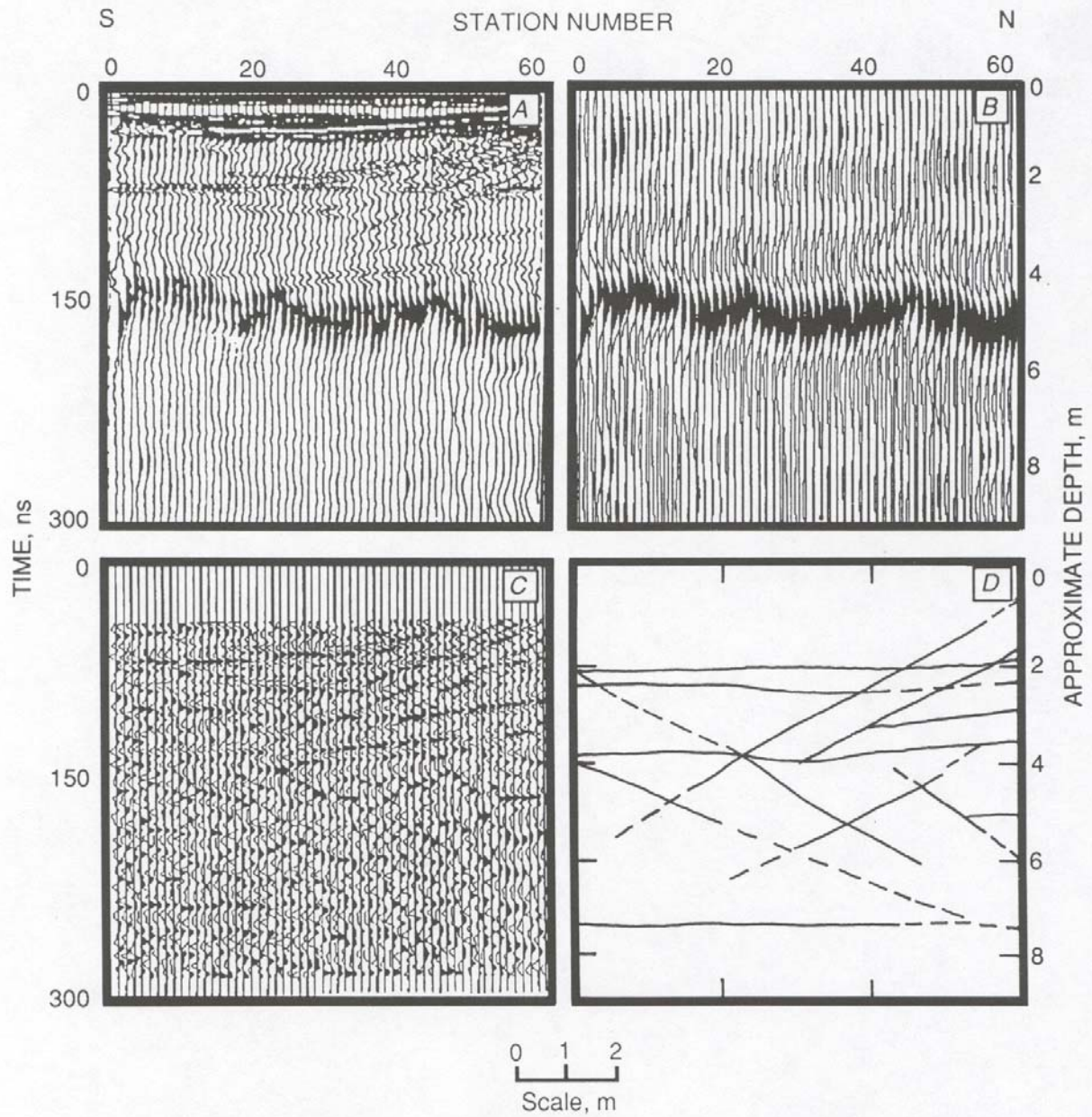
Figure 10.—Analysis of fractures at abandoned Duluth gabbro quarry in northeastern Minnesota. A, Unprocessed vertical common offset radar profile; B, processed (25-MHz low-pass filter) vertical common offset gabbro profile showing the water table reflection; C, processed (150-MHz high-pass filter) vertical common offset gabbro profile showing fracture reflections; D, mapped highwall fracture distribution.
