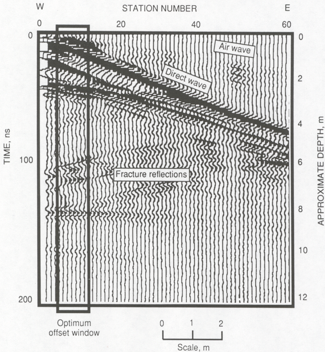
Figure 2.—WARR sounding conducted at north face of Charcoal granite quarry No. 3.
