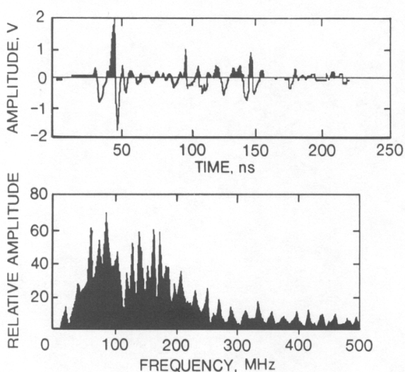
Figure 3.—Spectral analysis of WARR sounding conducted at north face of Charcoal granite quarry No. 3.
