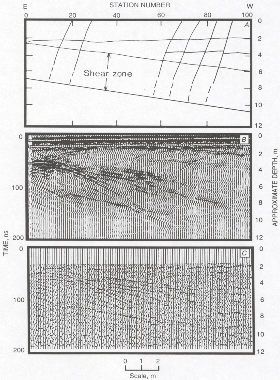
Figure 5.—Horizontal or plan view analysis of fractures from north face of Charcoal granite quarry No. 3 inward. A, Mapped and inferred vertical fractures; B, unprocessed horizontal common offset radar profile; C, processed horizontal common offset radar profile.
