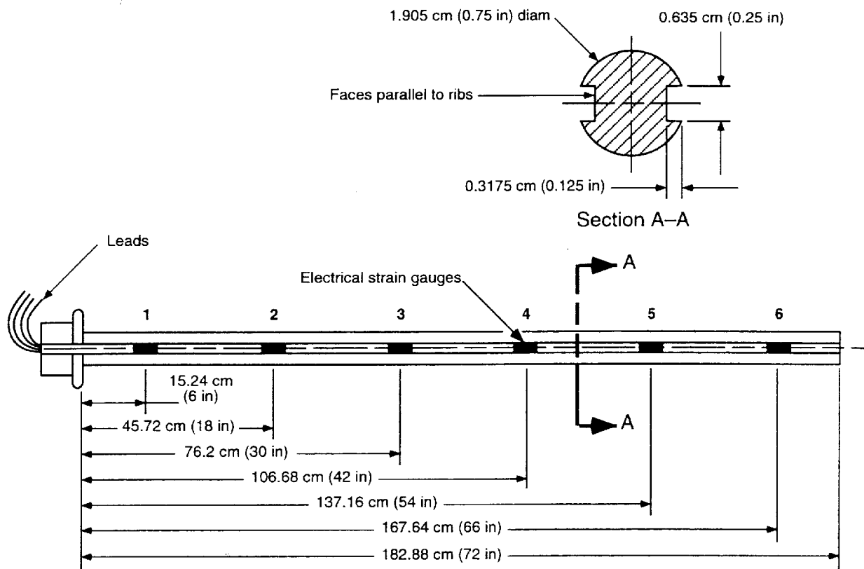
Figure 1.—Instrumented roof bolt
