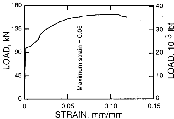
Figure 2.—Stress-strain curve of slotted roof bolt
