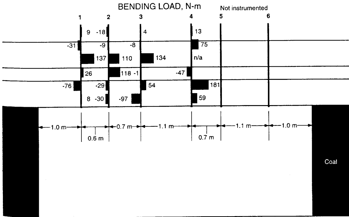
Figure 4.—Load profiles for test site 2
