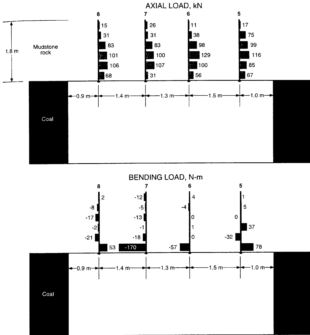
Figure 3.—Load profiles for test site 1
