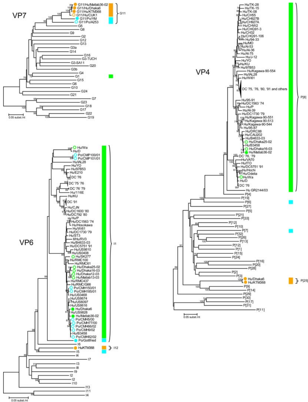
Figure 1. Phylogenetic trees based on full-length nucleotide sequences of rotavirus structural protein (VP4, VP6, and VP7) genes. Bootstrap values (500 replicates) >70 are shown. Only genotypes in which
