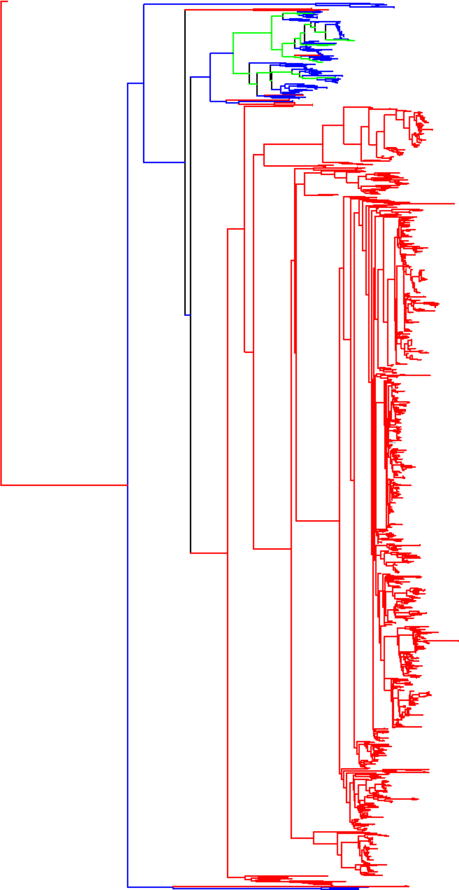
Technical Appendix Figure 4. Complete phylogenetic tree of all N1 nucleotide sequences. The tree was built by the neighbor-joining algorithm. Green branches show isolates whose H6 gene invaded North America from Eurasia, red branches show isolates from Eurasia, and blue branches show isolates from North America. Virus names are not shown because of the large tree size.
