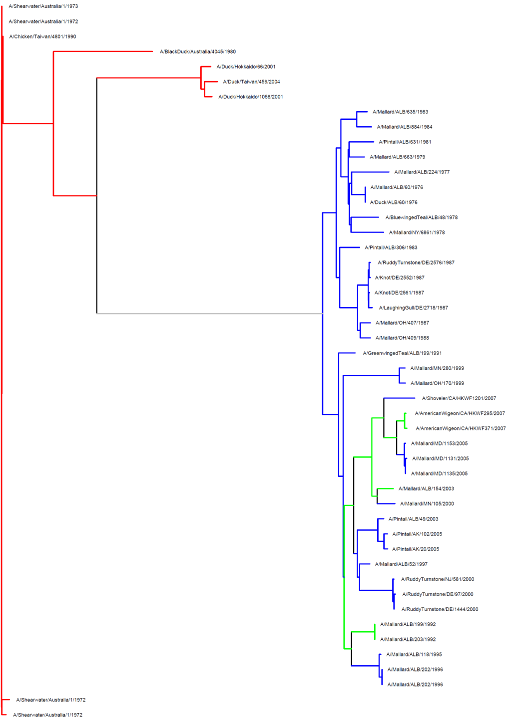
Technical Appendix Figure 6. Complete phylogenetic tree of all N5 nucleotide sequences. The tree was built by the neighbor-joining algorithm. Green branches show isolates whose H6 gene invaded North America from Eurasia, red branches show isolates from Eurasia, and blue branches show isolates from North America.
