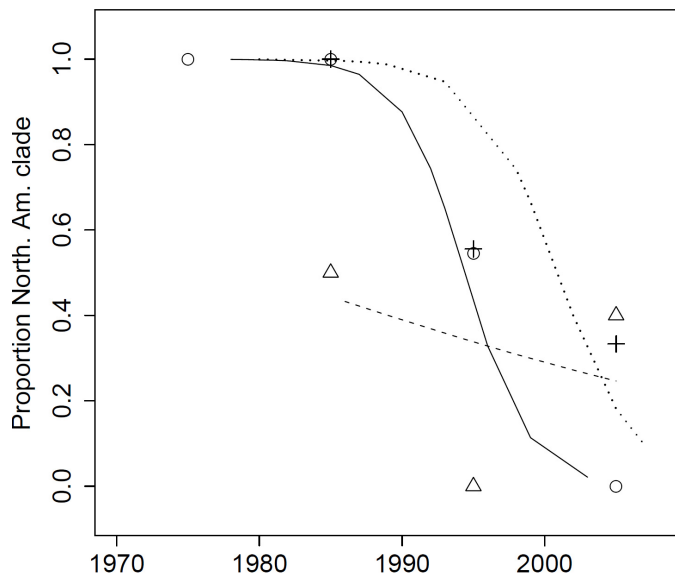
Technical Appendix Figure 2. Proportion of viruses from the North American clade among wild bird isolates in 3 regions of North America grouped by decade. Lines show fitted logistic regressions.
