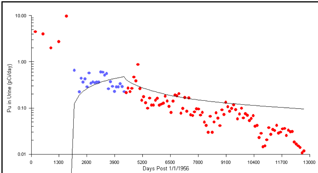
Figure B-12. Predicted (line) and observed (dots) 84th-percentile urinary excretion assuming inhalation intakes of type M plutonium, 1961 to 1967.
