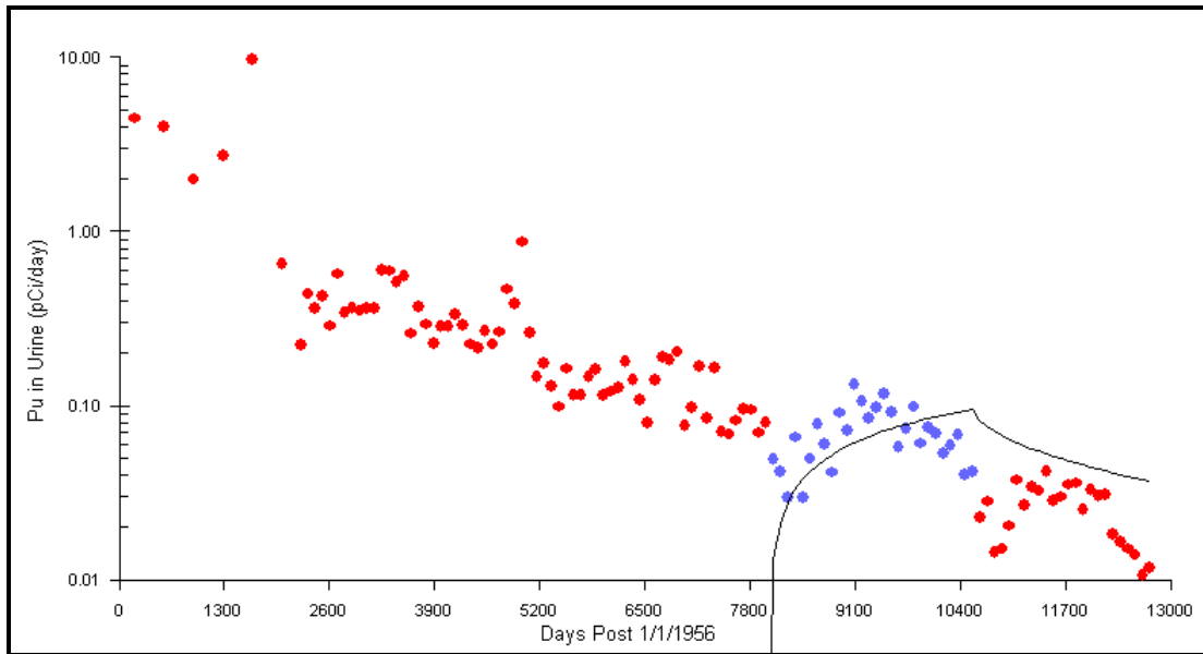
Figure B-15. Predicted (line) and observed (dots) 84th-percentile urinary excretion assuming inhalation intakes of type M plutonium, 1978 to 1984.
