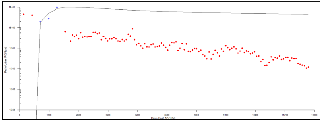
Figure B-25. Predicted (line) and observed (dots) 84th-percentile urinary excretion assuming a single chronic inhalation intake of type S plutonium, 1958 to 1960.
