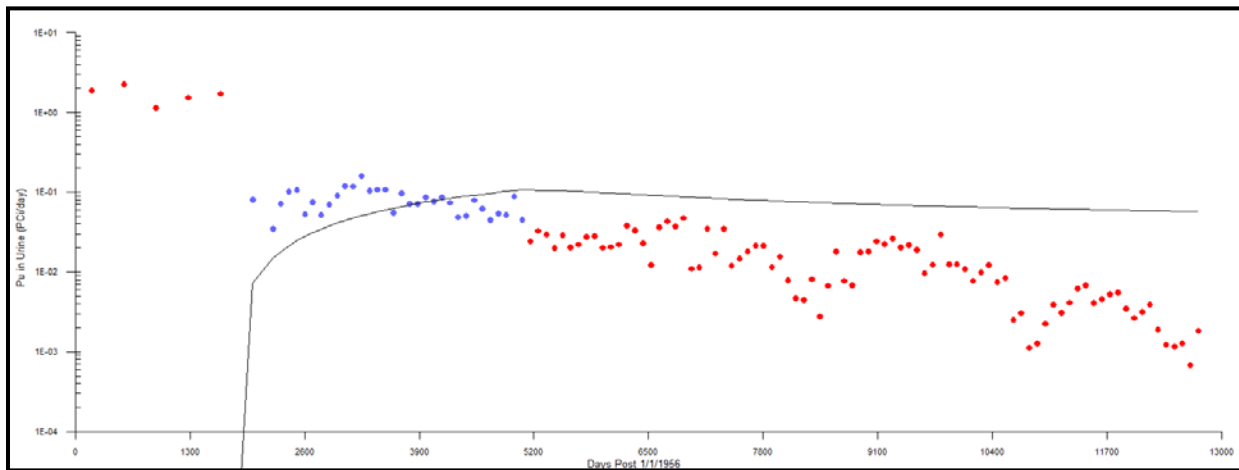
Figure B-20. Predicted (line) and observed (dots) 50th-percentile urinary excretion assuming a single chronic inhalation intake of type S plutonium, 1961 to 1969.
