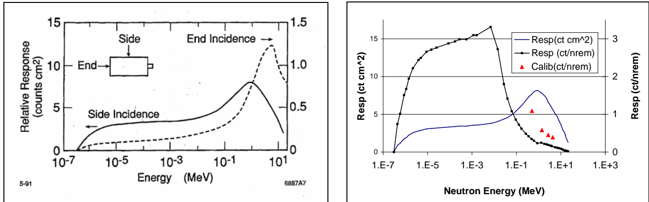
Figure A-2. Fluence and dose response vs. energy for PMS neutron detector (Liu et al. 1991) [11]
