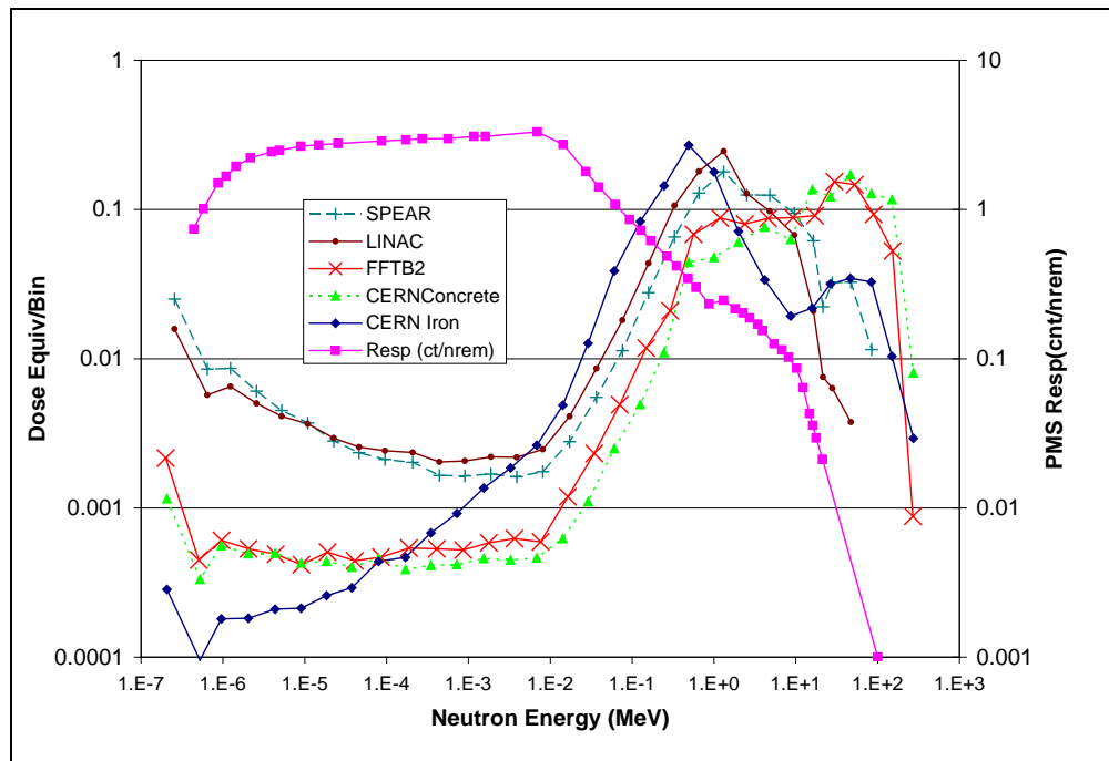
Figure A-3. Log plot of dose equivalent/bin for high-energy neutron spectra and PMS instrument response [12].
