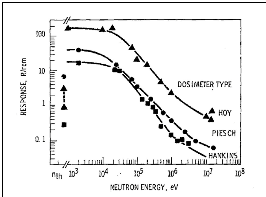
Figure A-5. Energy response of various albedo dosimeters (Piesch and Burghardt 1978).
