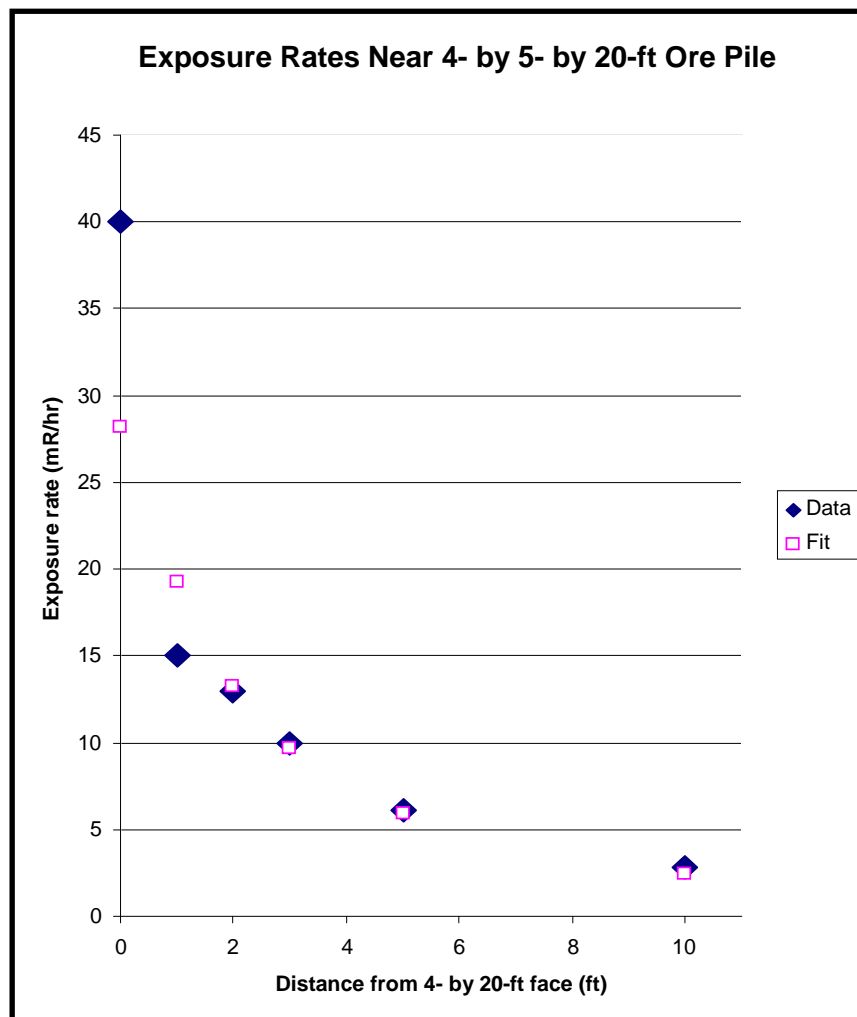
Figure 4-1. Fit to gamma exposure data for a 4- by 5- by 20-ft pile of 8% African pitchblende ore.
