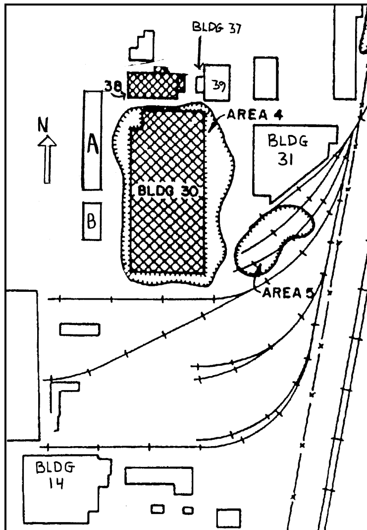
Figure 2-1. Linde Ceramics Plant and Tonawanda Laboratory buildings on LAPC Tonawanda site.
