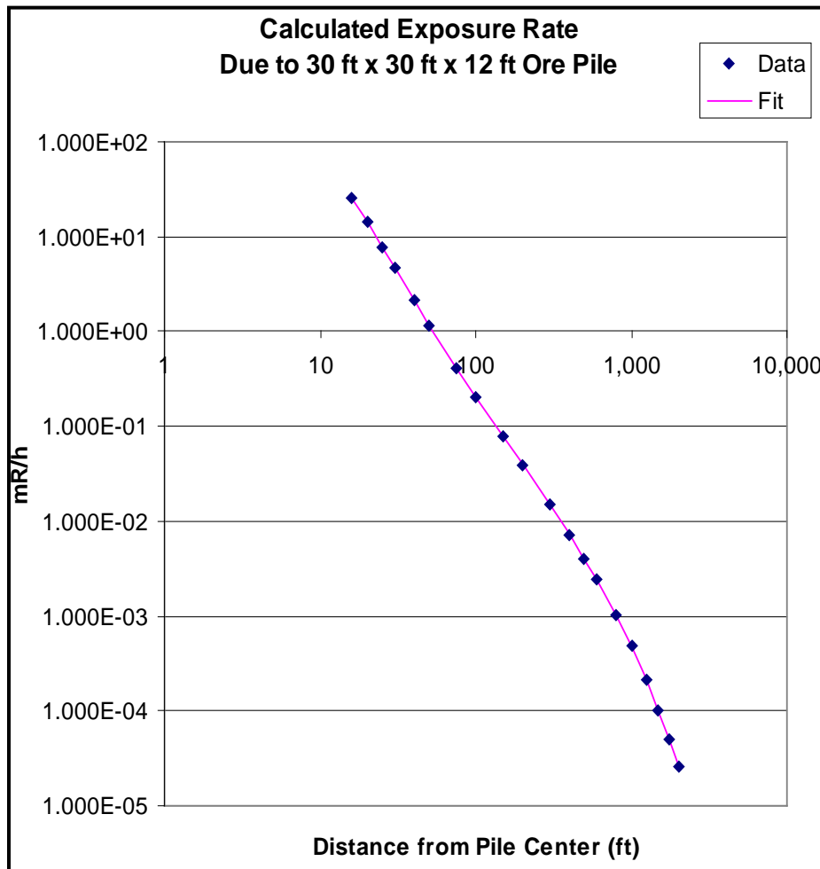
Figure 4-2. Calculated exposure rates and analytic fit for a 30- by 30- by 12-ft pile of 8% African pitchblende ore.
