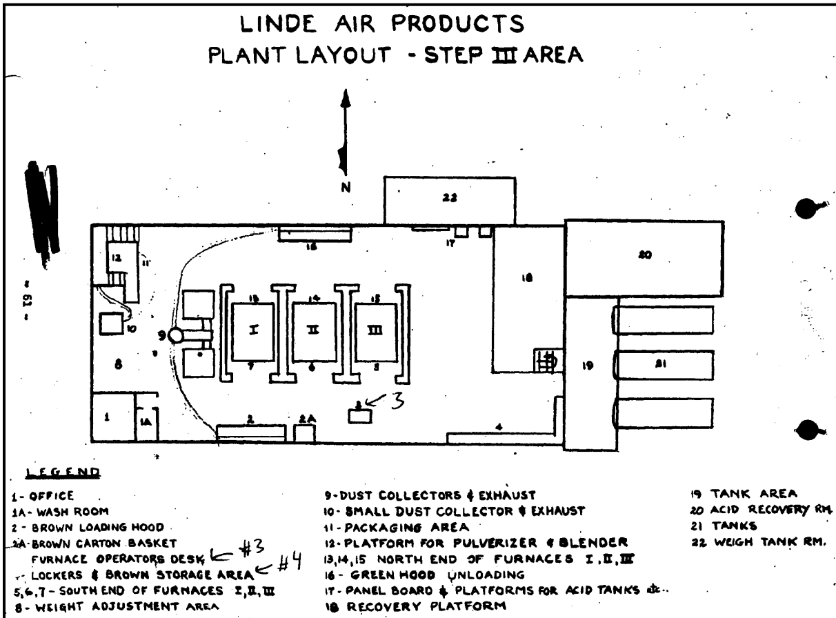
Figure 2-4. Building 38 layout (Klevin 1949a).
