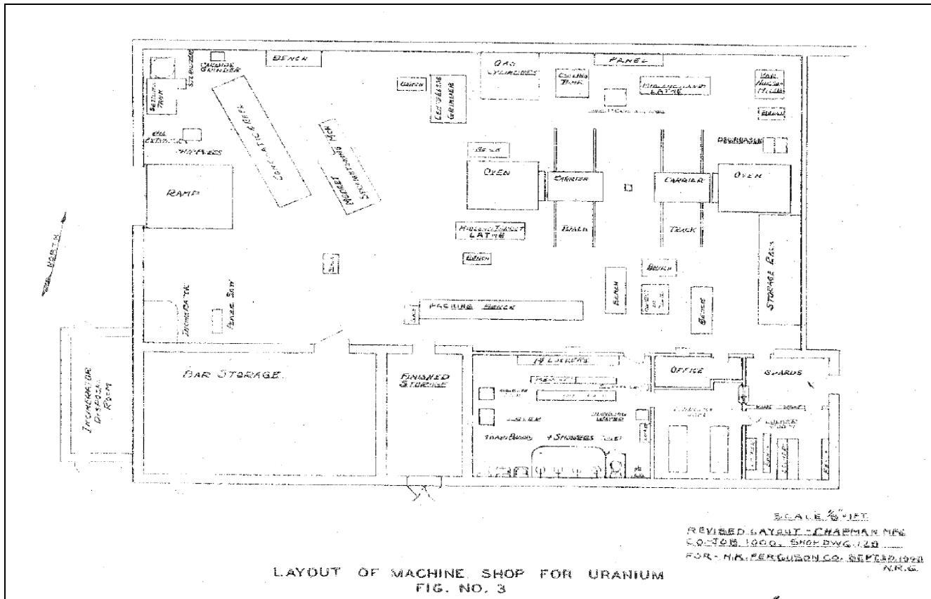
Figure 2-2. Layout of machine shop in Building 23 (Kemmer, 1949).
