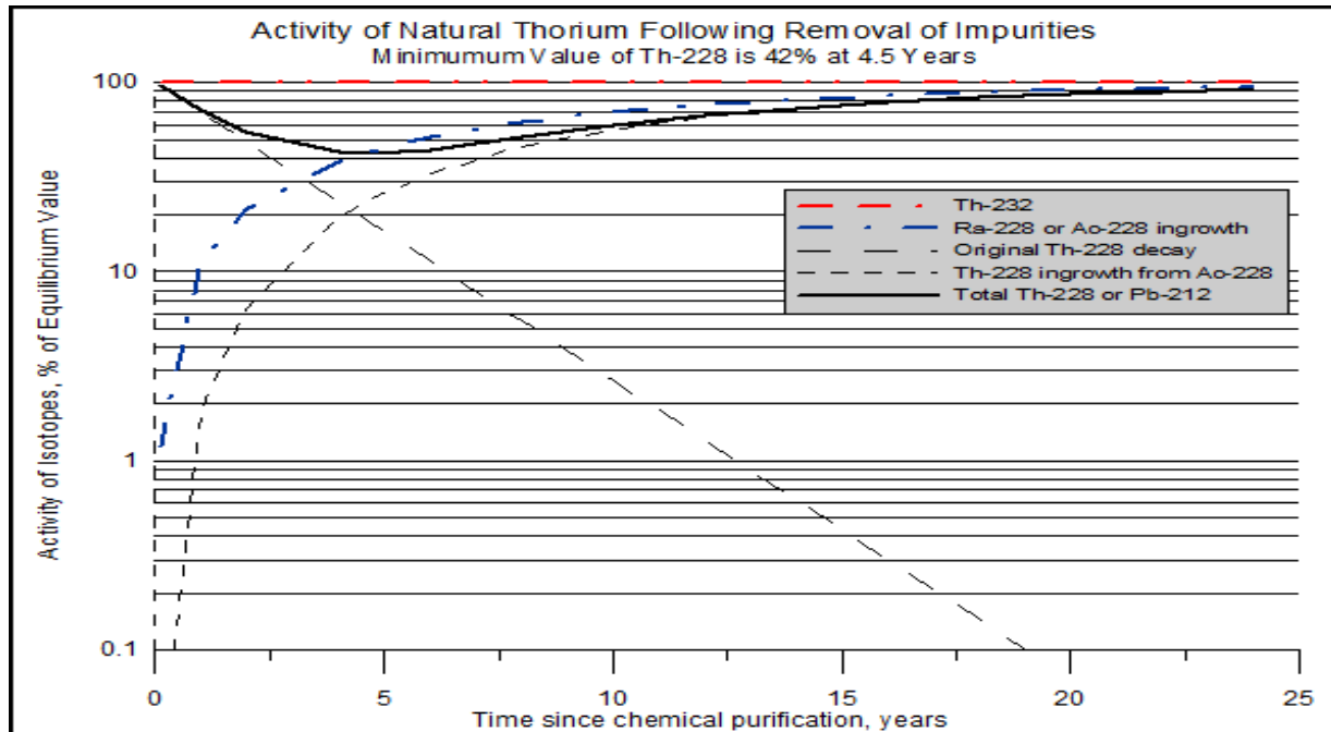
Figure 5-2: Decay and Buildup of Thorium-228 and Daughters Following Processing
