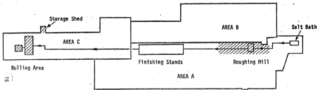
Figure 1. Superior Steel processing areas (ORNL 1981).
