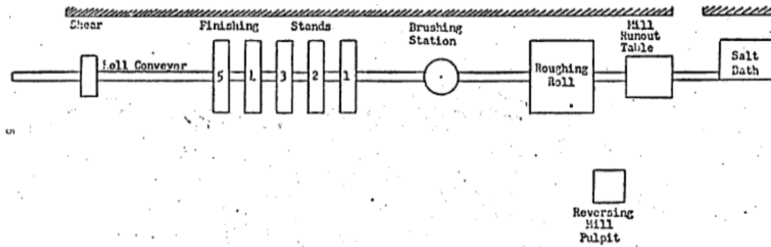
Figure 2. Superior Steel uranium mill layout (ORNL 1981).
