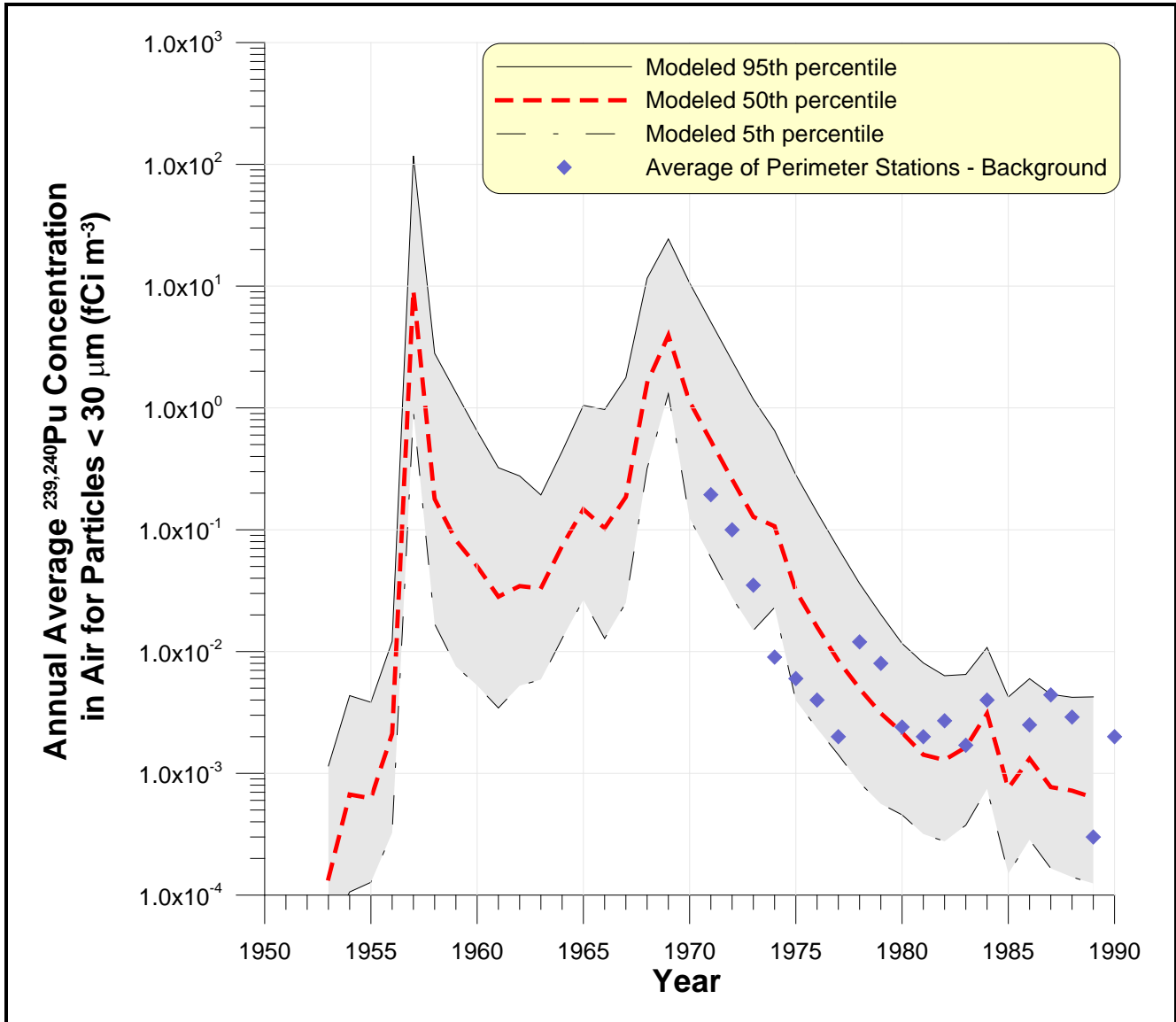
Figure 4A-4. Annual average ^{239,240}\text{Pu} concentrations in air as a function of time for particles < 30\ \mu\text{m} Aerodynamic Equivalent Diameter (AED) in the perimeter area surrounding RFP. (Model-predicted concentrations represent the average of 27 computational nodes as shown in Figure 4A-7 using the model described in Rood and Grogan (1999).)
